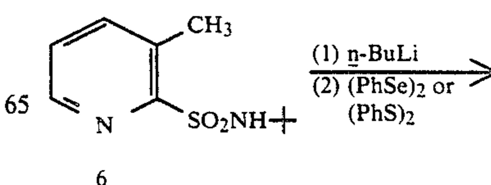
Equation 6
