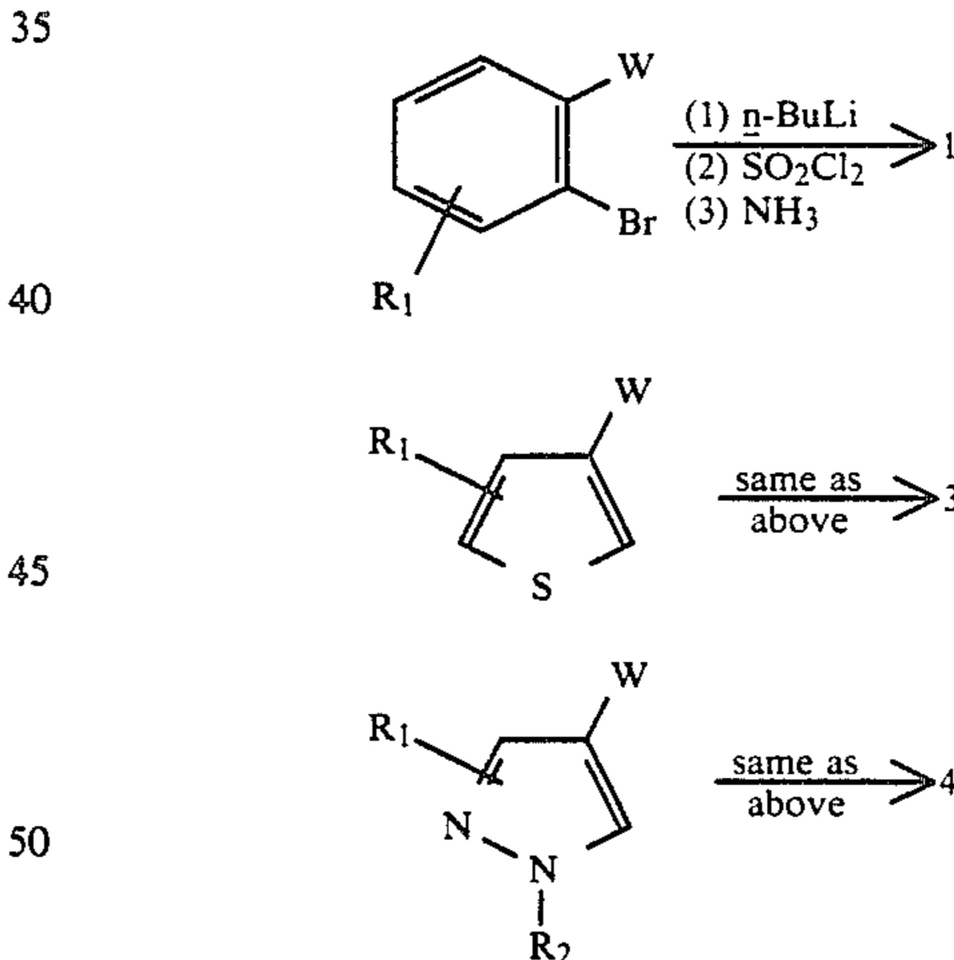
Equation 5
