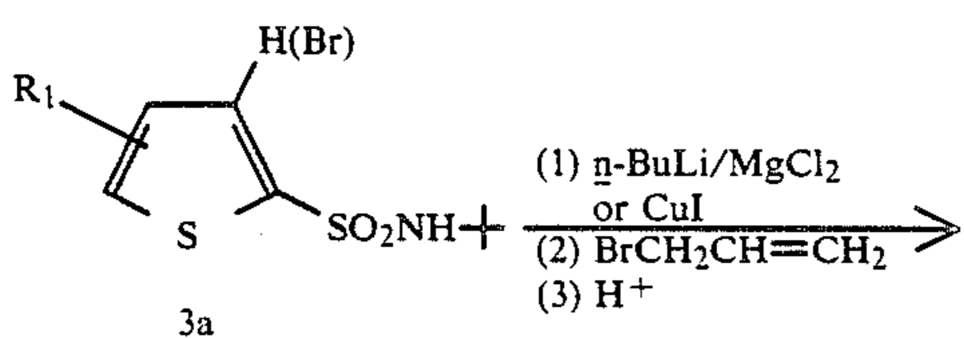
Equation 4
