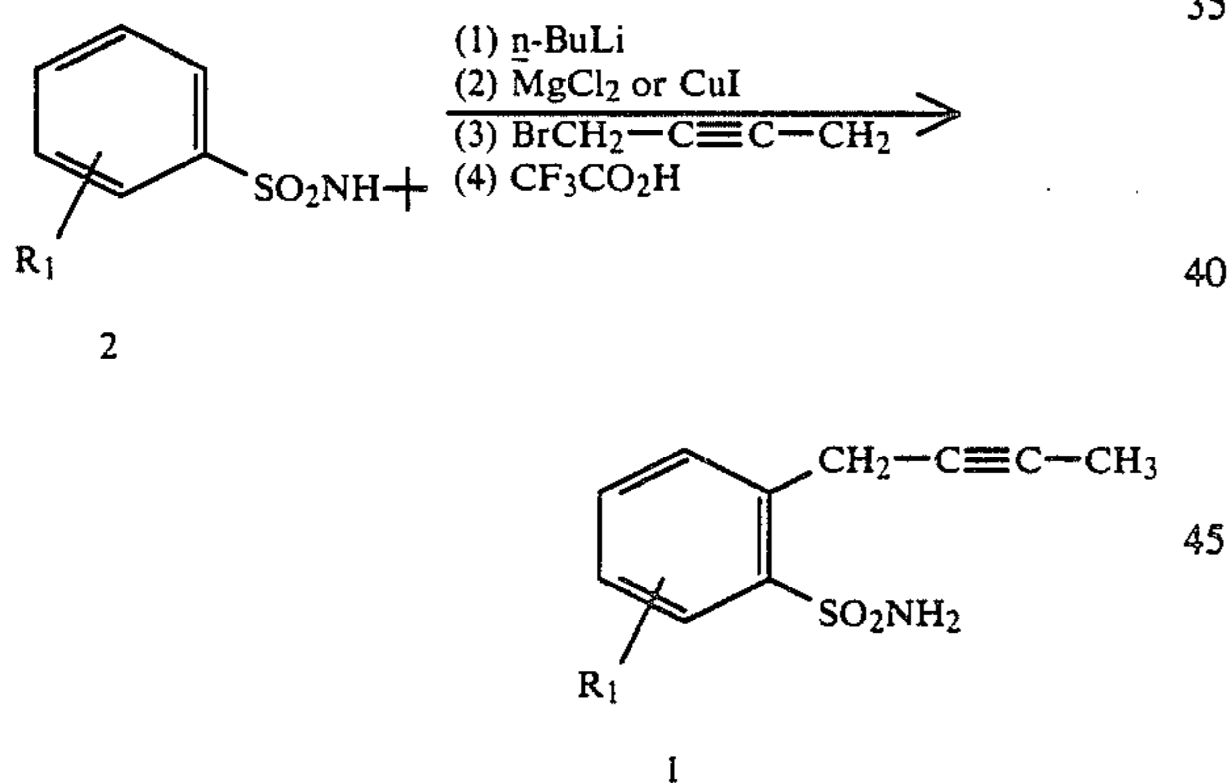
Equation 3
