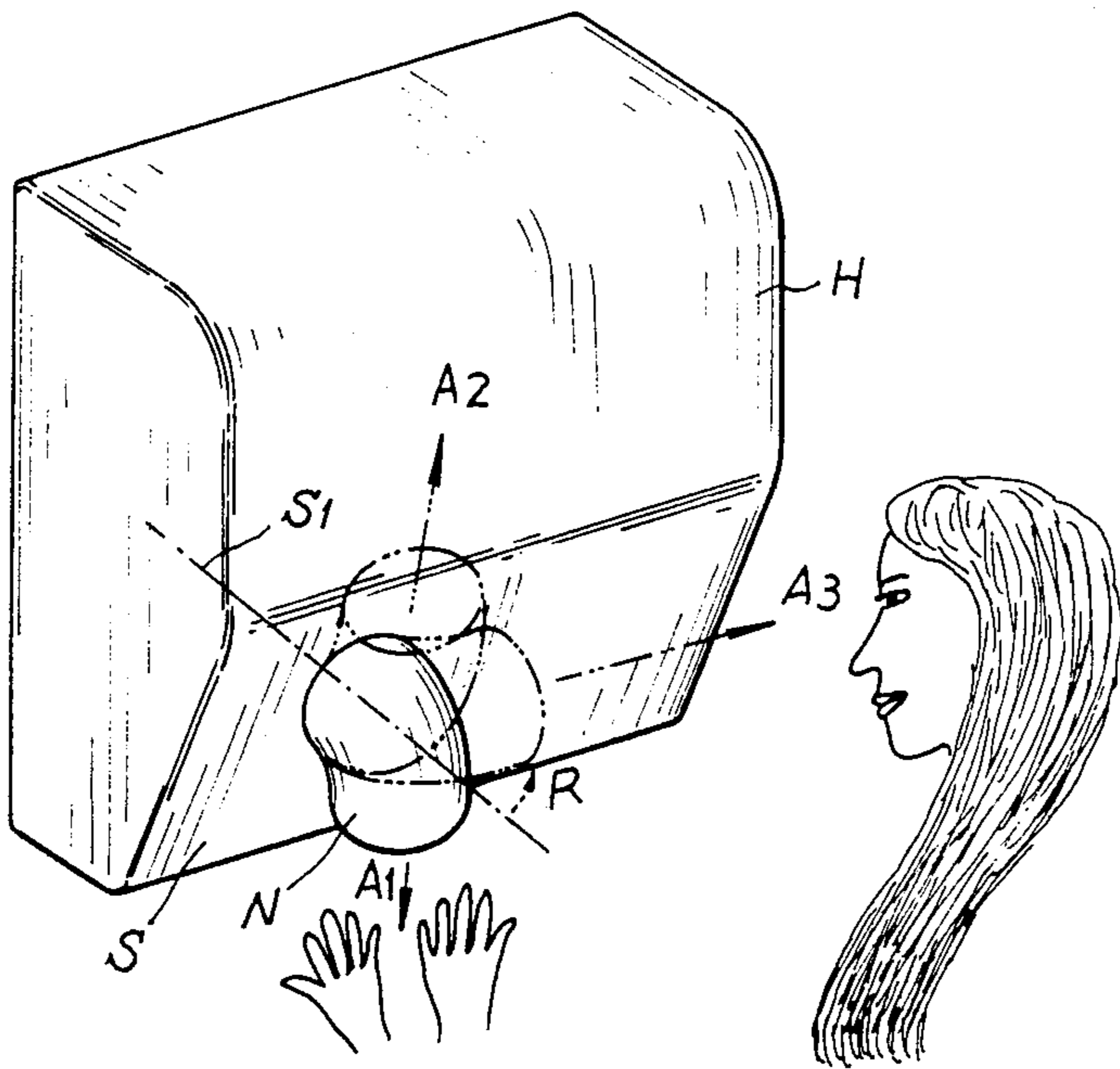
FIG. 1 PRIOR ART
