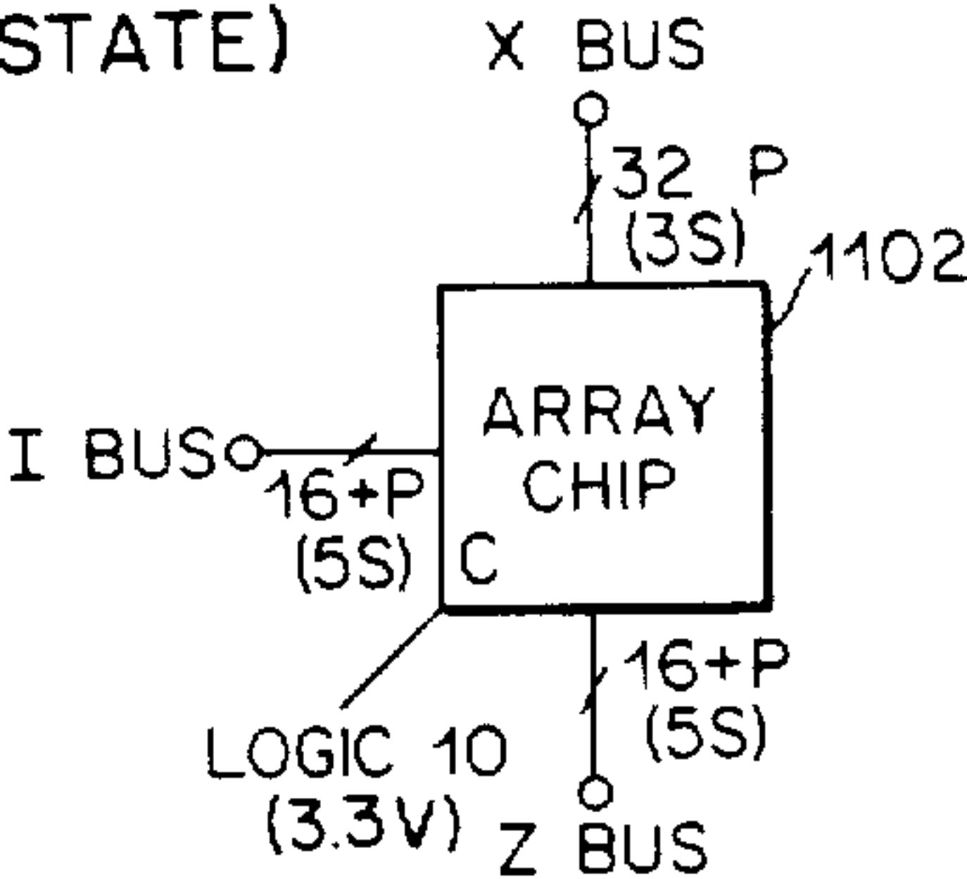
D. MAXIMUM INTERCONNECT (4*5-STATE)
