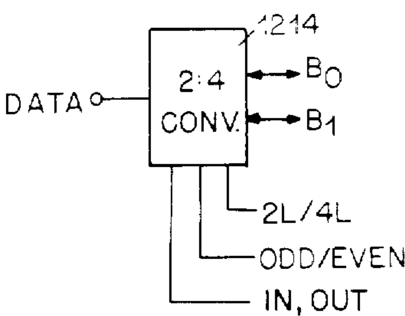
FIG. 10 C. 2:4 LEVEL CONVERTER SYMBOL
