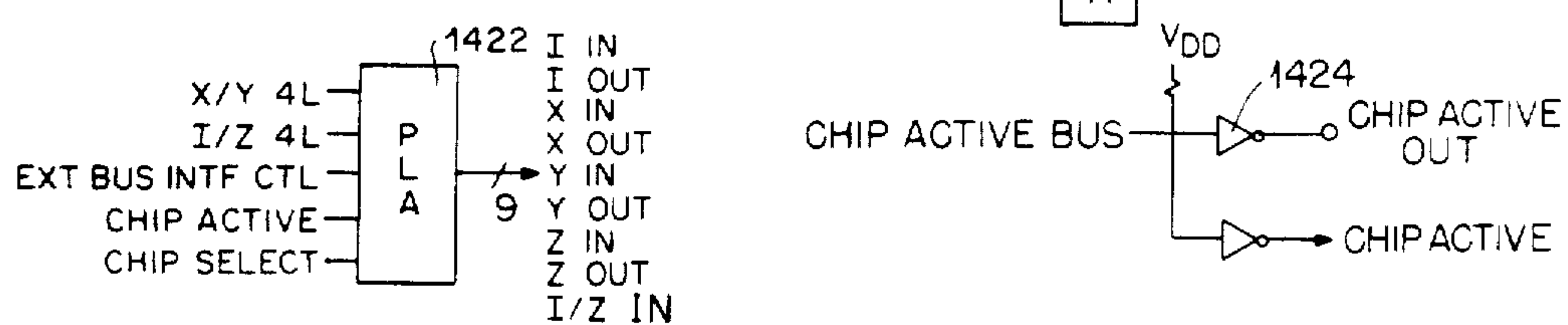
FIG. 12B. COMMON CONTROL LOGIC
