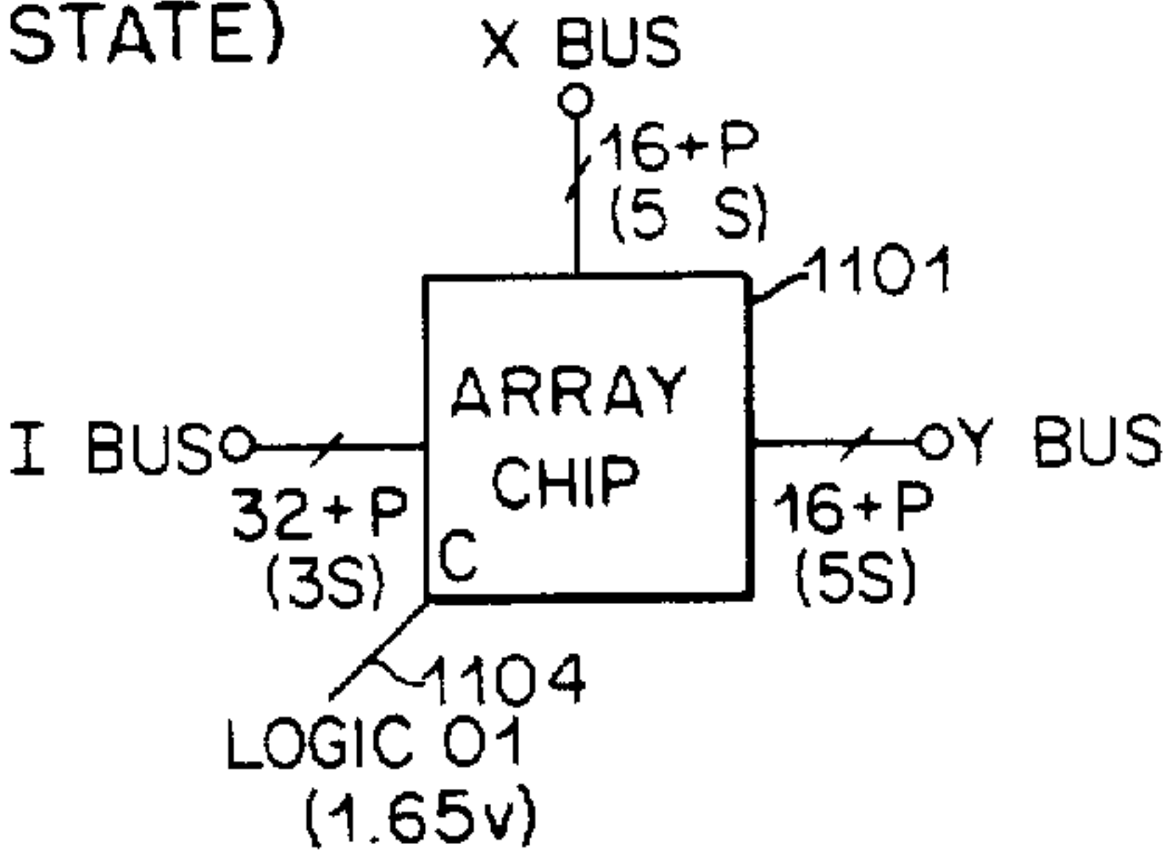
C. MEDIUM INTERCONNECT B (1*3-STATE, 2*5 STATE)
