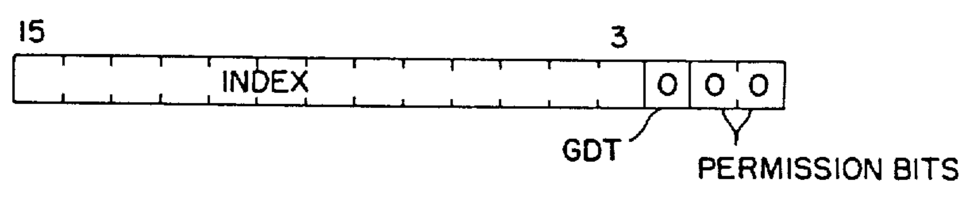
FORMAT FOR PROTECTED MODE SEGMENT SELECTOR DESIGNATING GLOBAL ADDRESS SPACE
