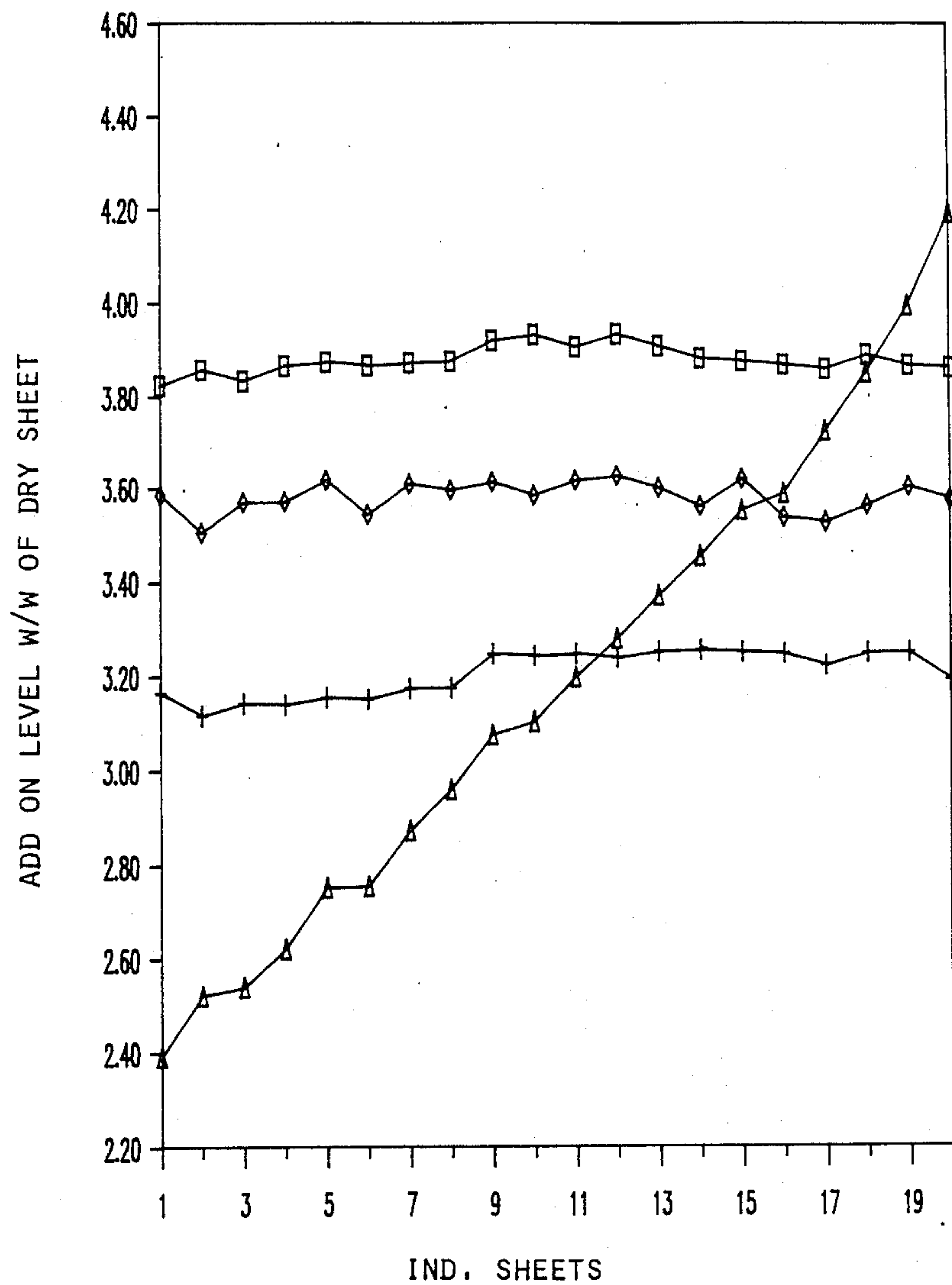
Figure 2E Liquid Retention 1 MONTH AT 50°C
