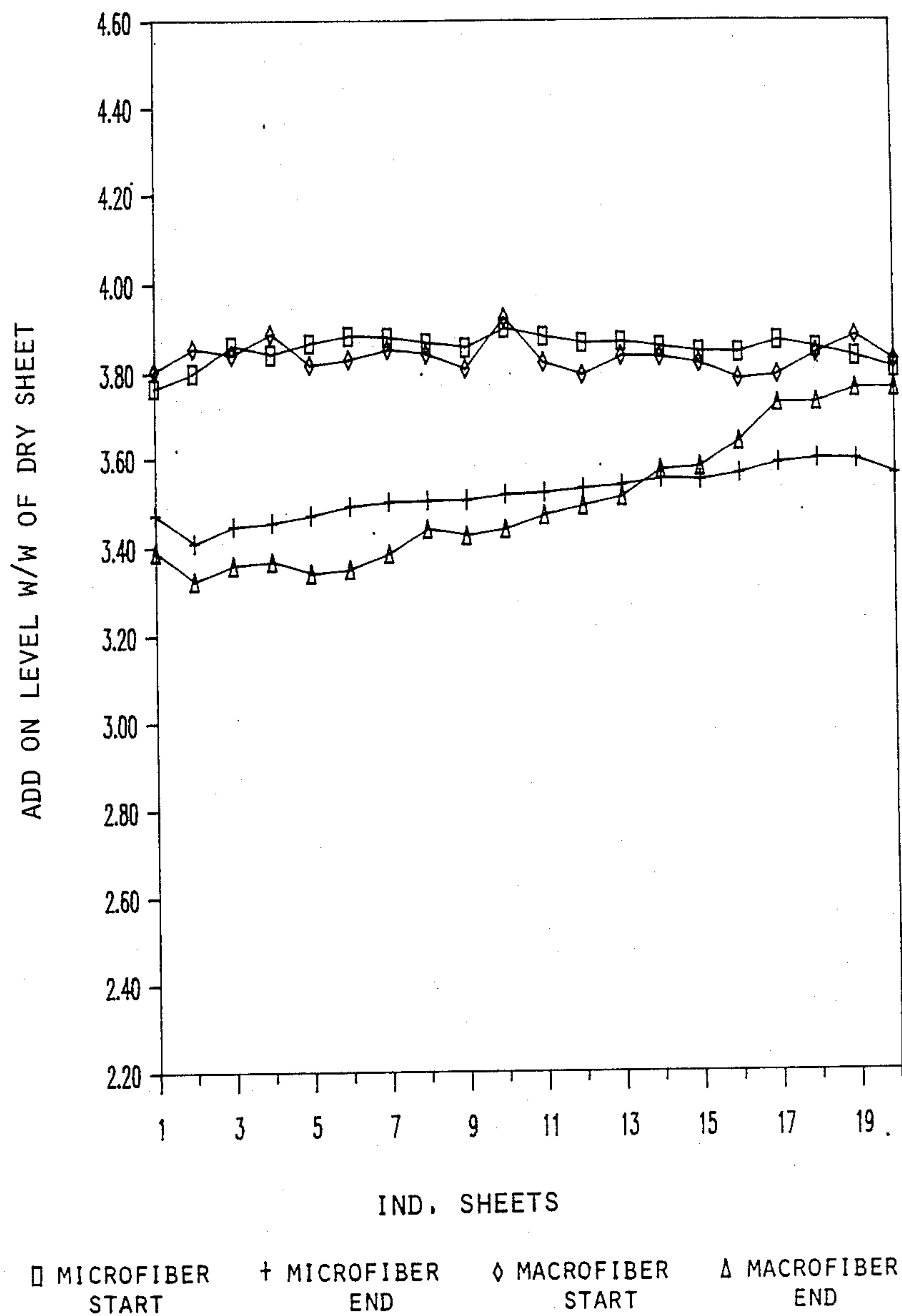
Figure 2D Liquid Retention 1 MONTH AT 40°C
