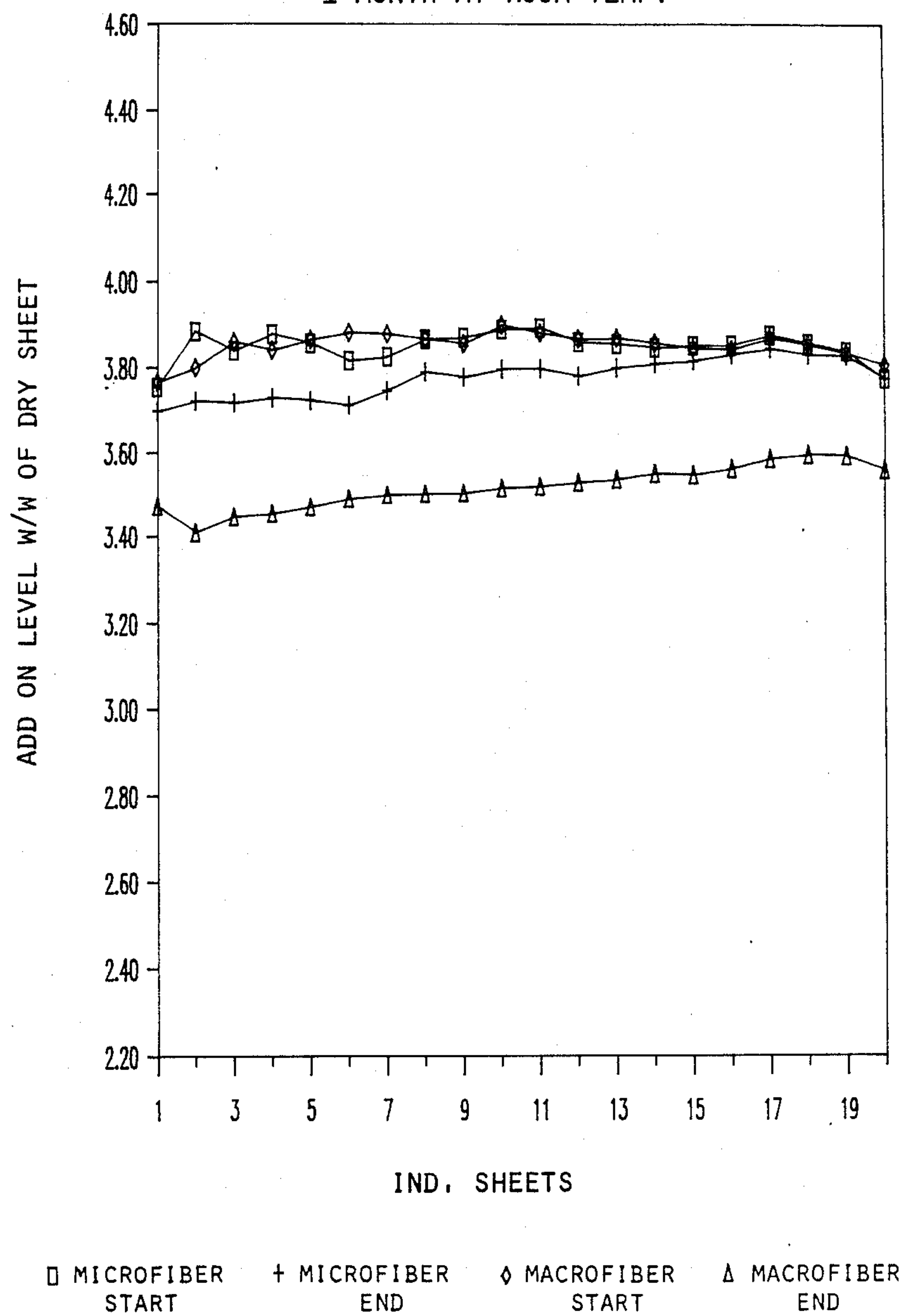
Figure 2B Liquid Retention 1 MONTH AT ROOM TEMP.
