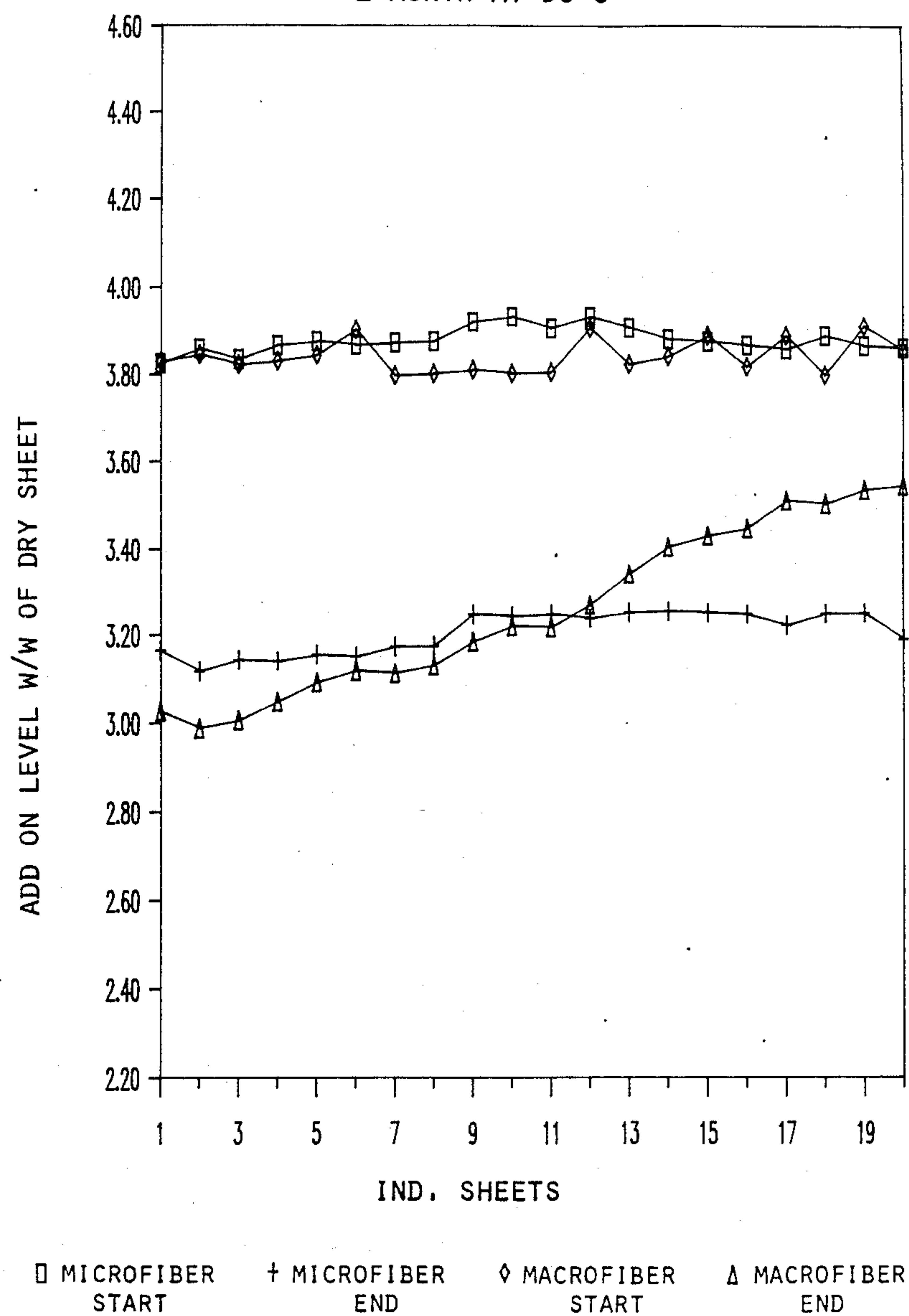
Figure 2F Liquid Retention 1 MONTH AT 50°C
