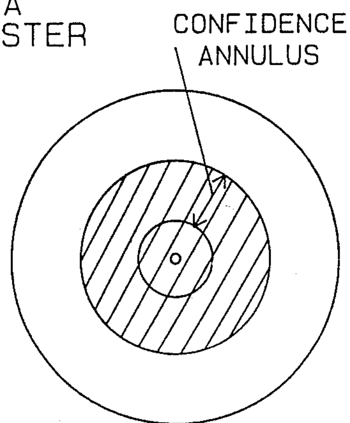
FIG 3C CONFIDENCE SPHERE
