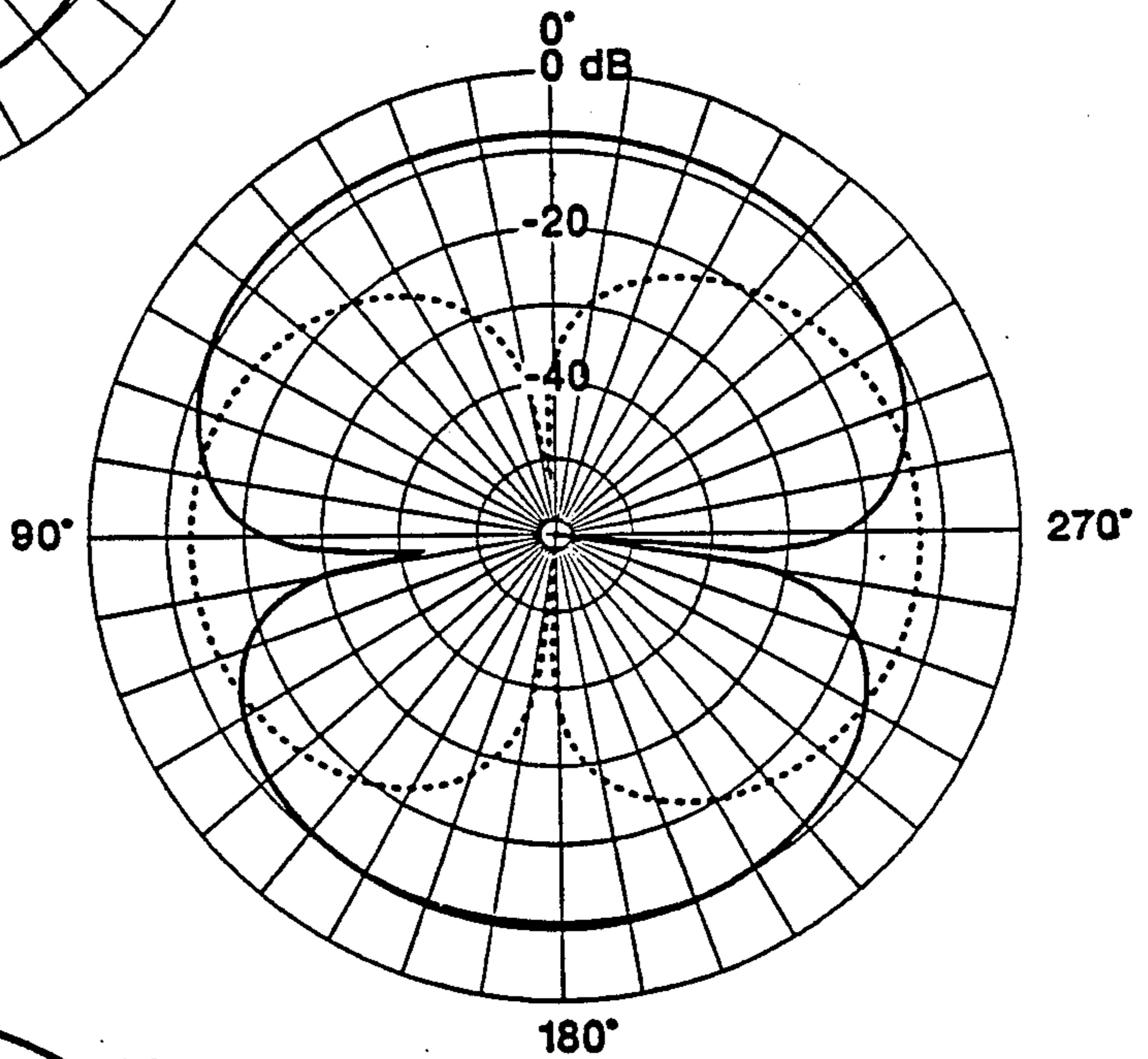
SLOT ANTENNA WITHOUT PASSIVE GROUND ELEMENT
