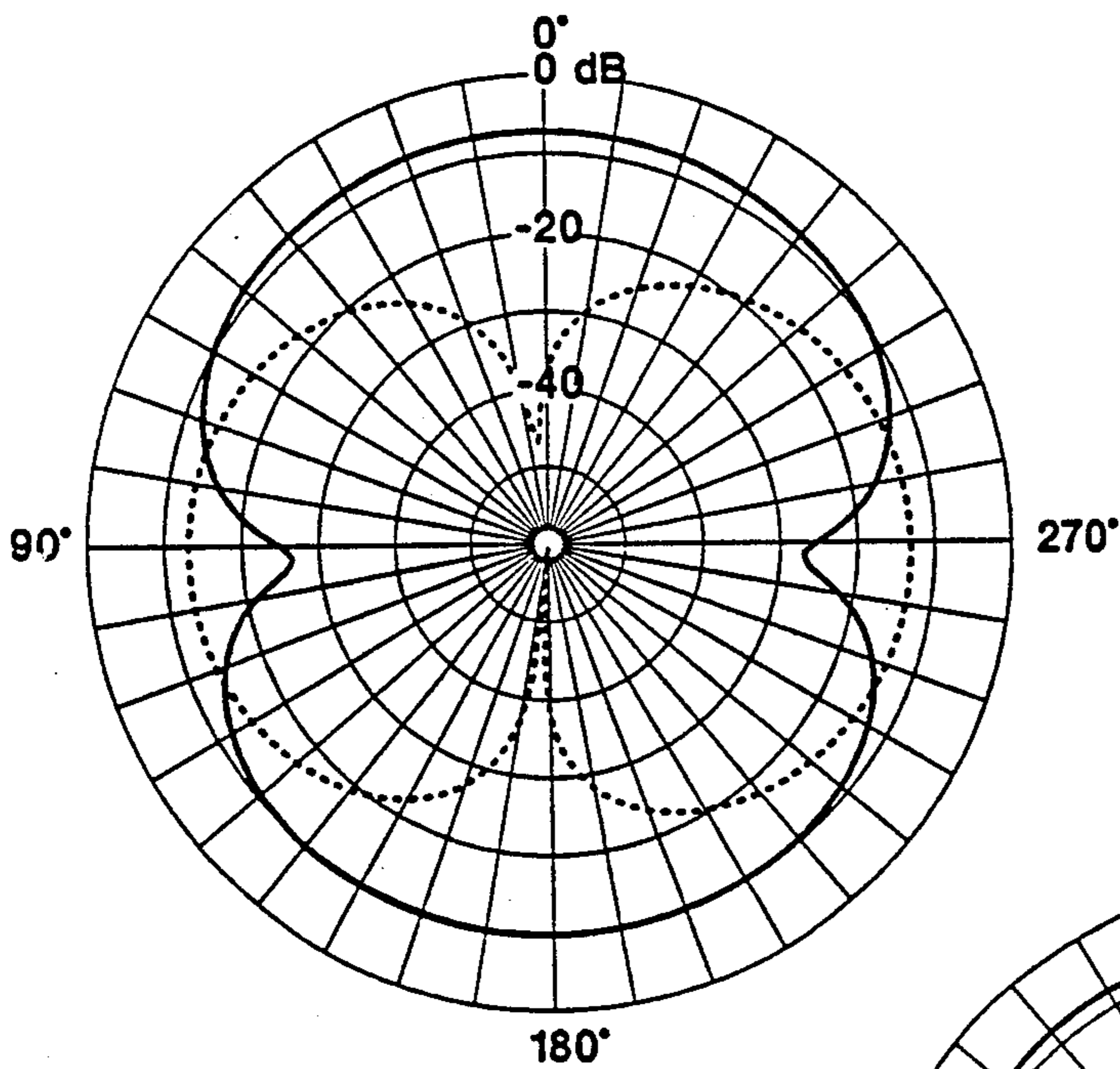
SLOT ANTENNA WITH PASSIVE GROUND ELEMENT
