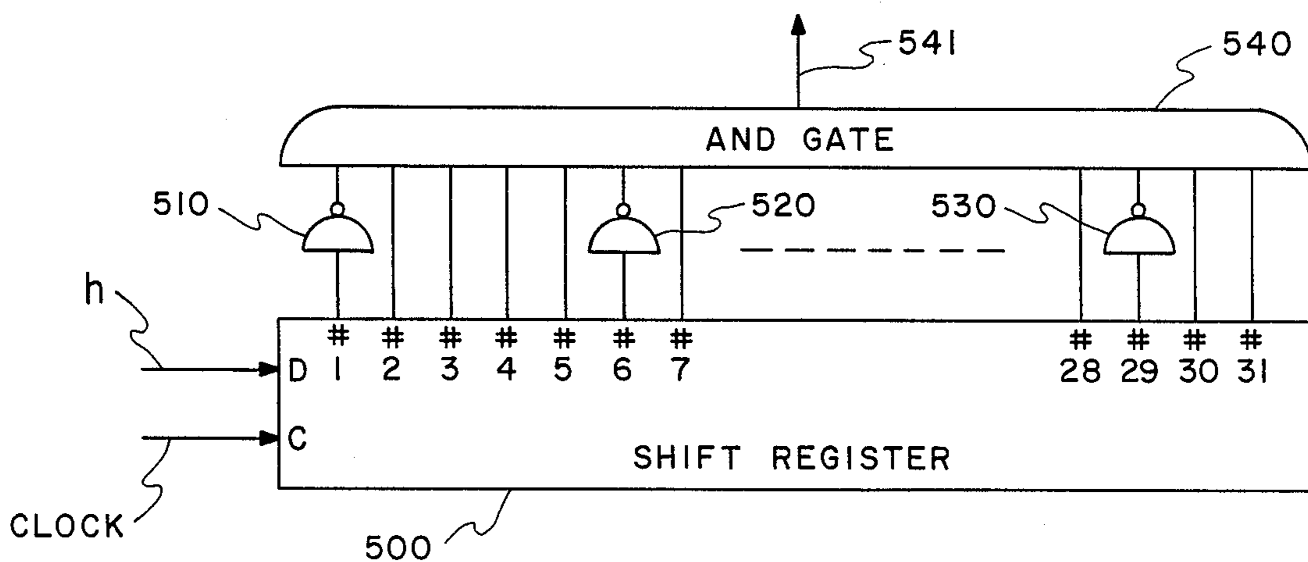
FRAME SYNCHRONIZATION AND END SIGNAL DETECTOR
