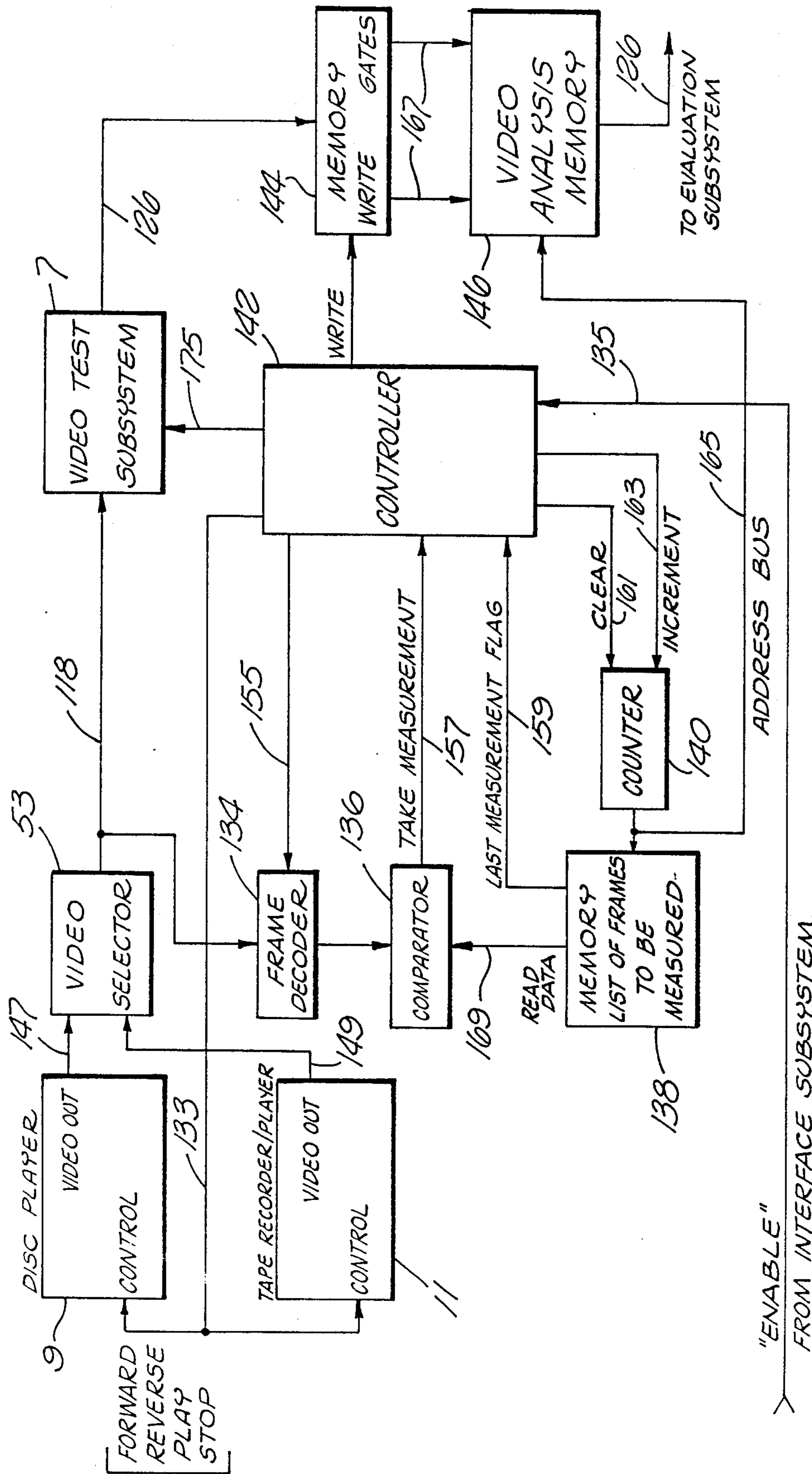
FIG. 22 VIDEO ANALYSIS LOGIC FROM INTERFACE SUBSYSTEM.
