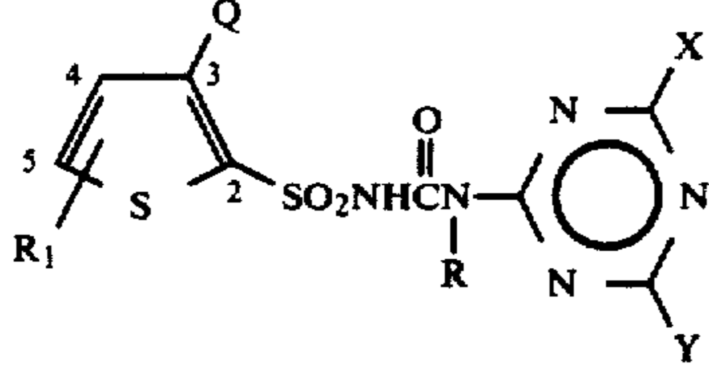
General Formula 11
