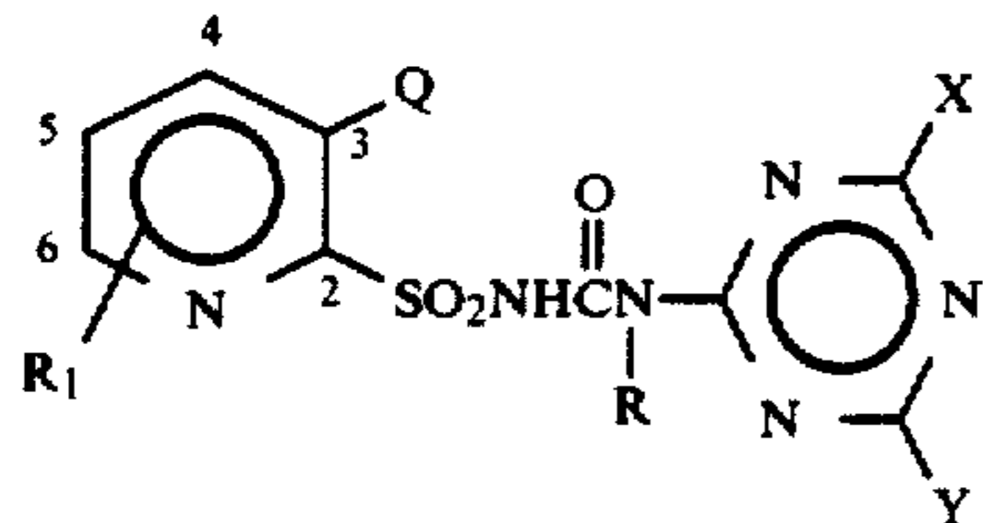
General Formula 15
