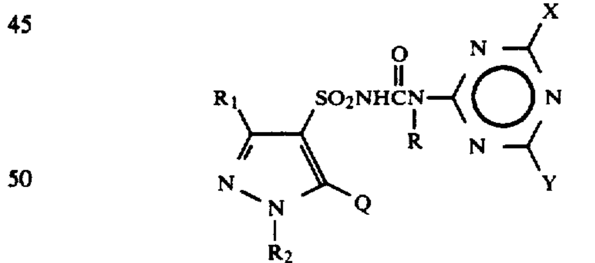
General Formula 21
