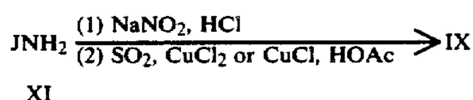
Equation 9
