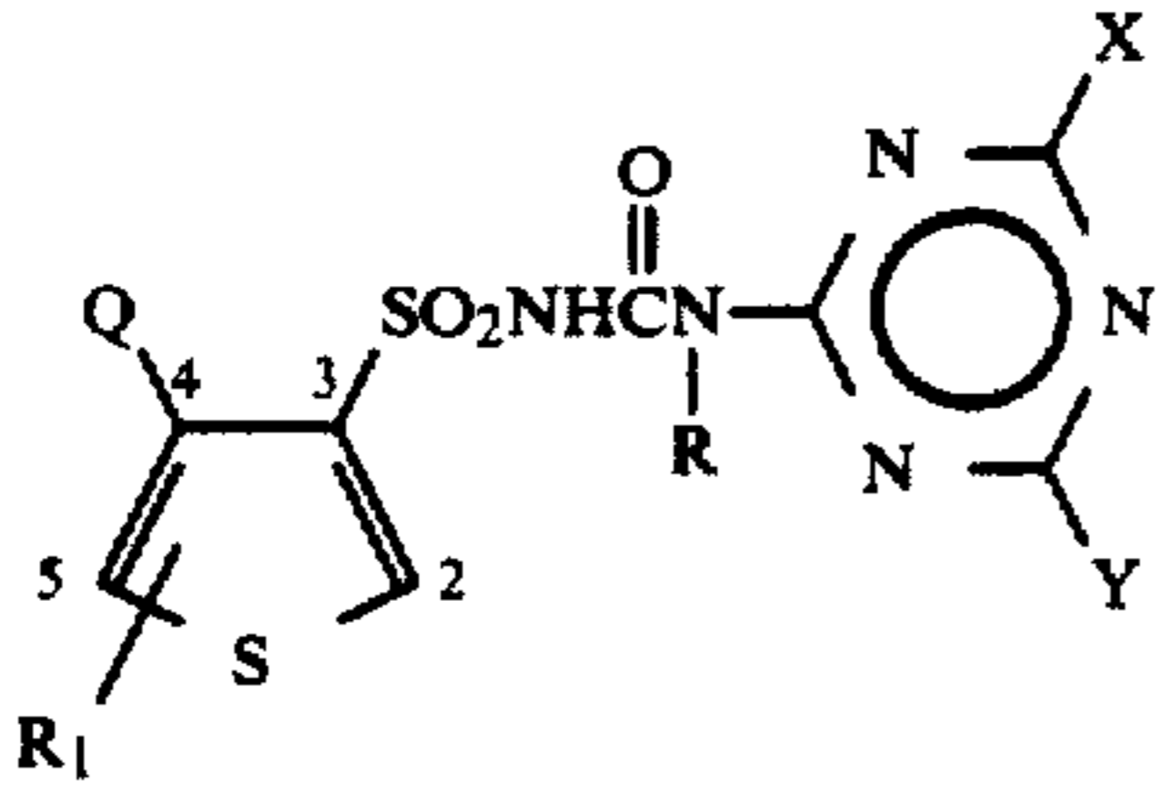
General Formula 13
