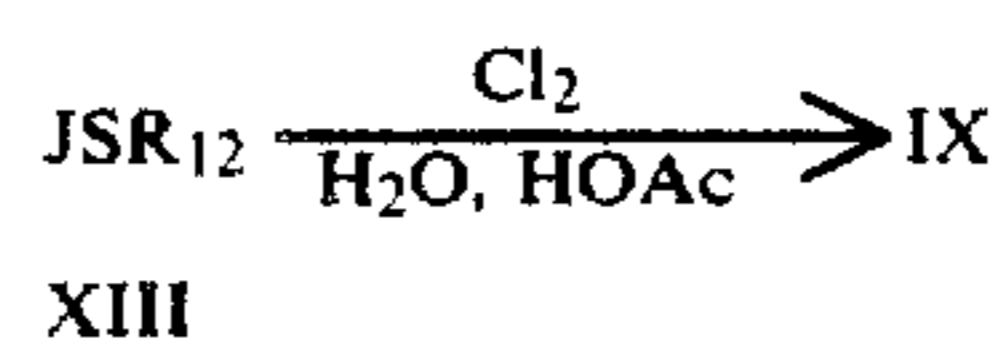
Equation 11
