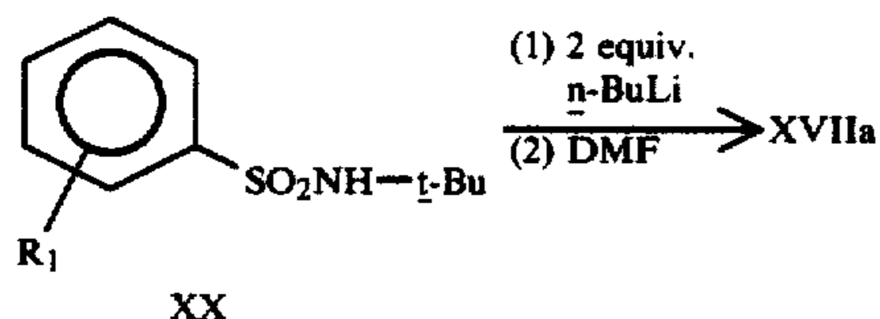
Equation 19a
