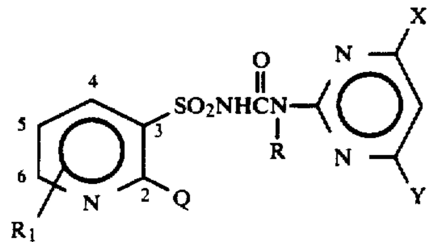
General Formula 16
