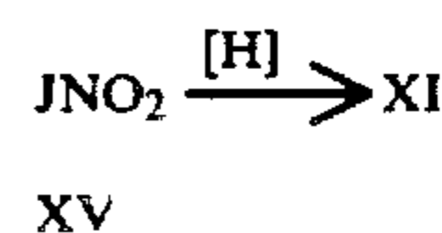
Equation 12
