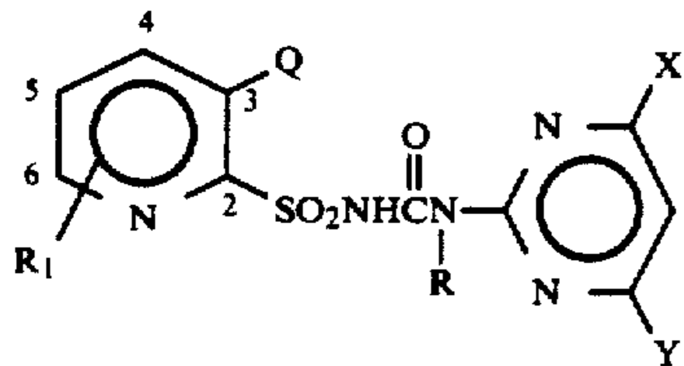
General Formula 14
