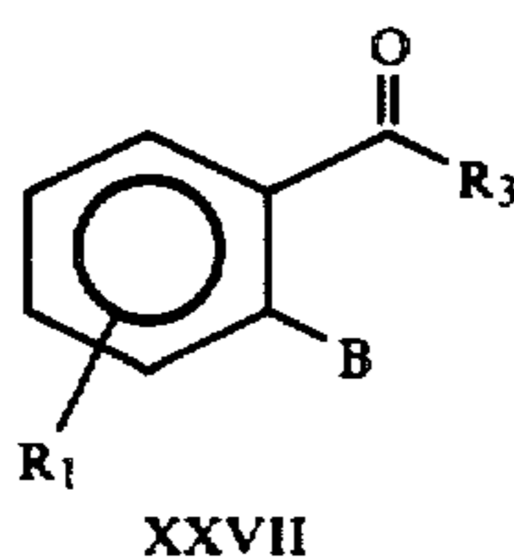
Equation 21
