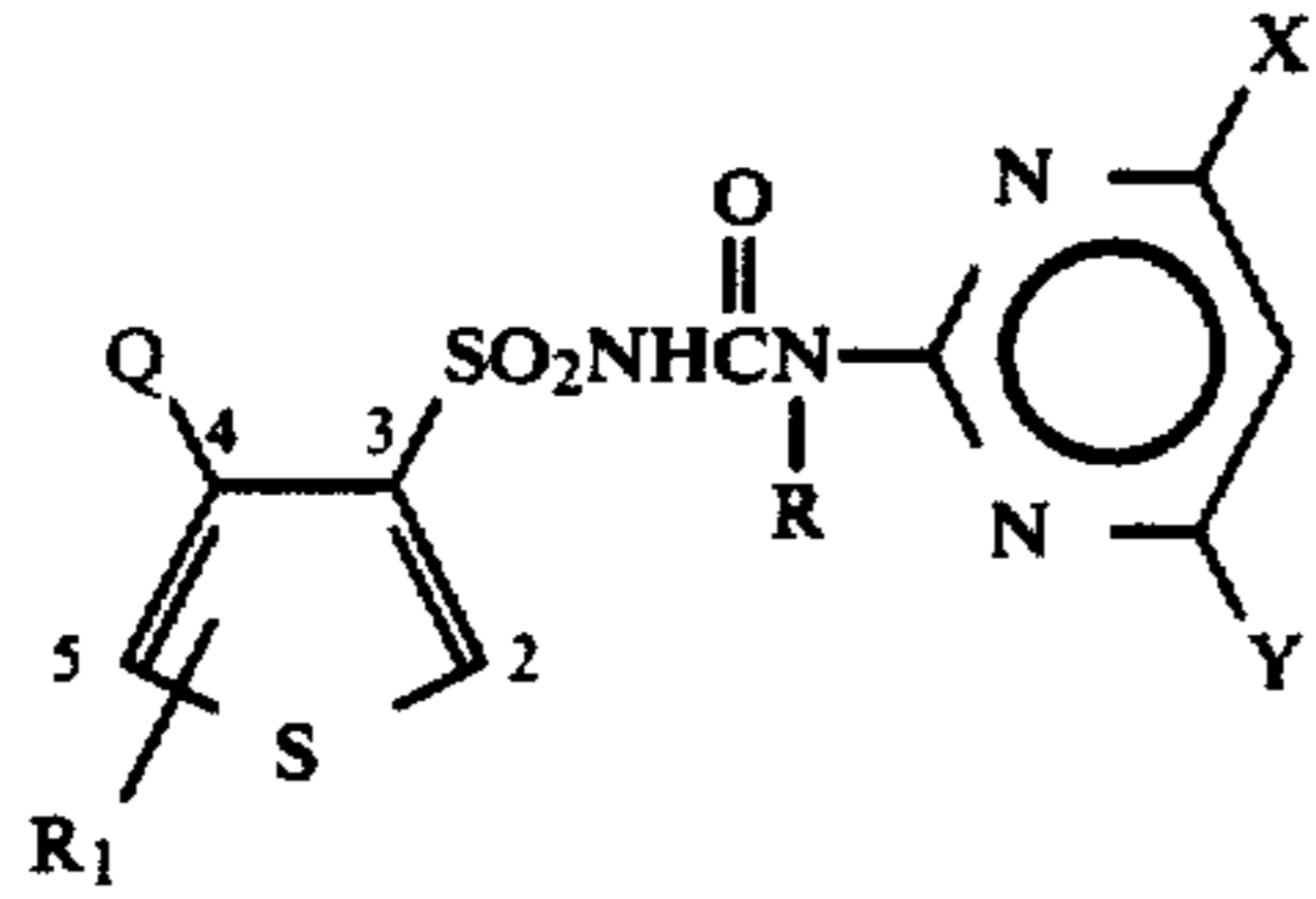
General Formula 12
