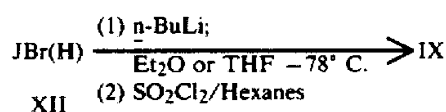
Equation 10
