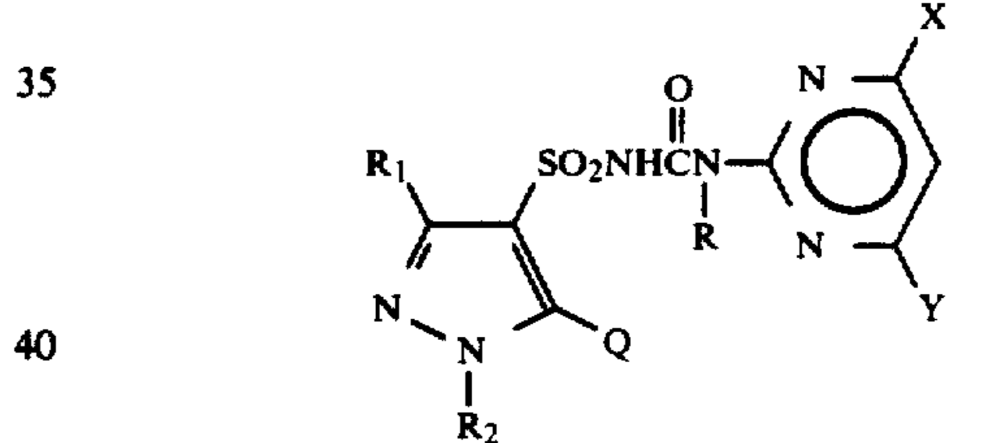
General Formula 20
