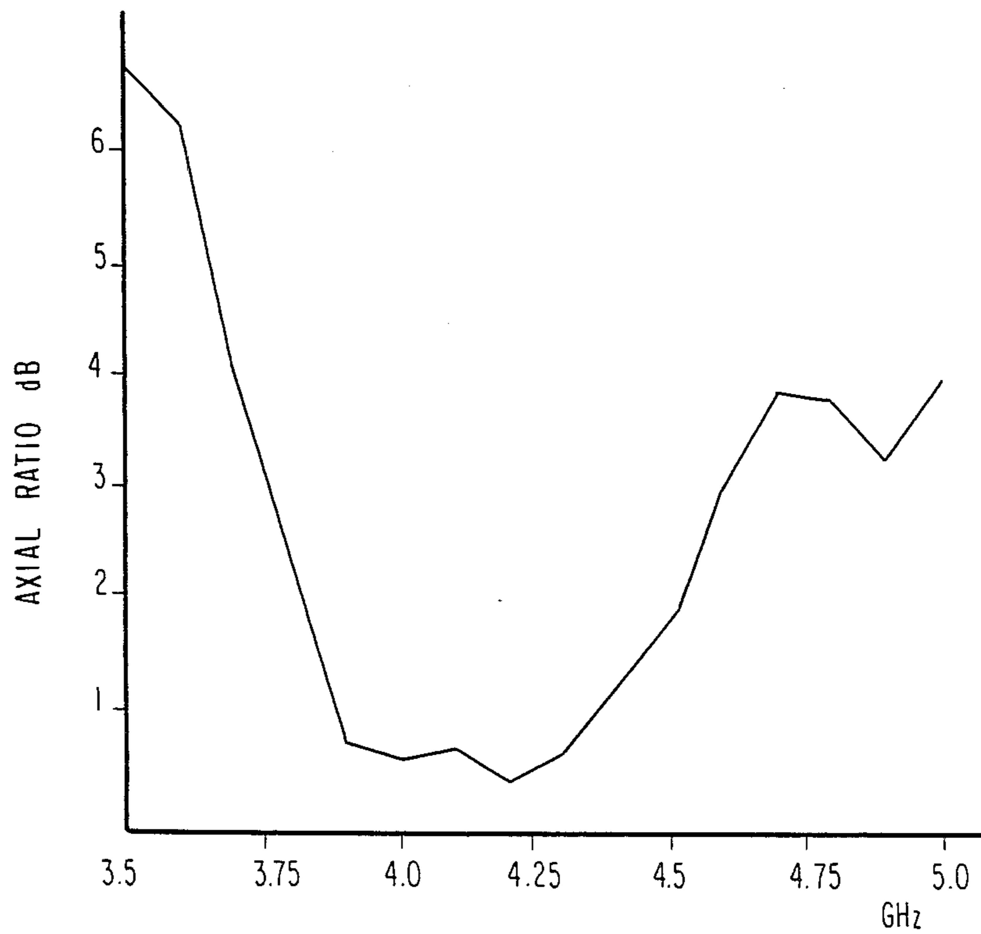
FIG. 7 - AXIAL RATIO OF 4-ELEMENT ARRAY
