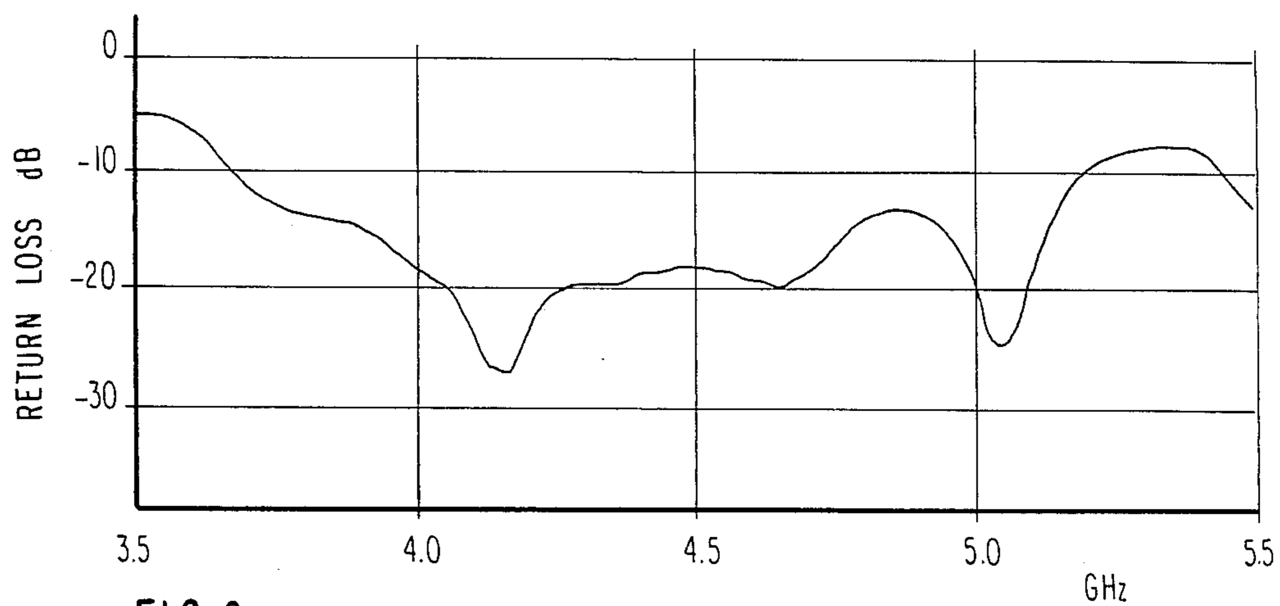
FIG. 6 - RETURN LOSS OF 4-ELEMENT CIRCULARLY POLARIZED CF-EMCP
