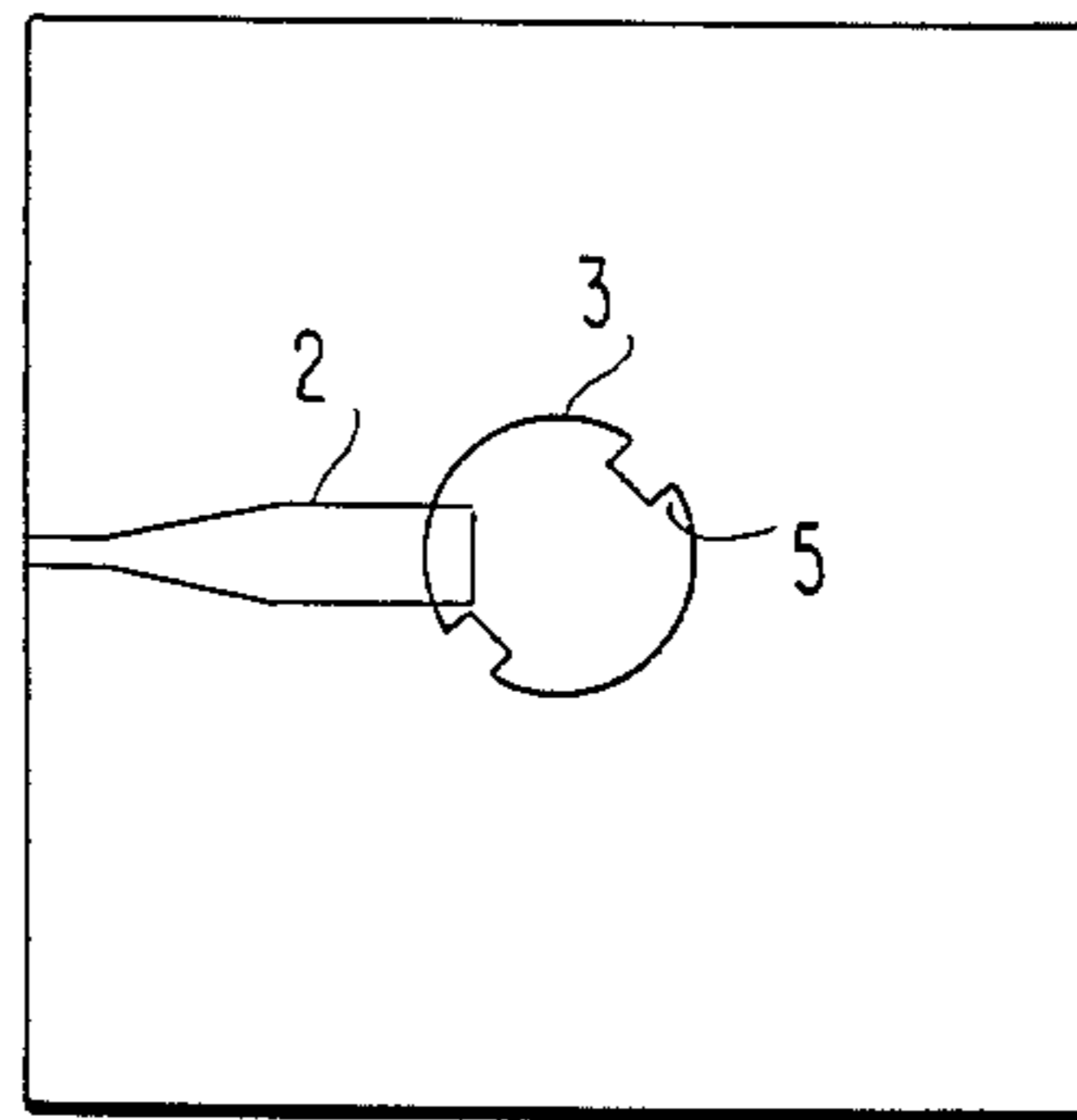
FIG. 3a - CONFIGURATION OF CIRCULARLY POLARIZED CF-EMCP ELEMENT WITH NEGATIVE SEGMENTS (NOTCHES)
