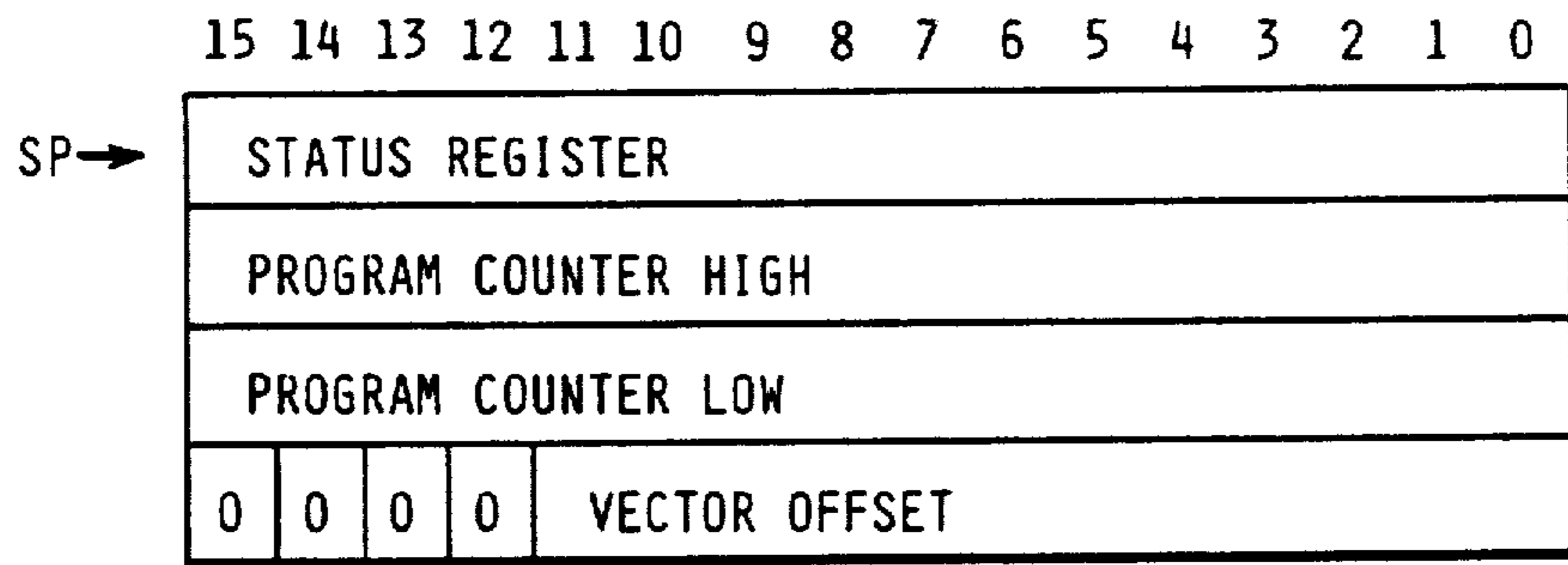
PRE-INSTRUCTION EXCEPTION STACK FRAME
