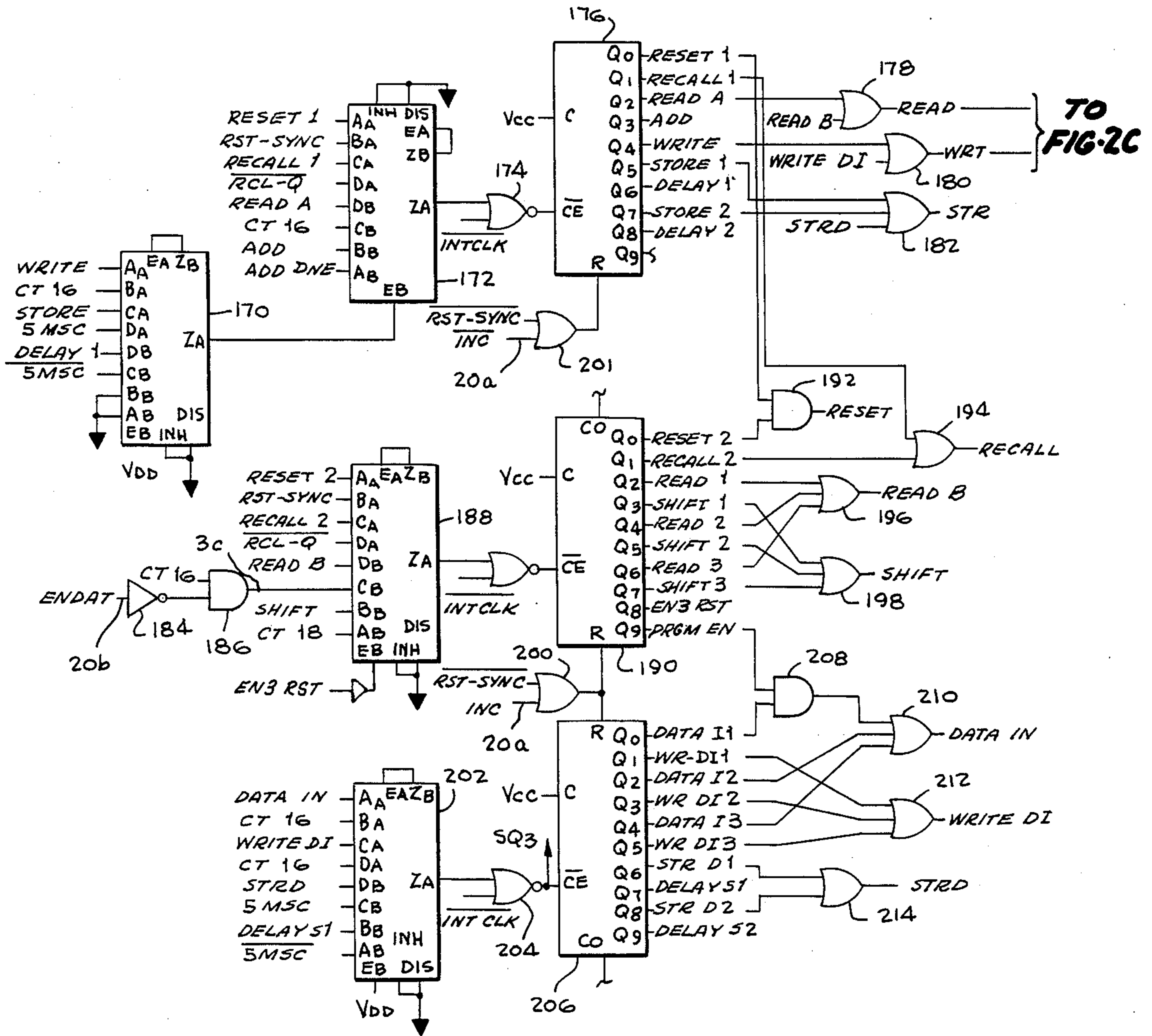
SEQUENTIAL CONTROL LOGIC 2B
