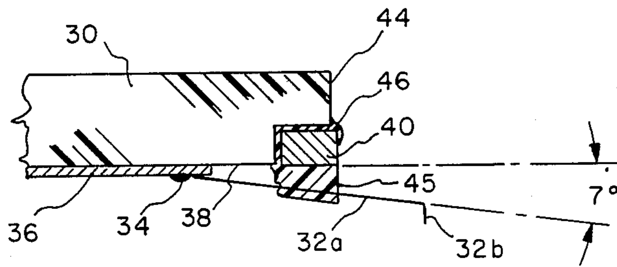
FIG. 2 PRIOR ART
