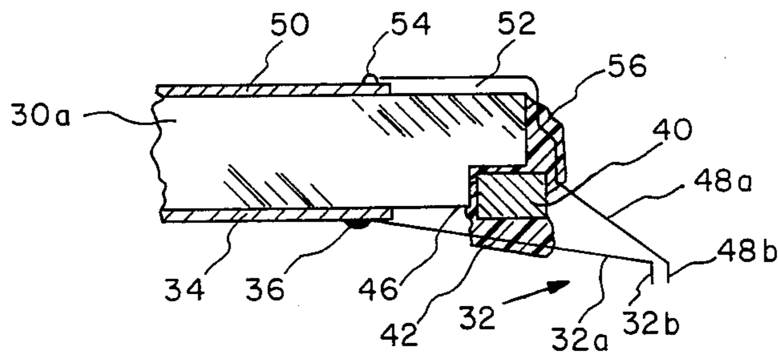
FIG. 3 PRIOR ART
