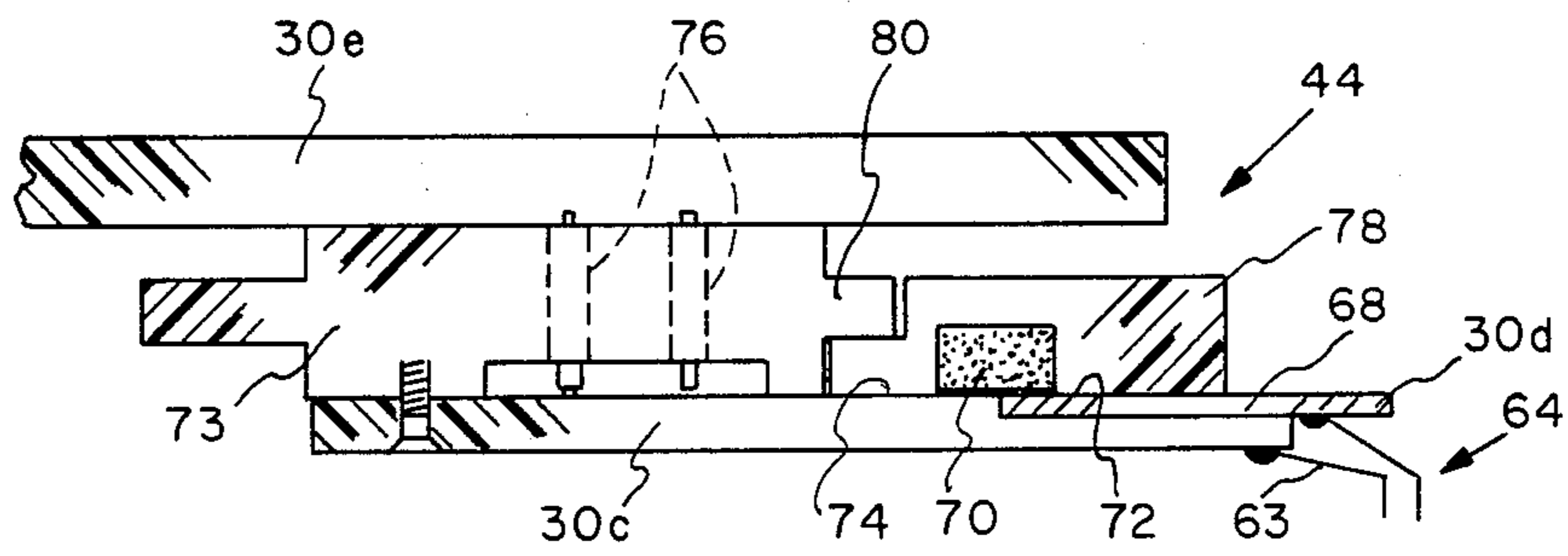
FIG. 5 PRIOR ART
