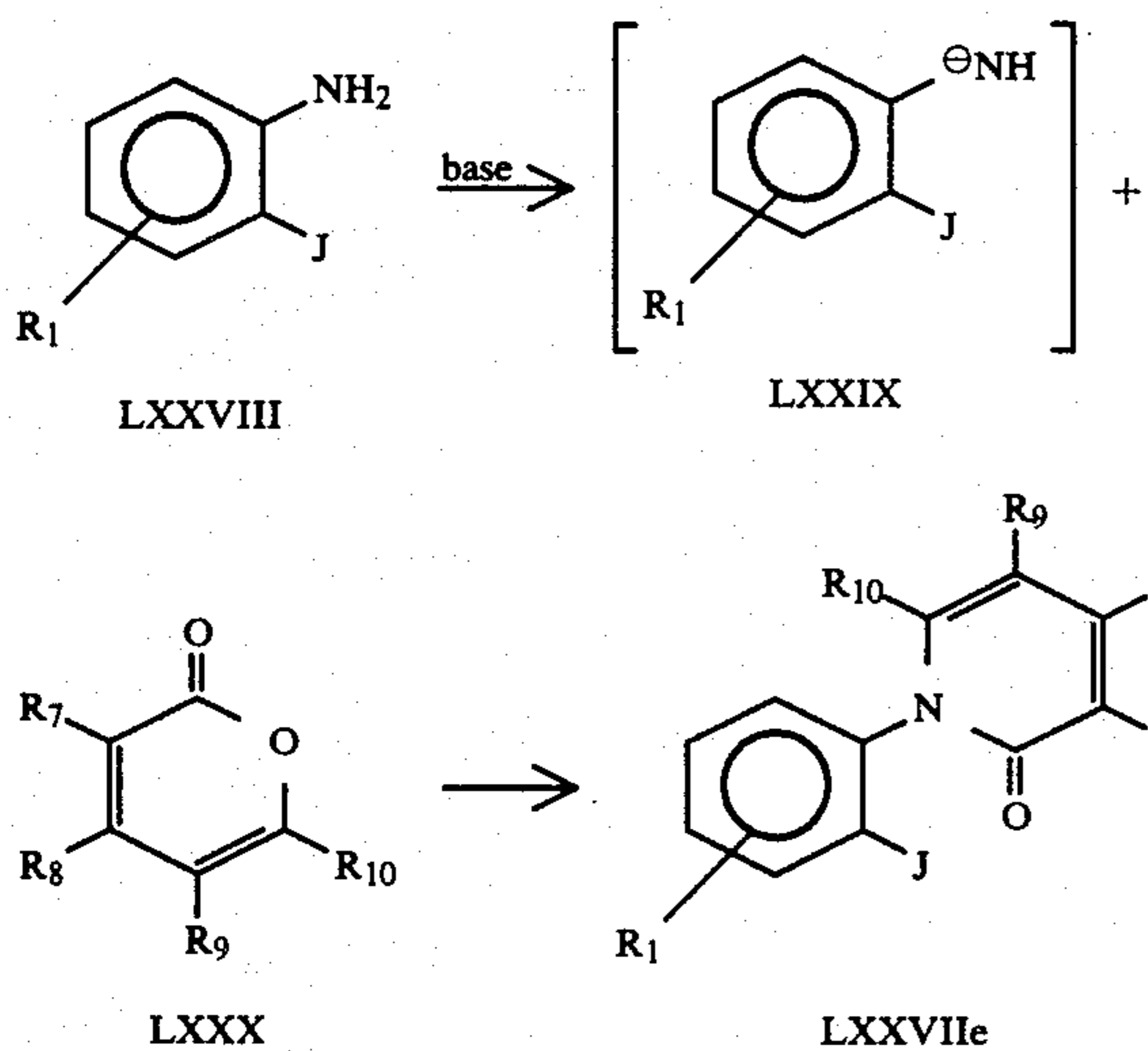
Equation 56
