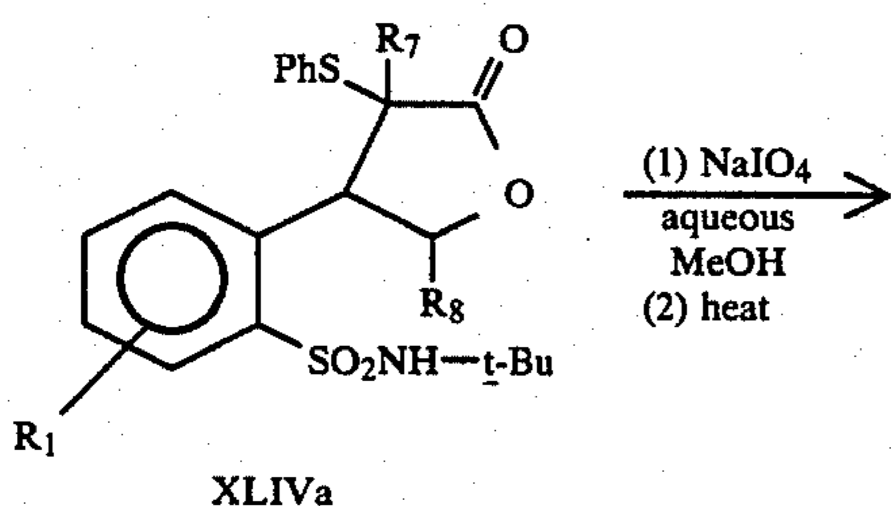
Equation 33
