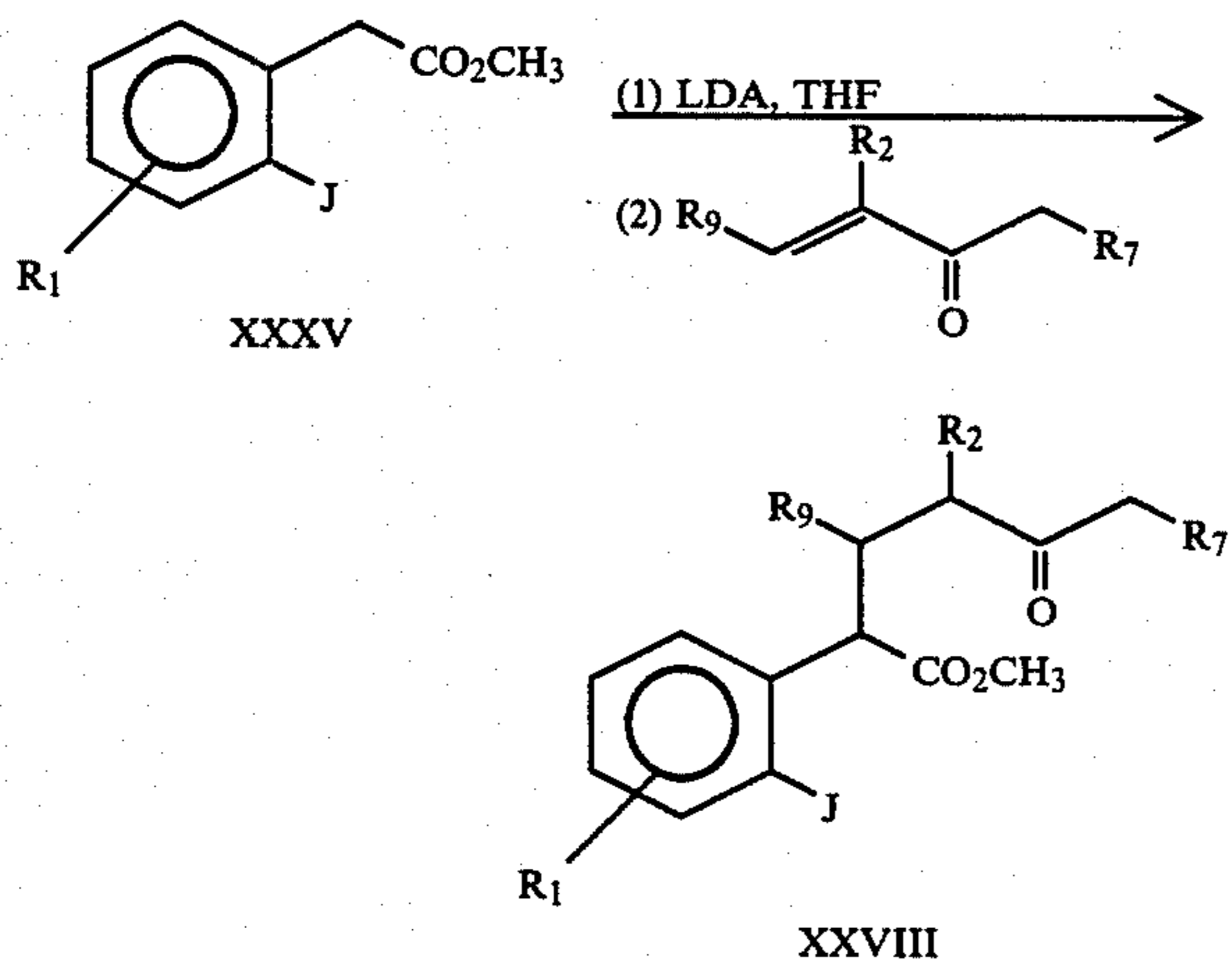
Equation 30
