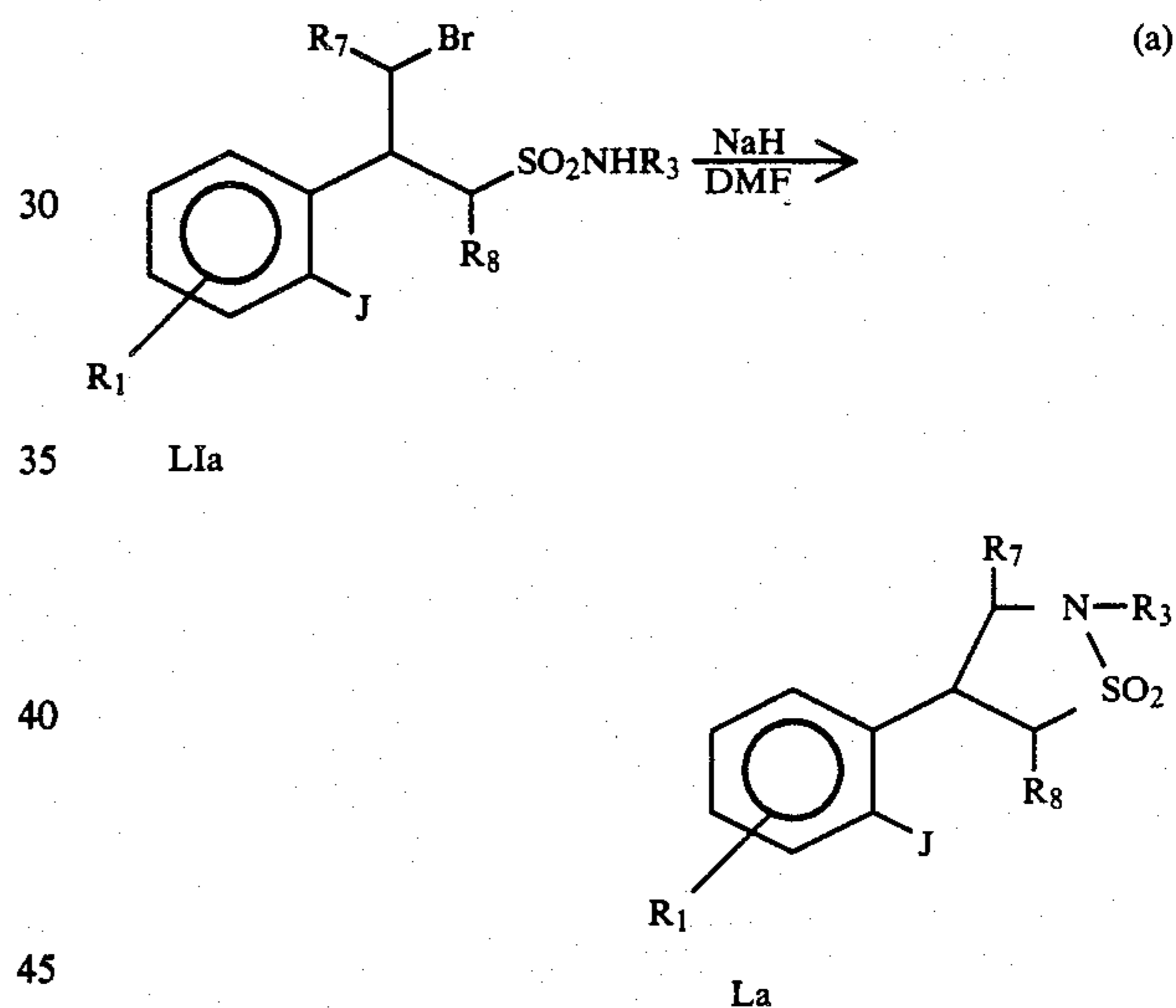
Equation 41
