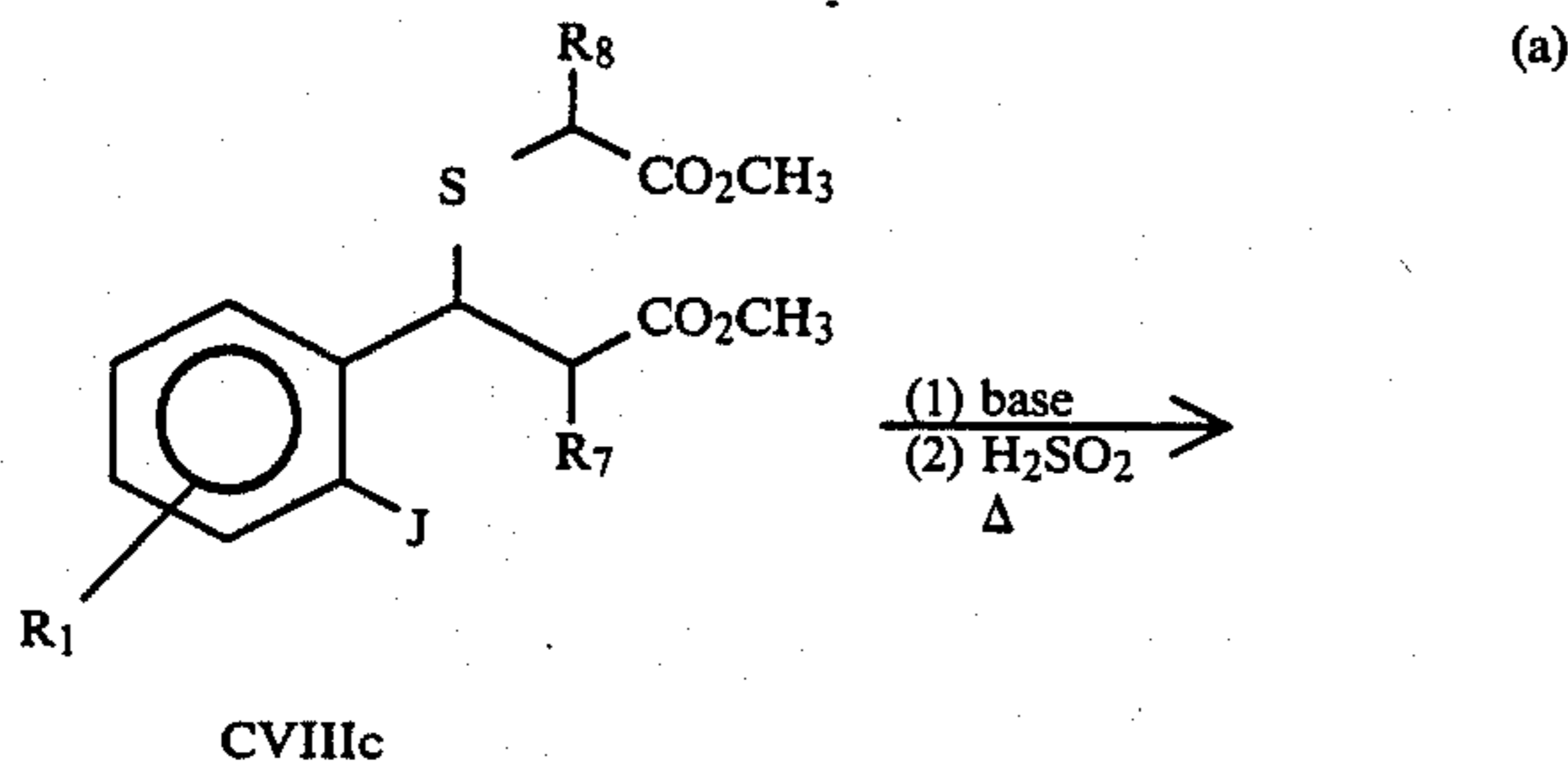
Equation 69
