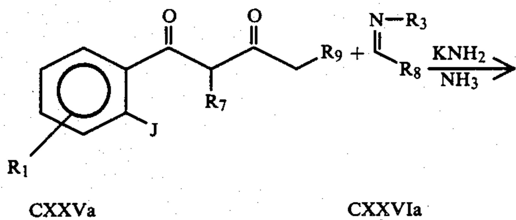
Equation 77
