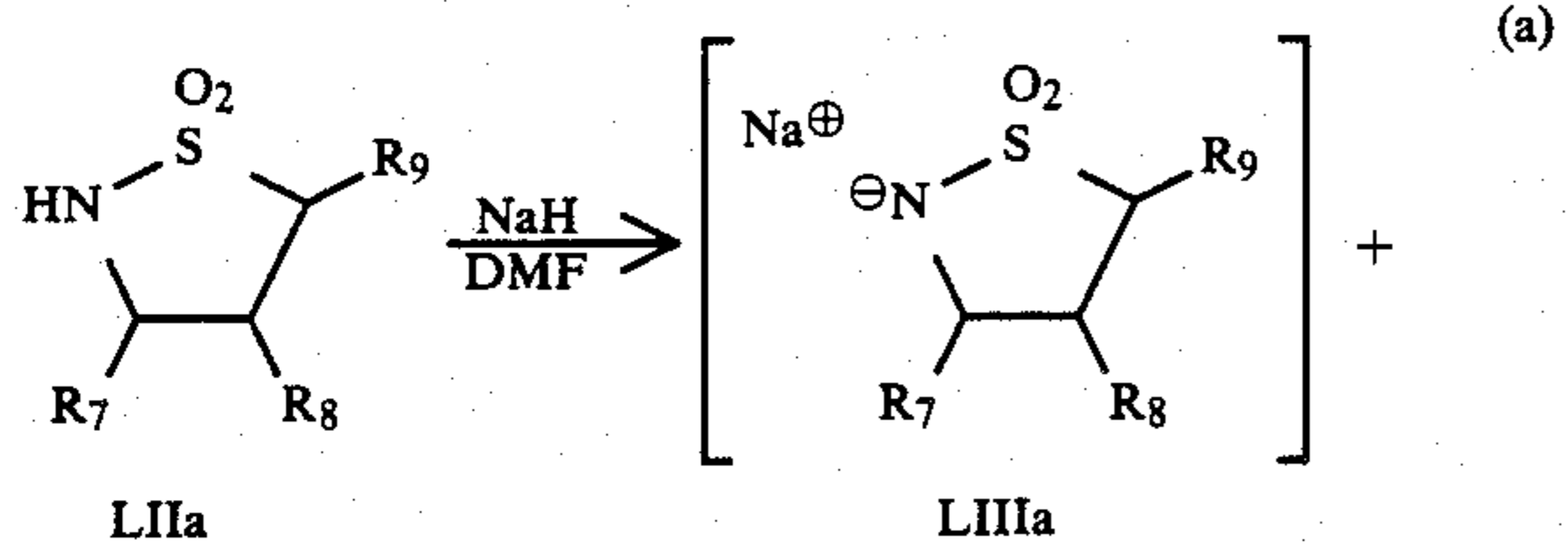
Equation 43
