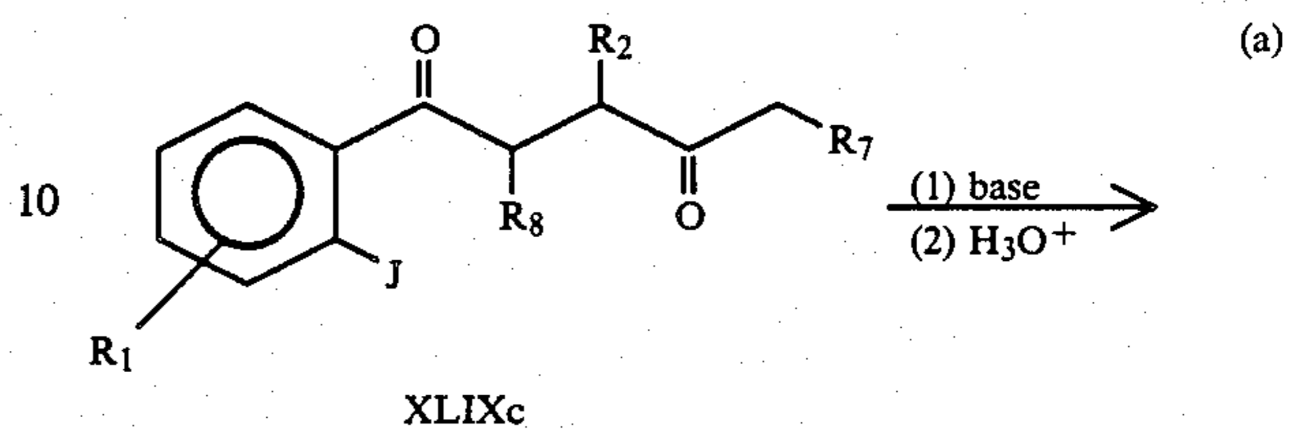
Equation 39
