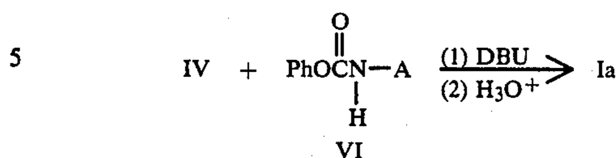
Equation 3
