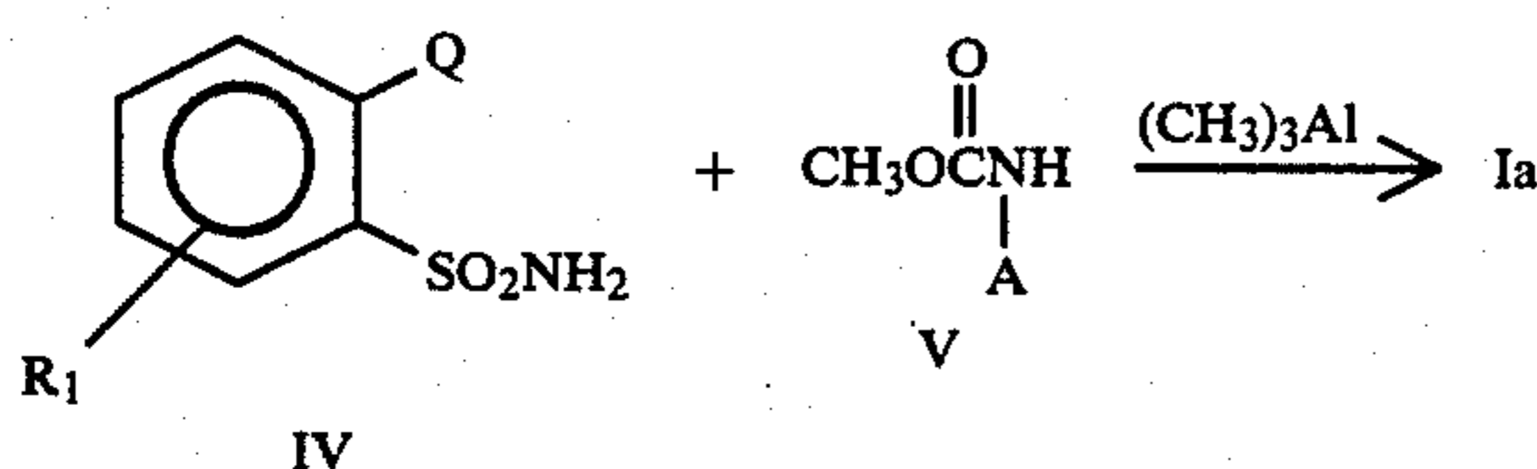
Equation 2
