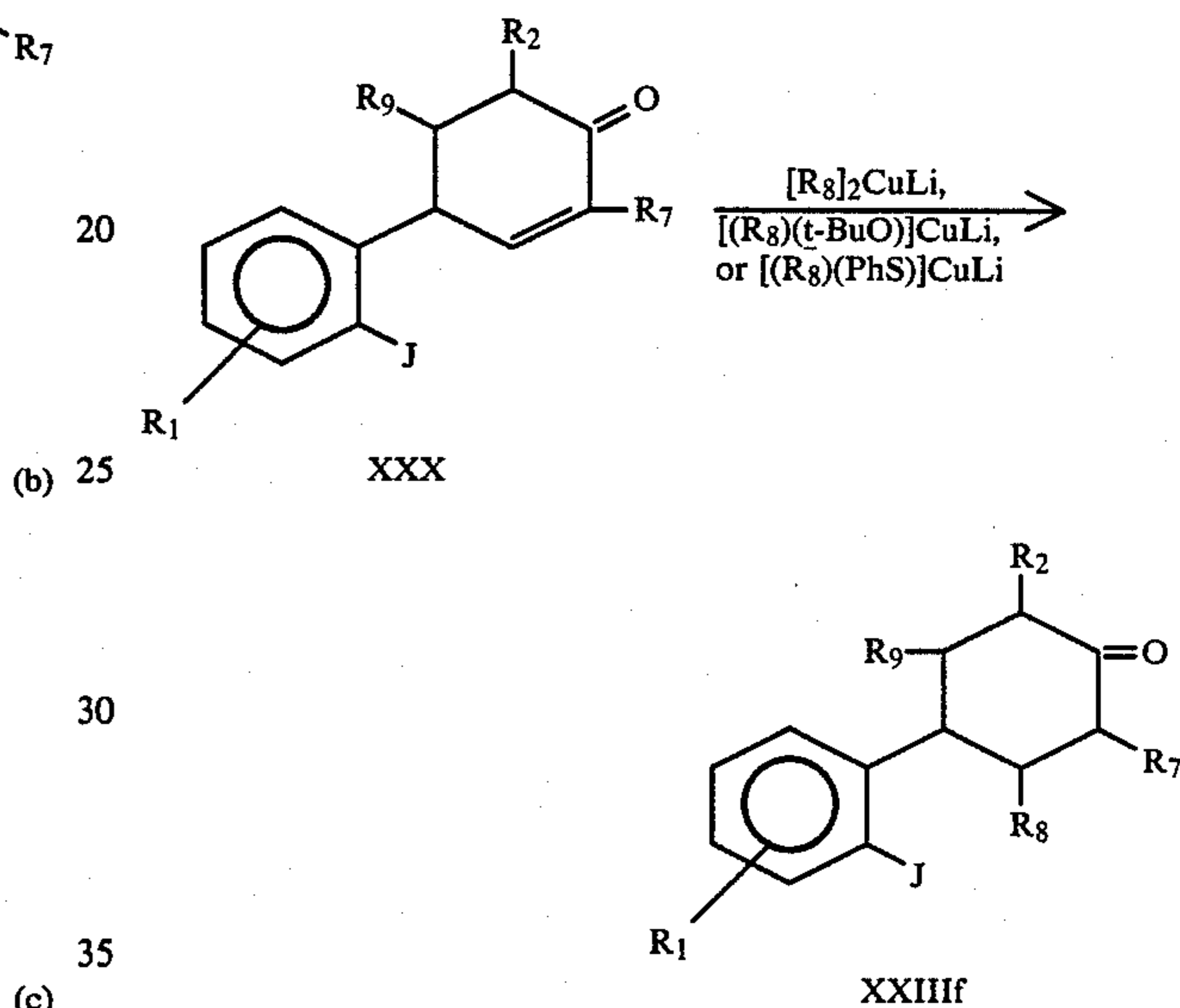
Equation 26
