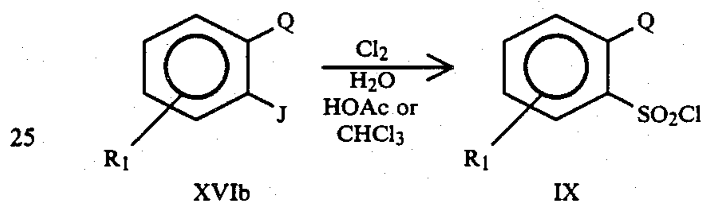
Equation 13
