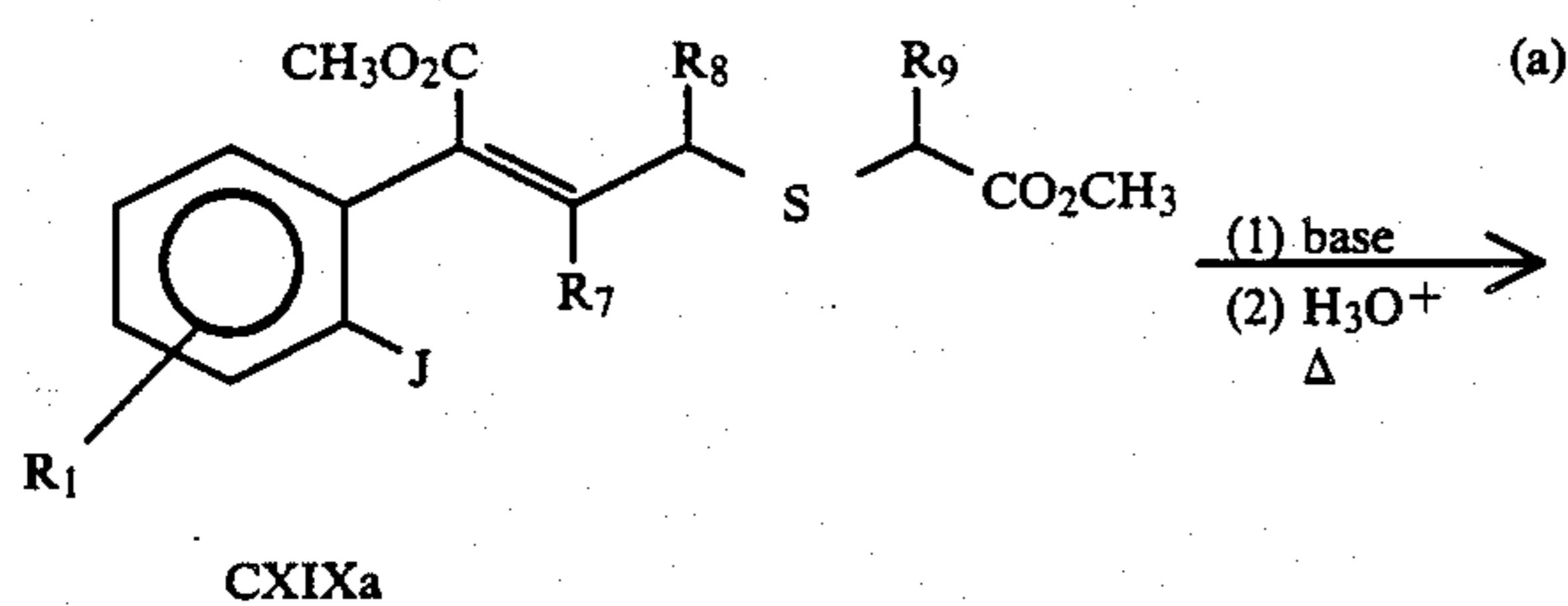
Equation 74
