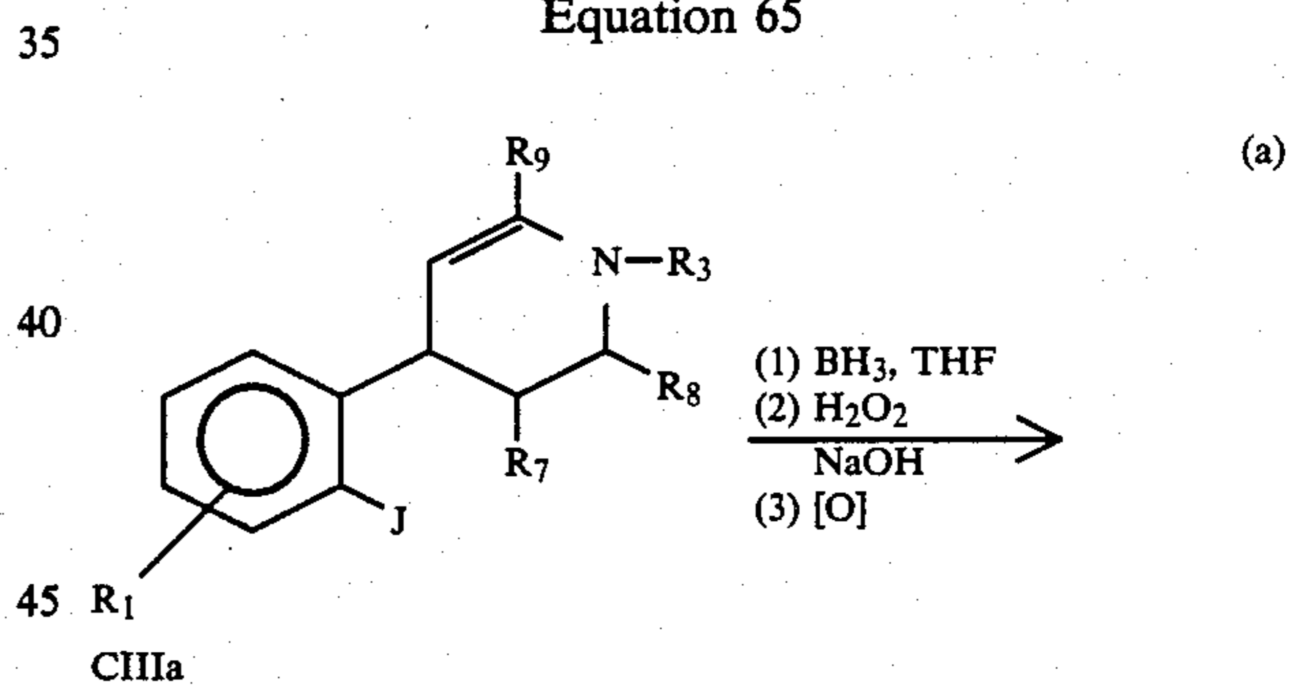
Equation 65
