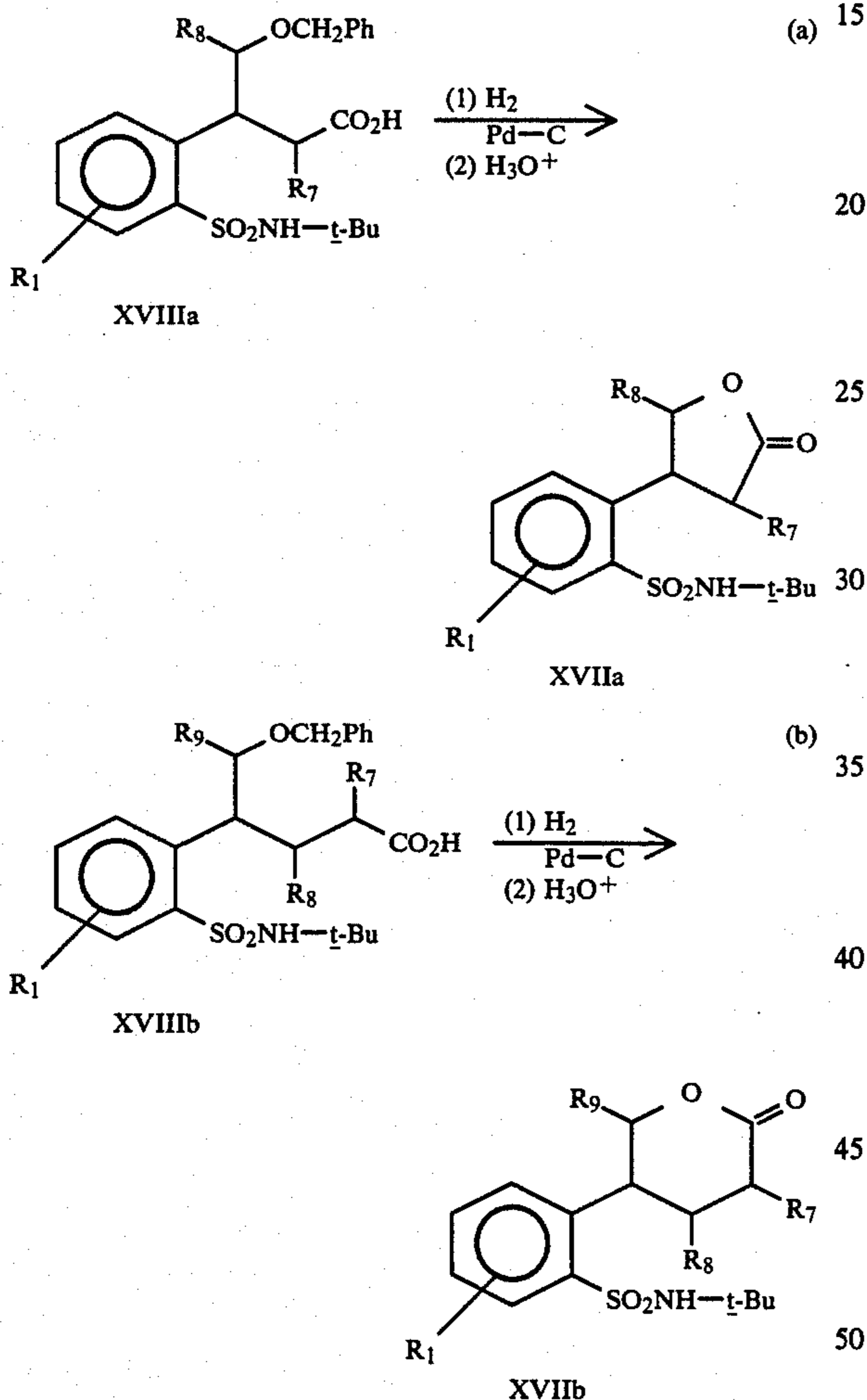
Equation 14
