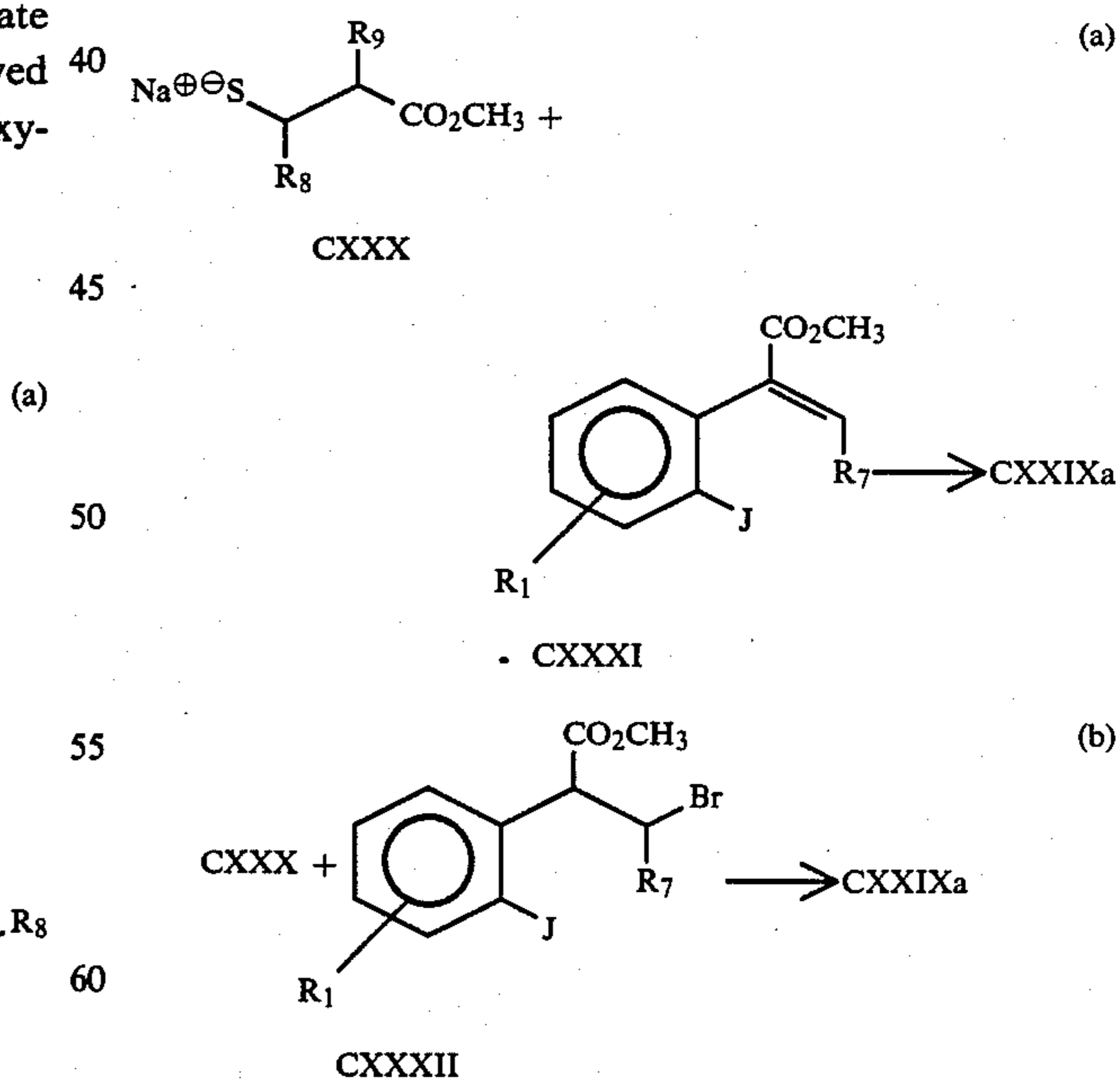
Equation 80
