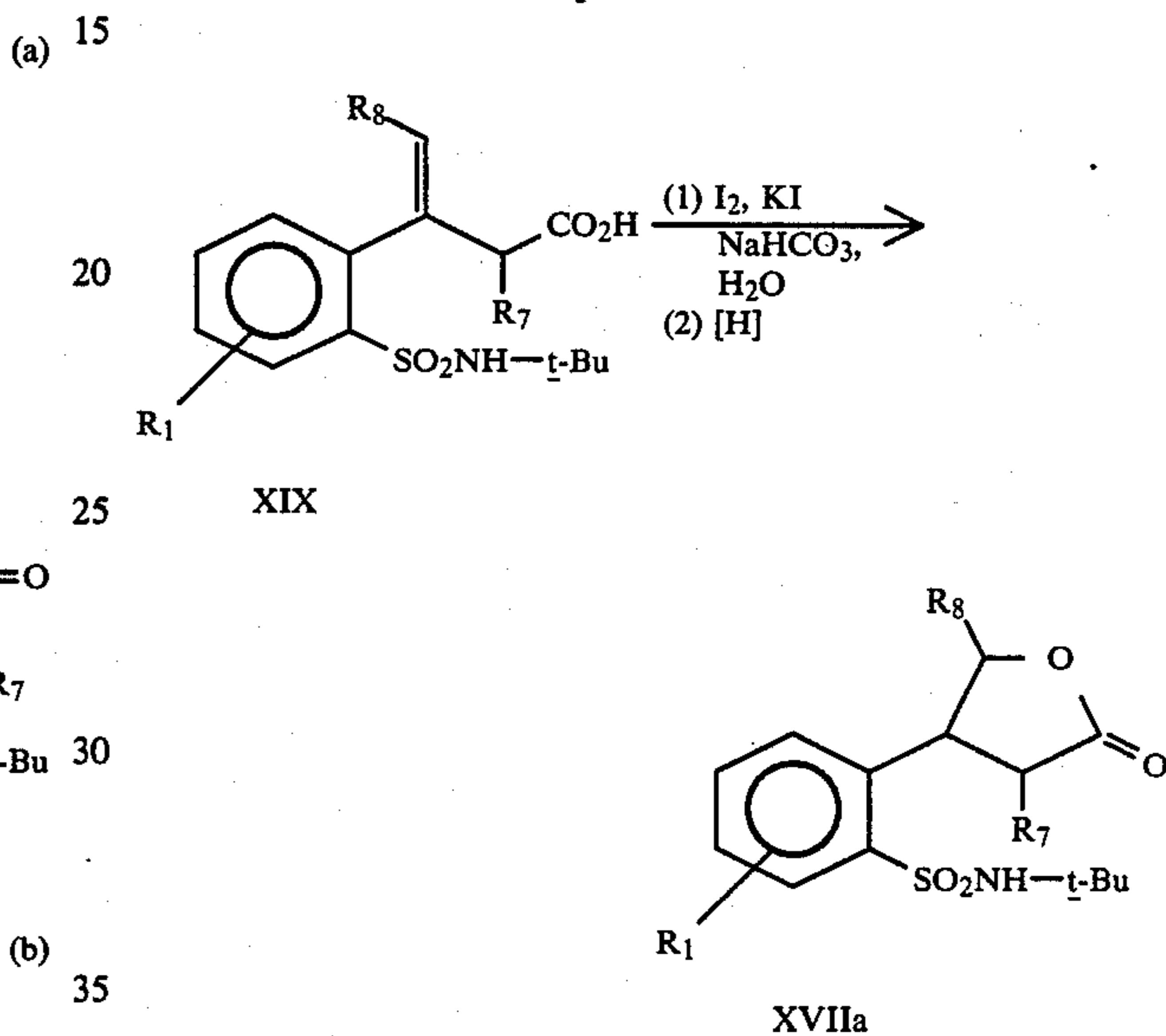
Equation 15
