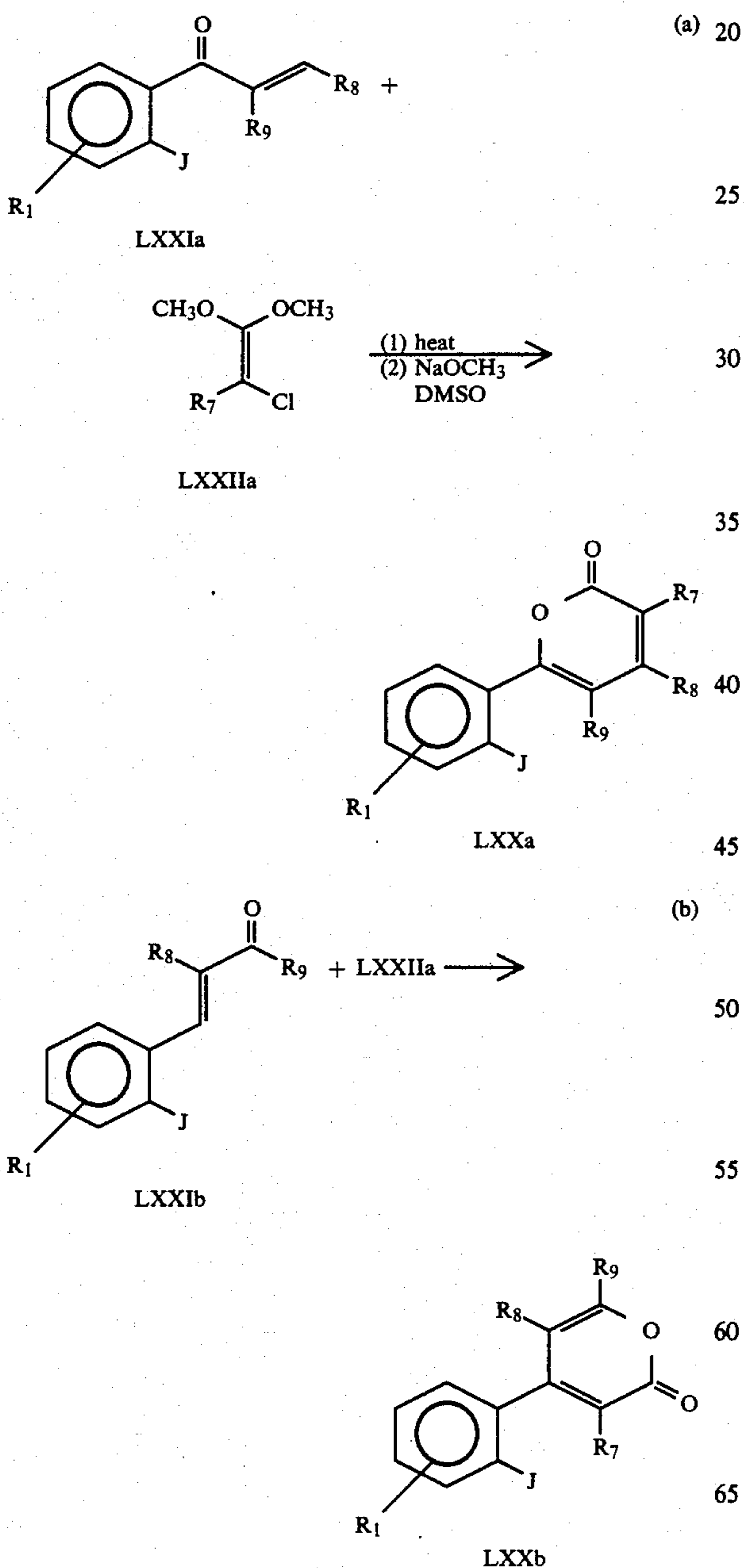
Equation 52
