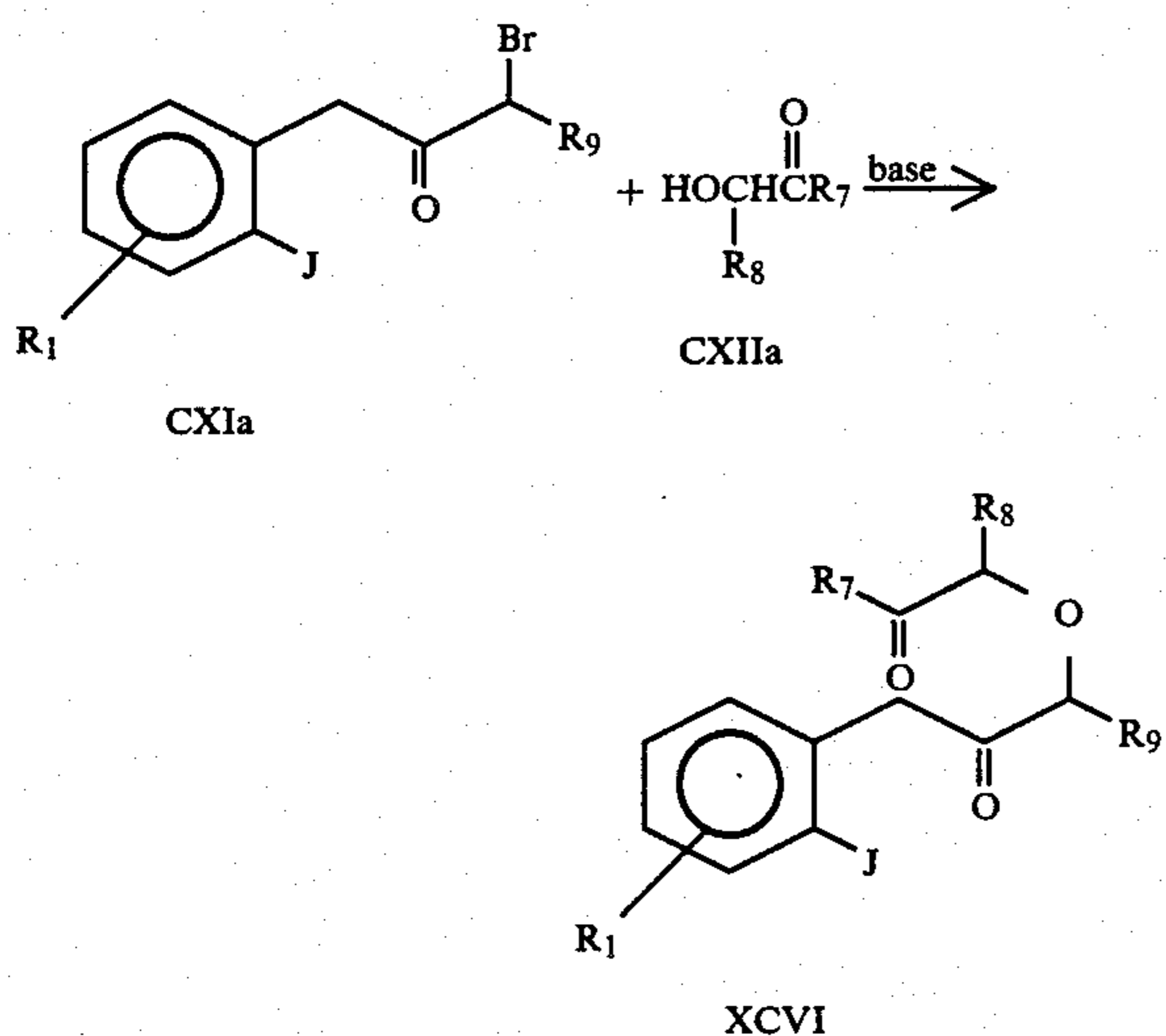
Equation 71
