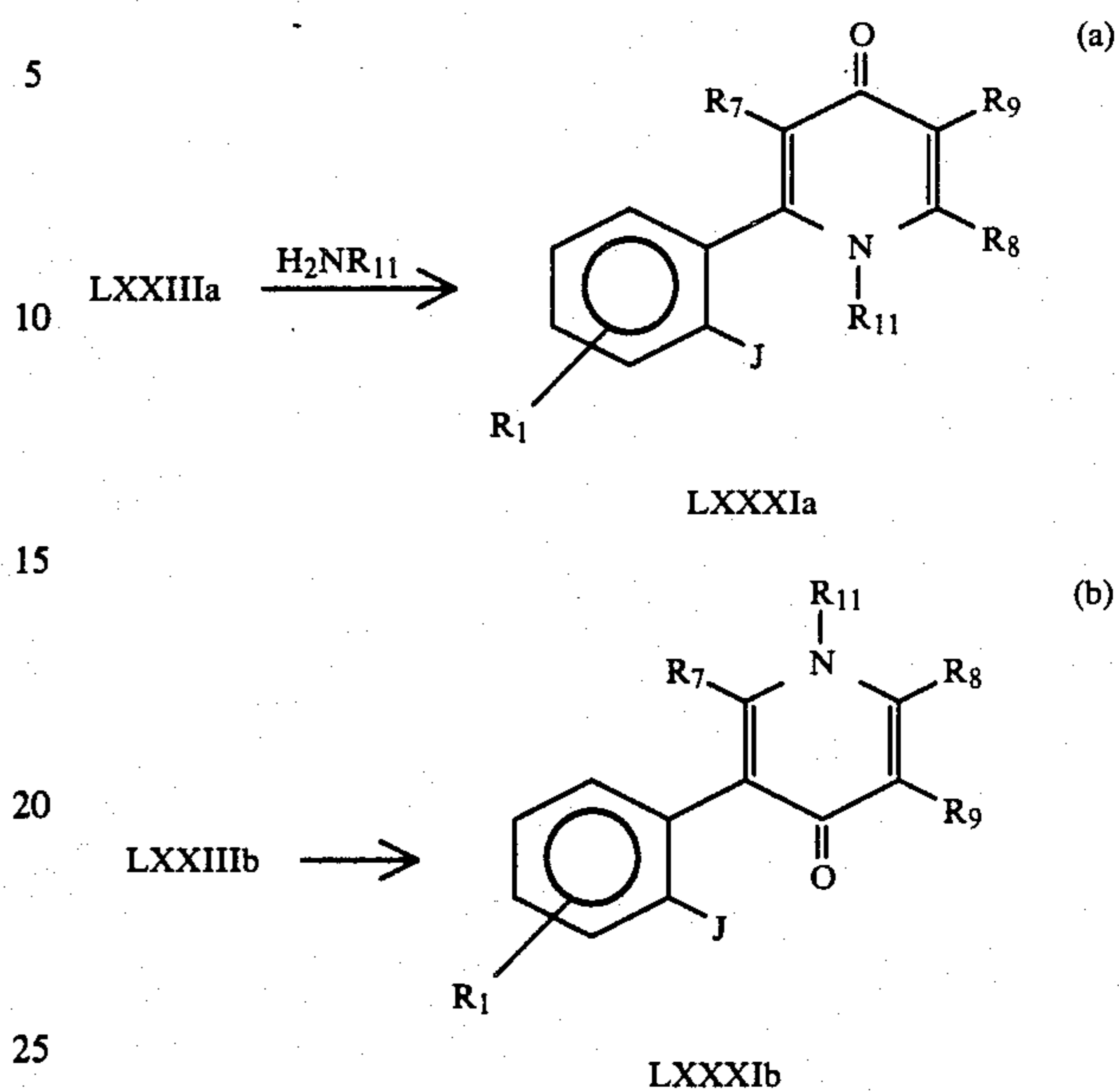
Equation 57
