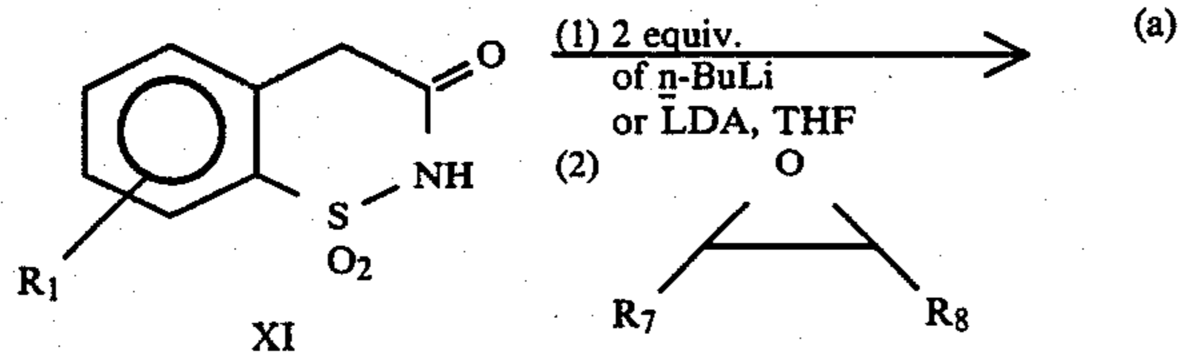
Equation 9
