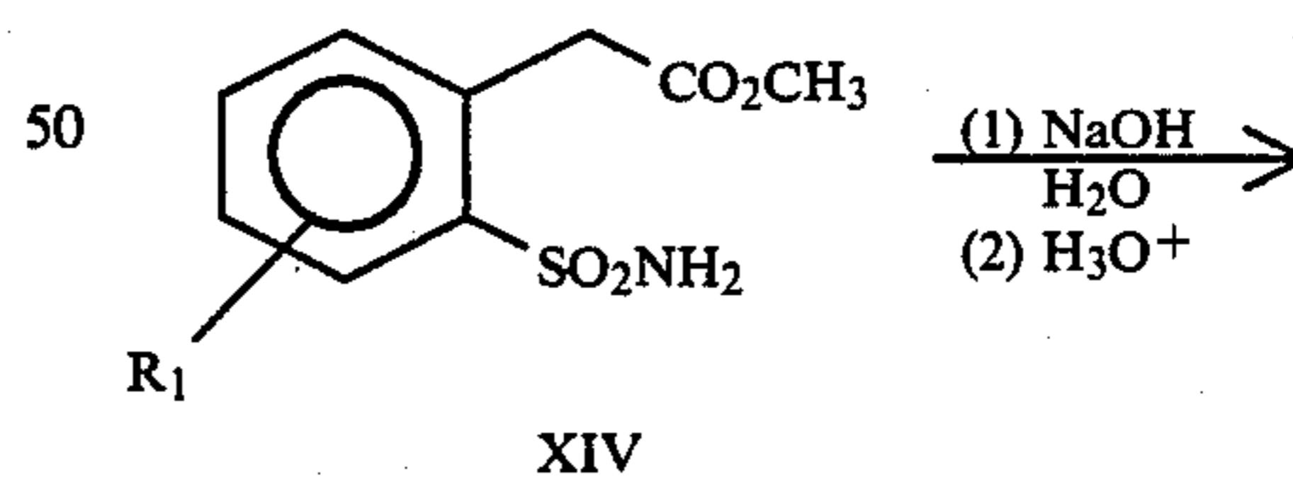
Equation 10
