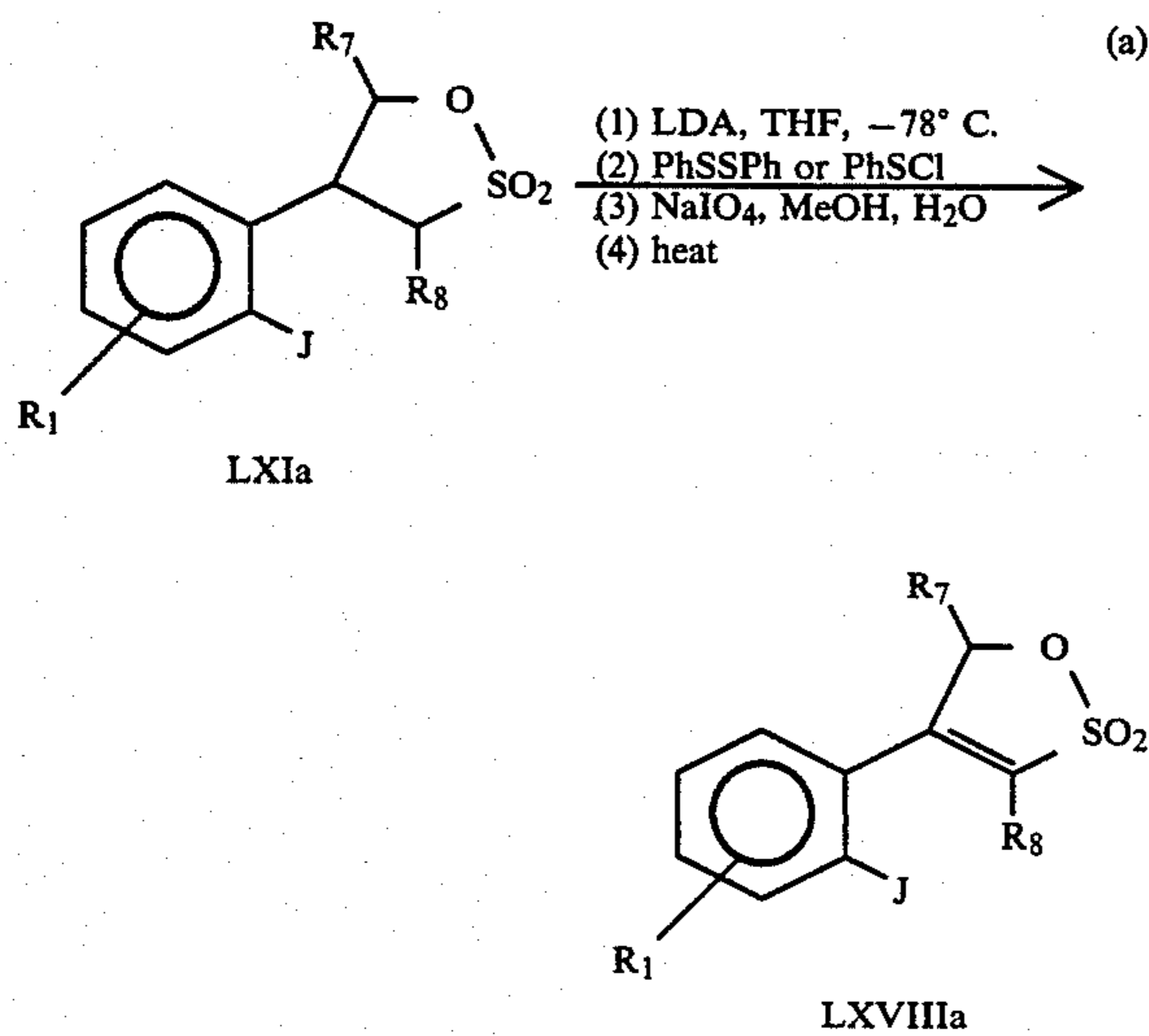
Equation 51
