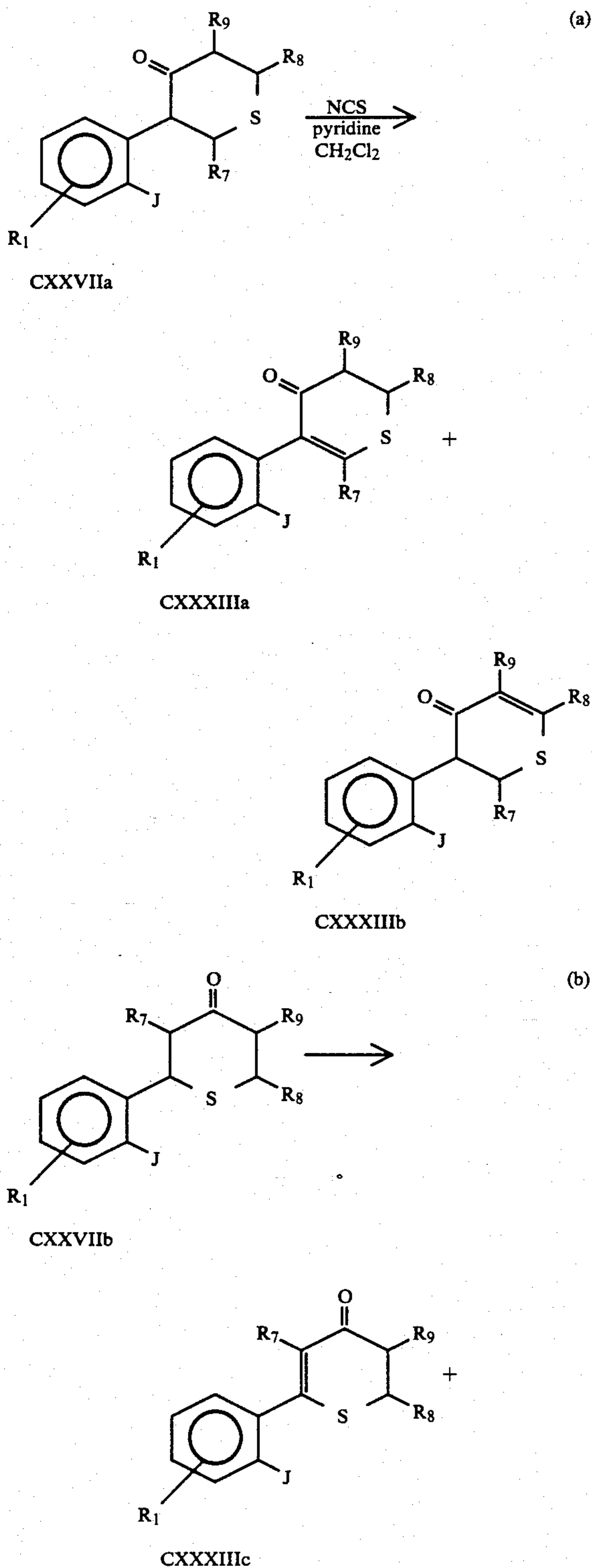
Equation 81
