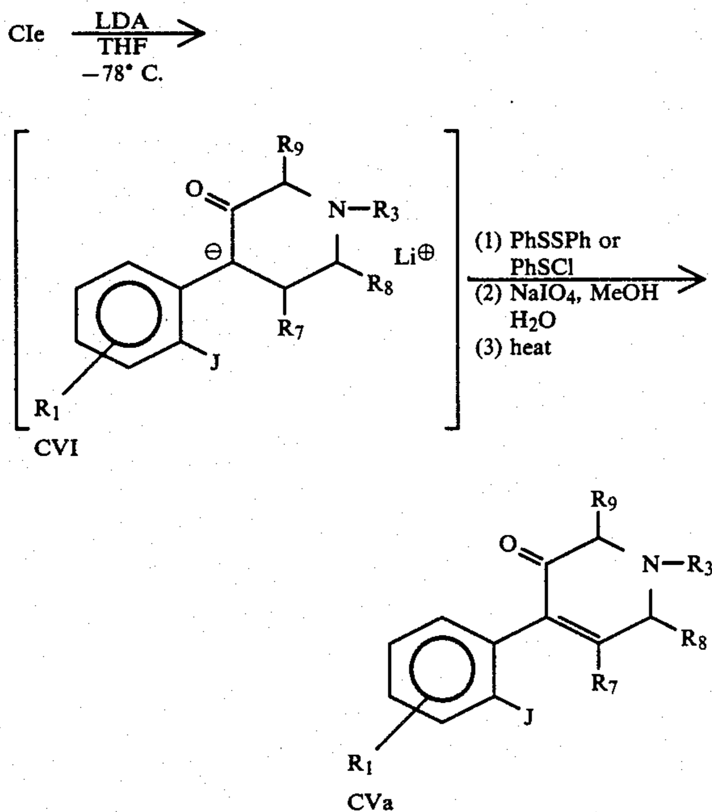
Equation 67
