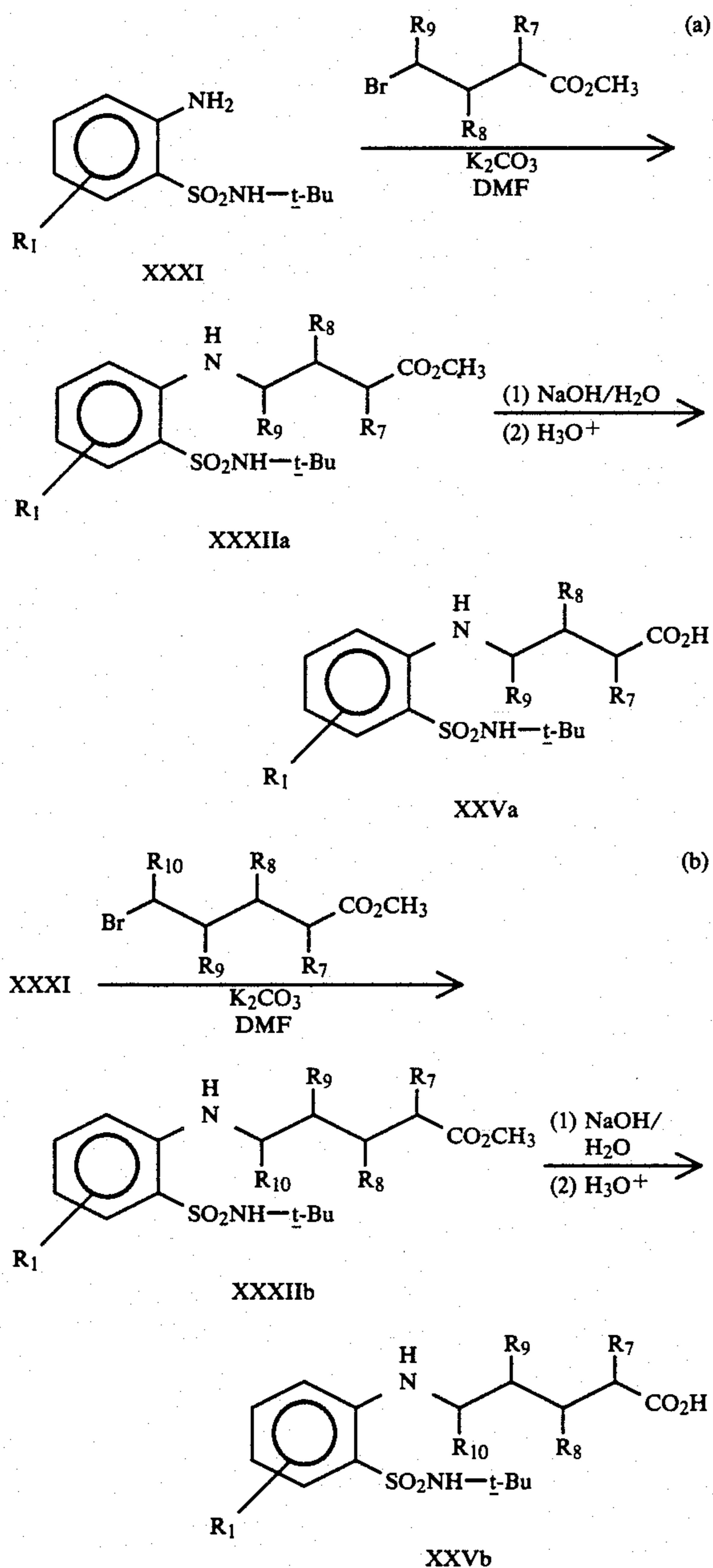
Equation 27
