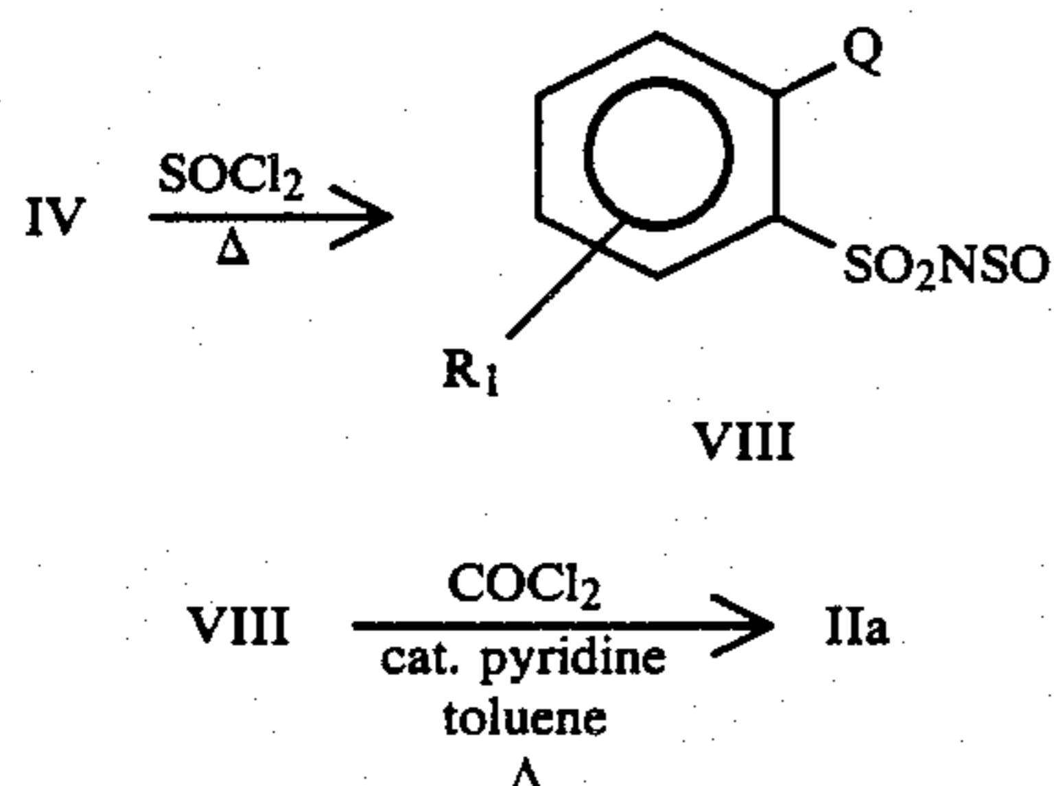
Equation 6
