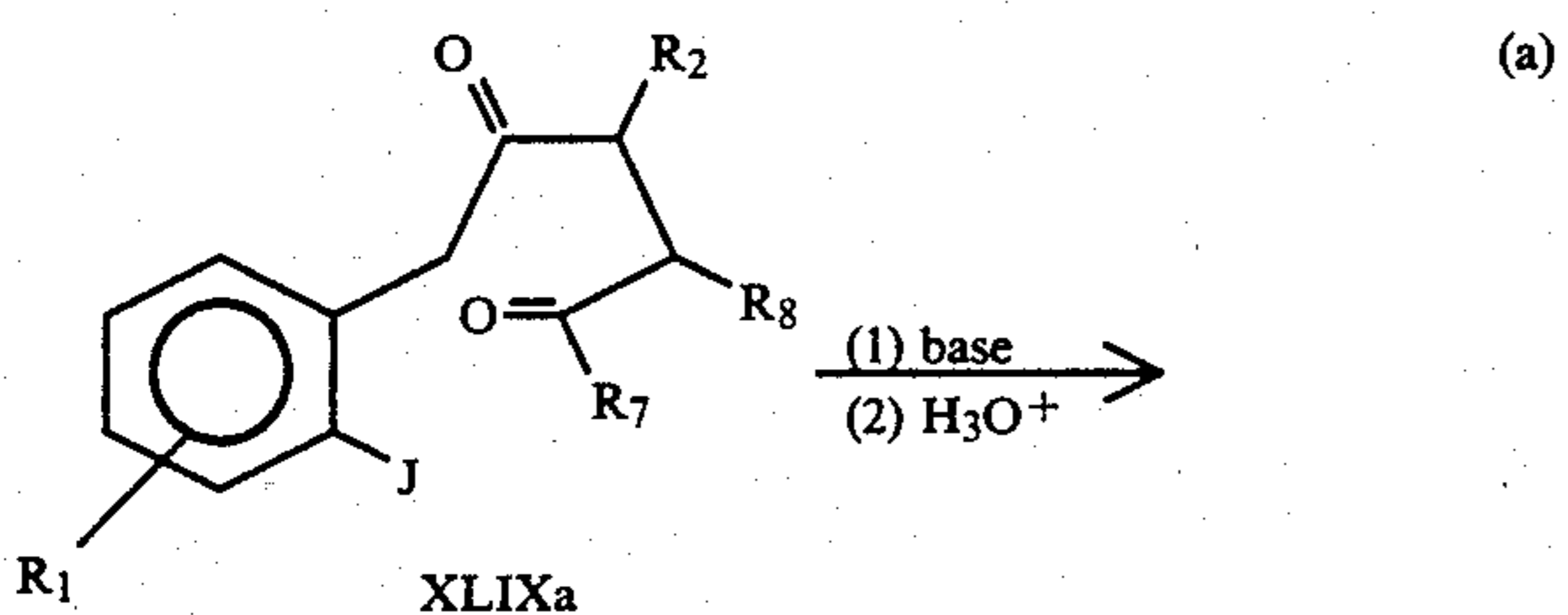
Equation 38
