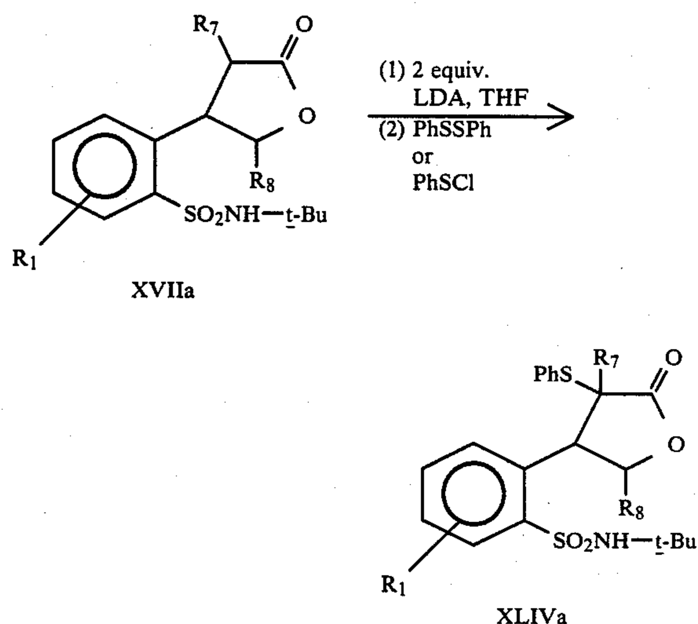
Equation 34
