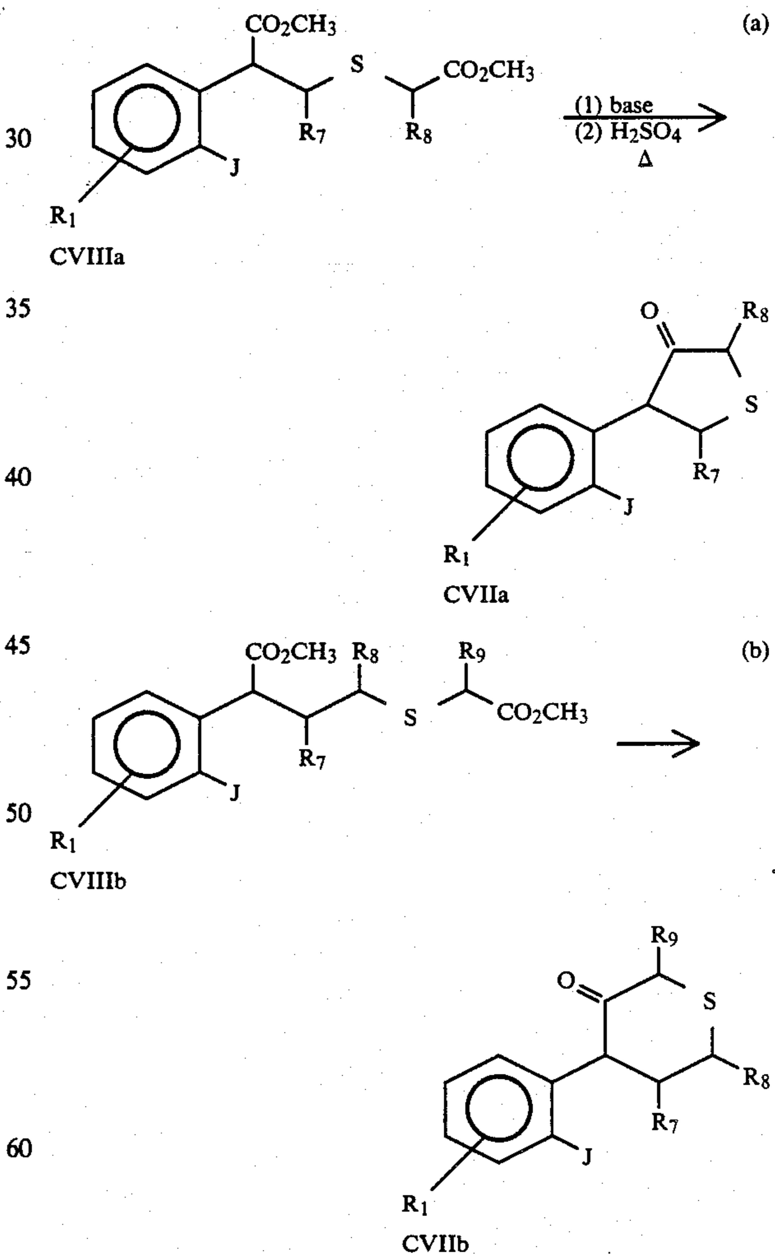
Equation 68
