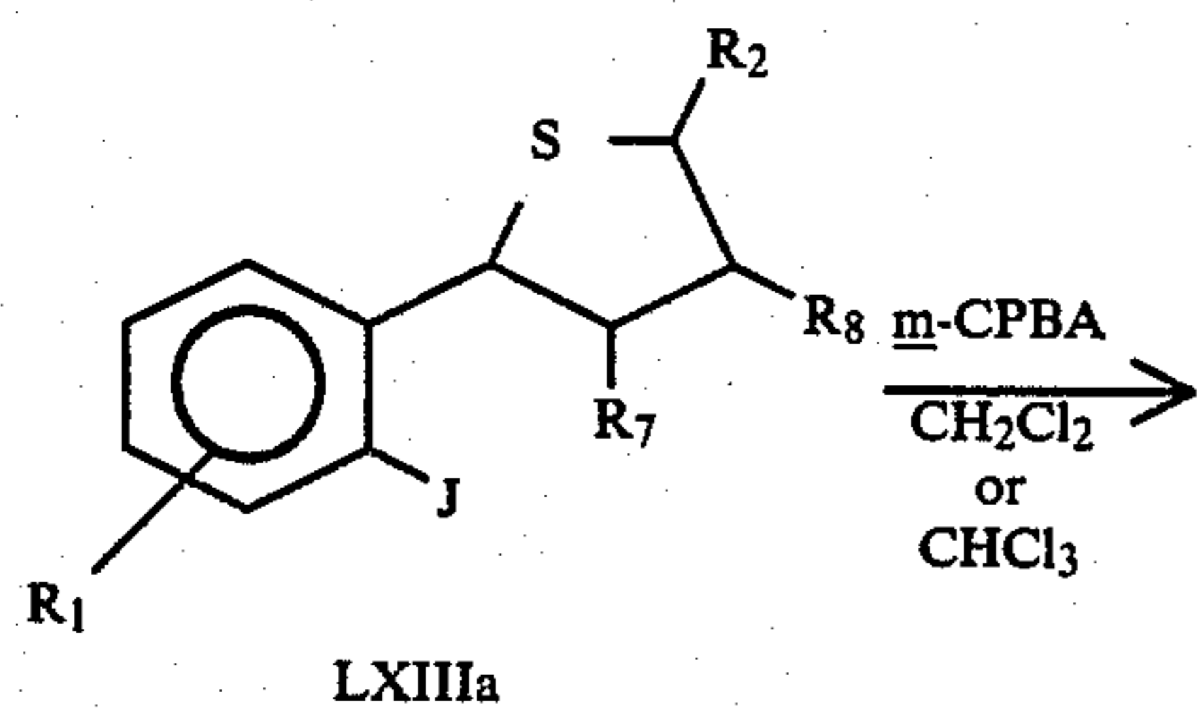
Equation 48
