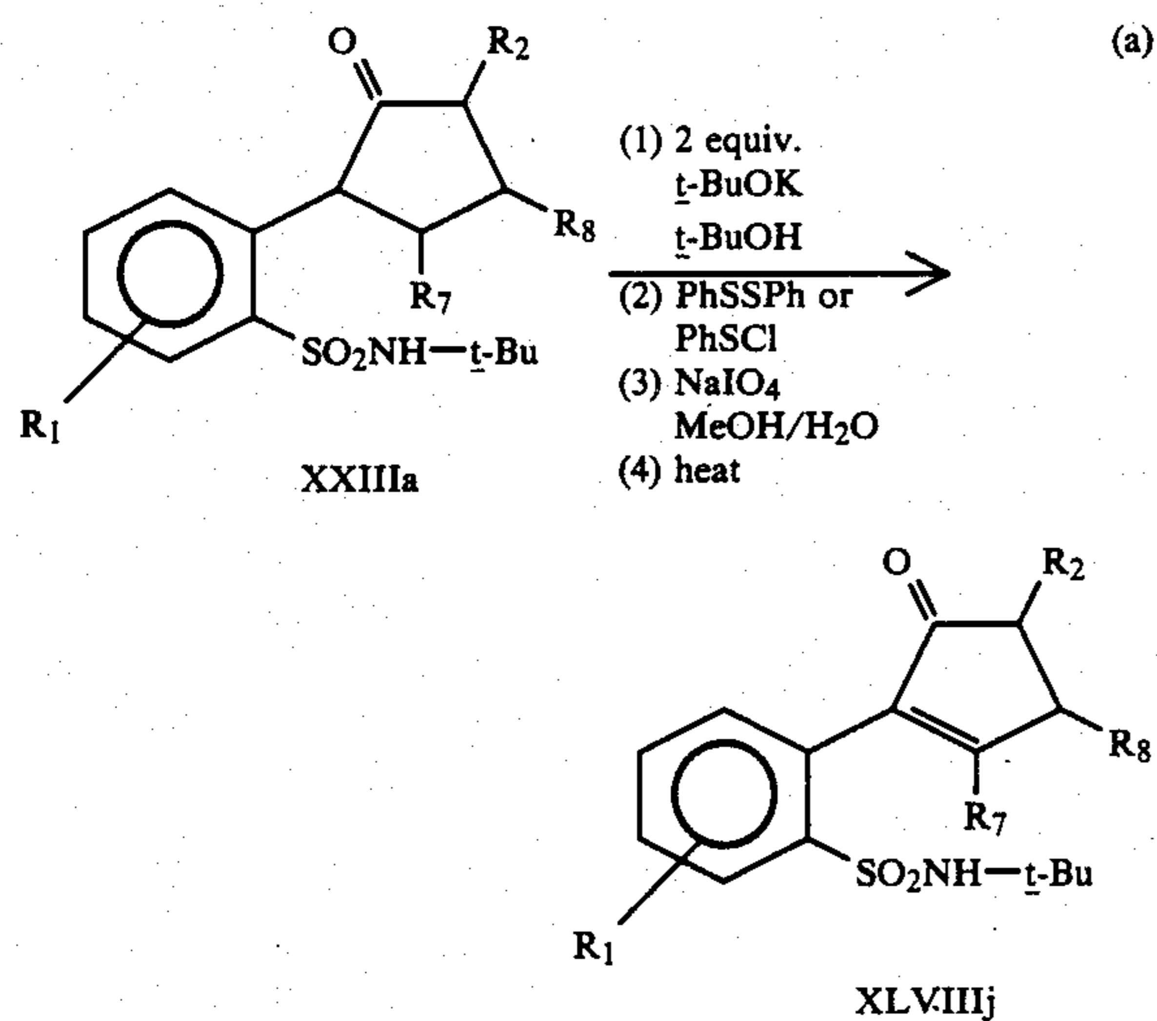
Equation 40
