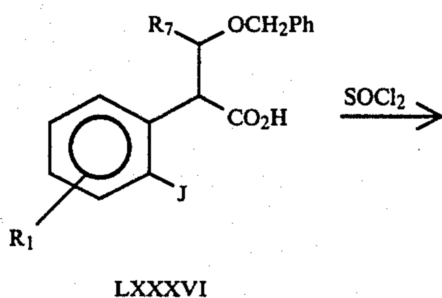
Equation 59
