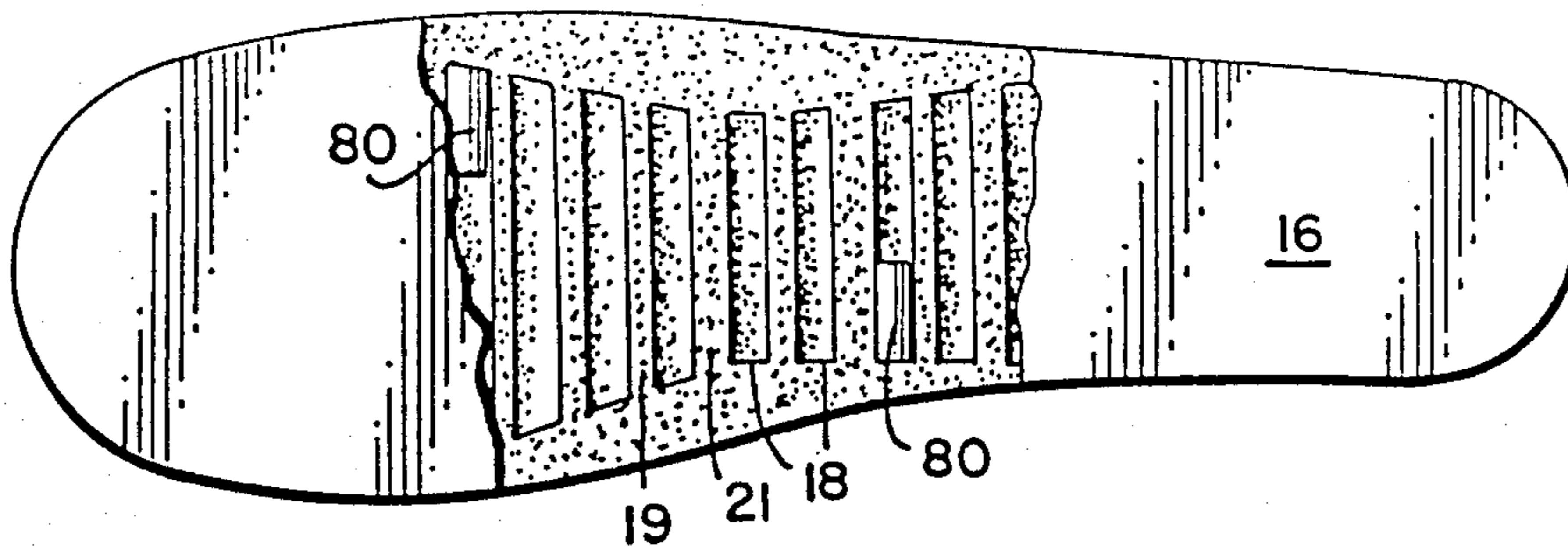
FIG. 13. (RELAXED STATE)
