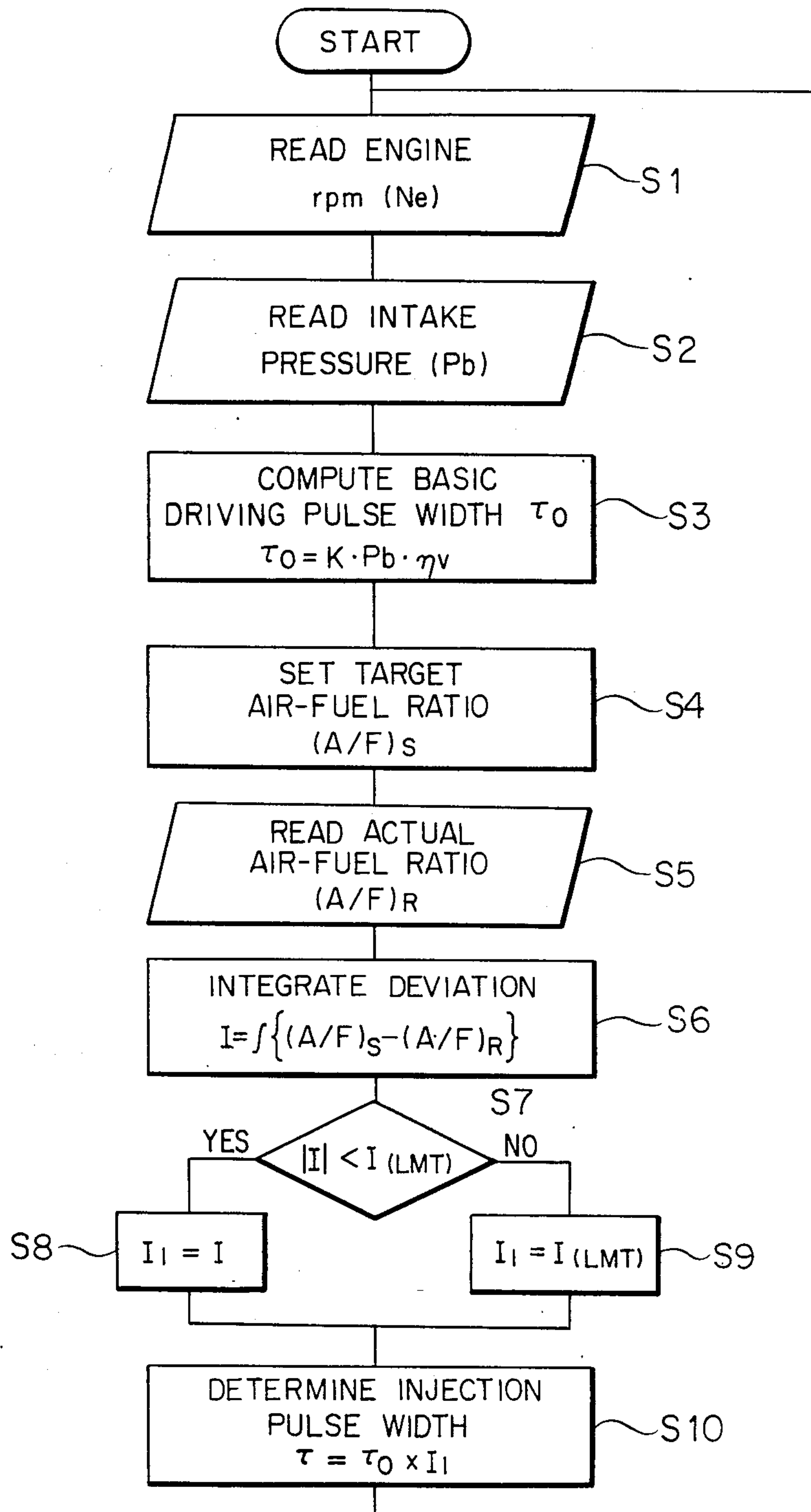
FIG. 6 PRIOR ART
