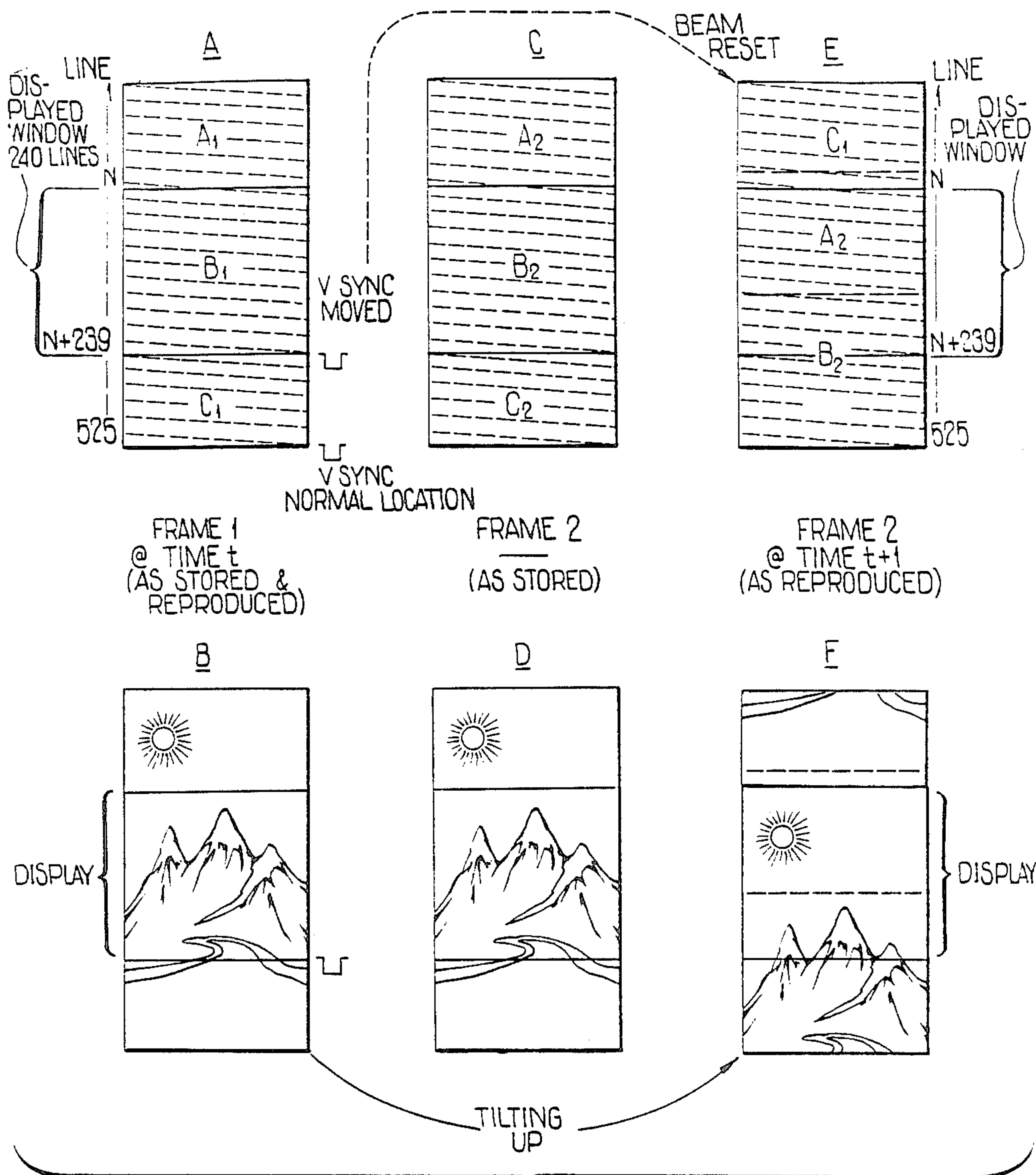
FIG 10 VERTICAL WINDOWING
