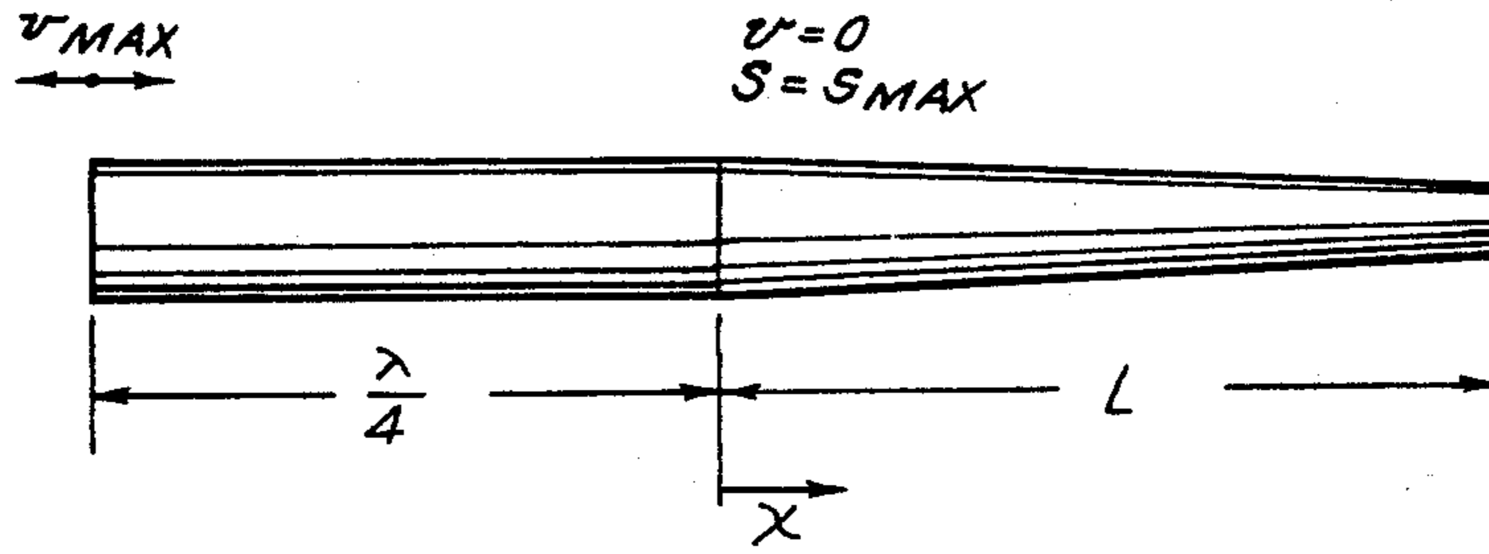
FIG. 1 HIGH VELOCITY ULTRASONIC EXTENSIONAL RESONATOR
