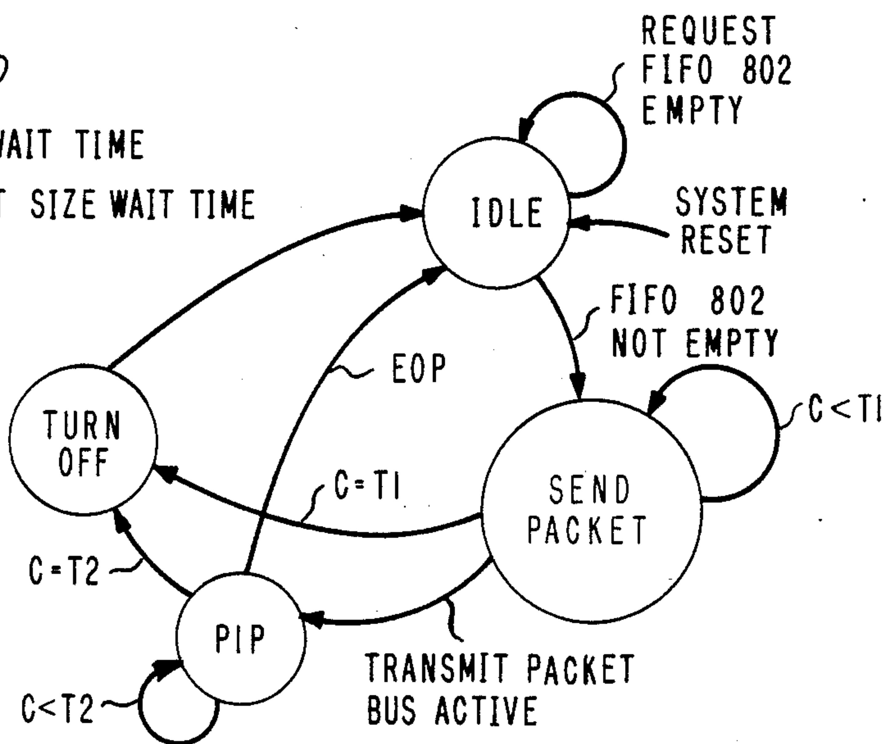
OUTPUT CONTROLLER 803
