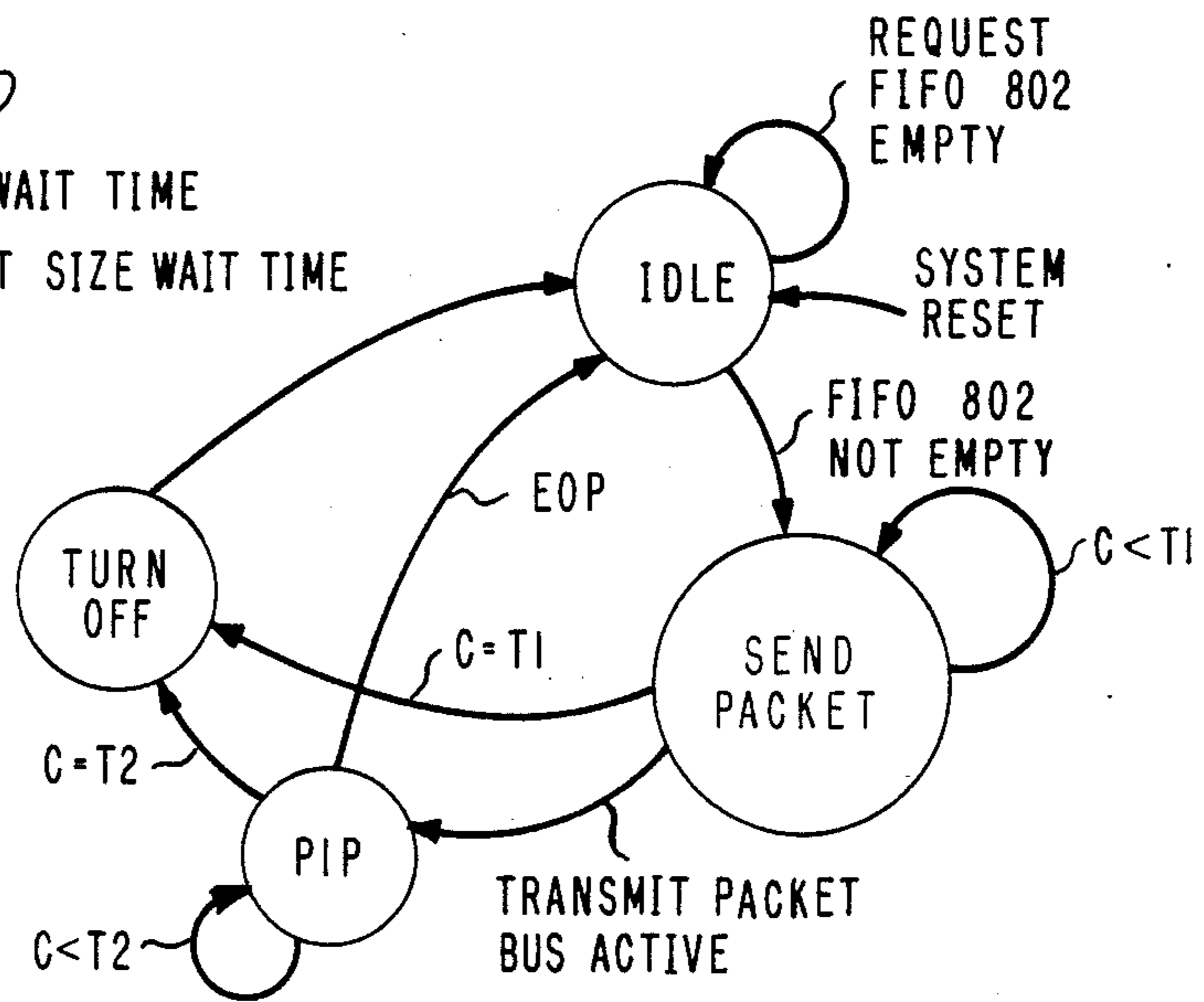
OUTPUT CONTROLLER 803
