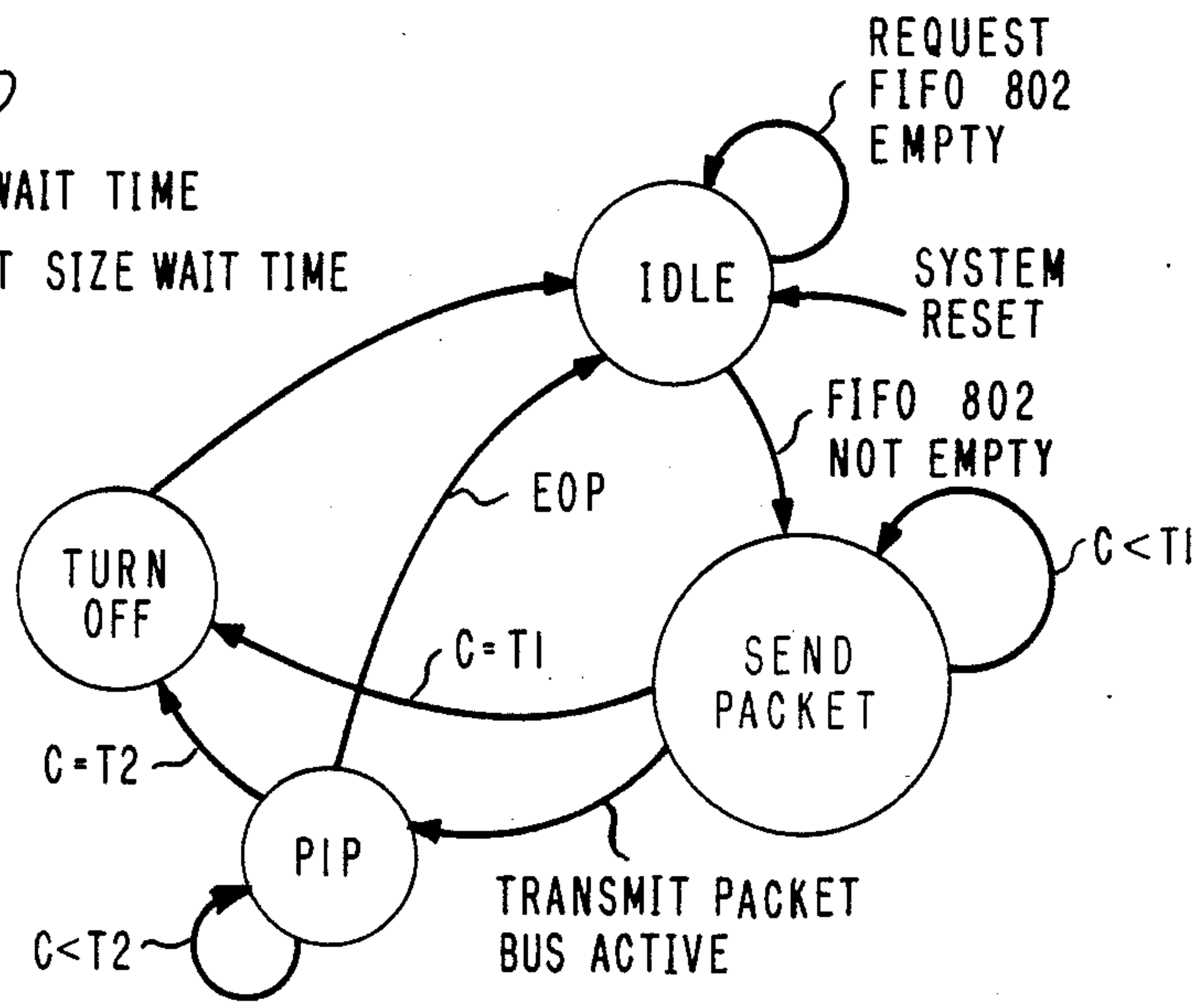
OUTPUT CONTROLLER 803
