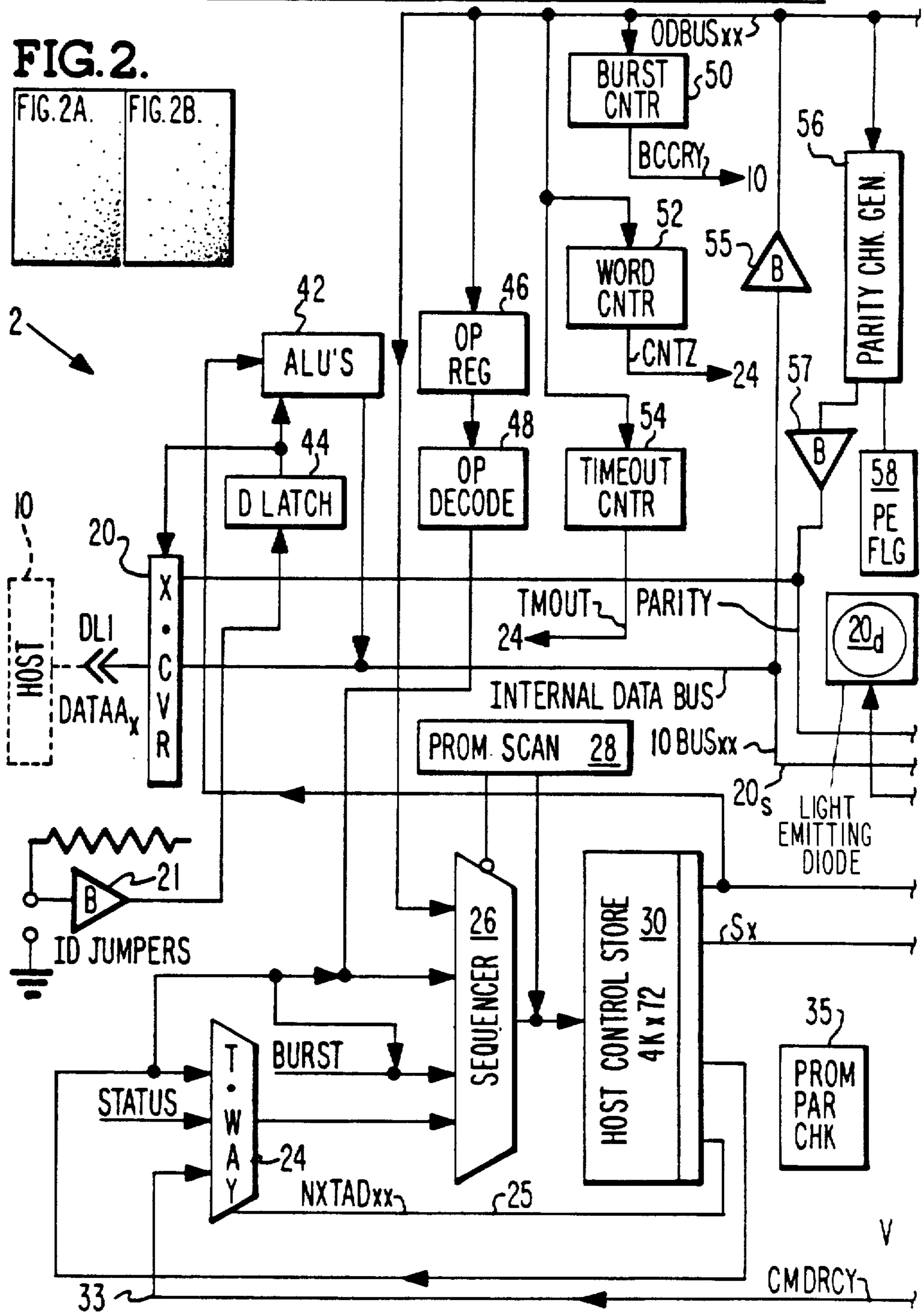
FIG. 2A. Host Adapter Basic Block Diagram.
