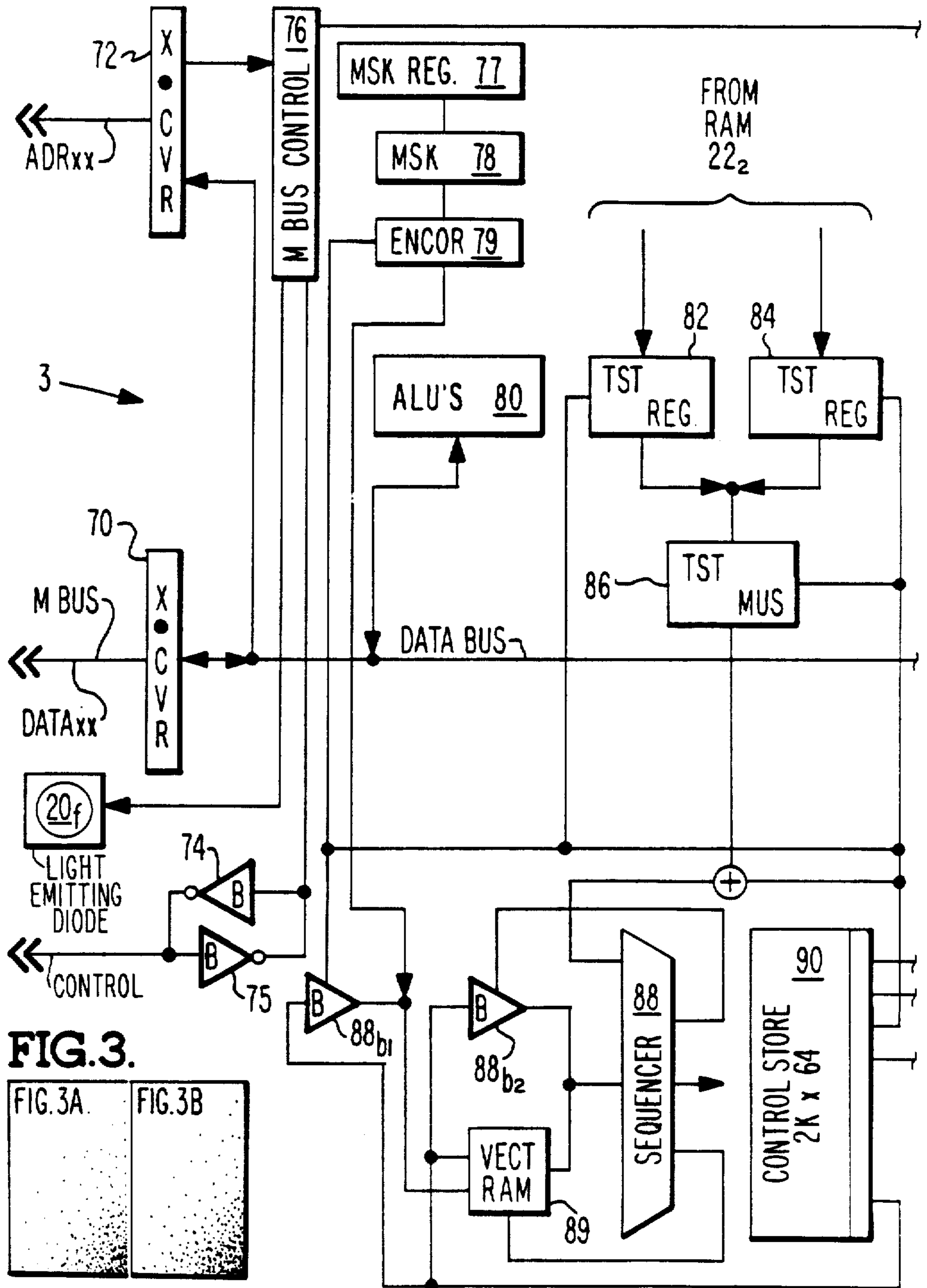
FIG.3A. Formatter Card Basic Block Diagram.
