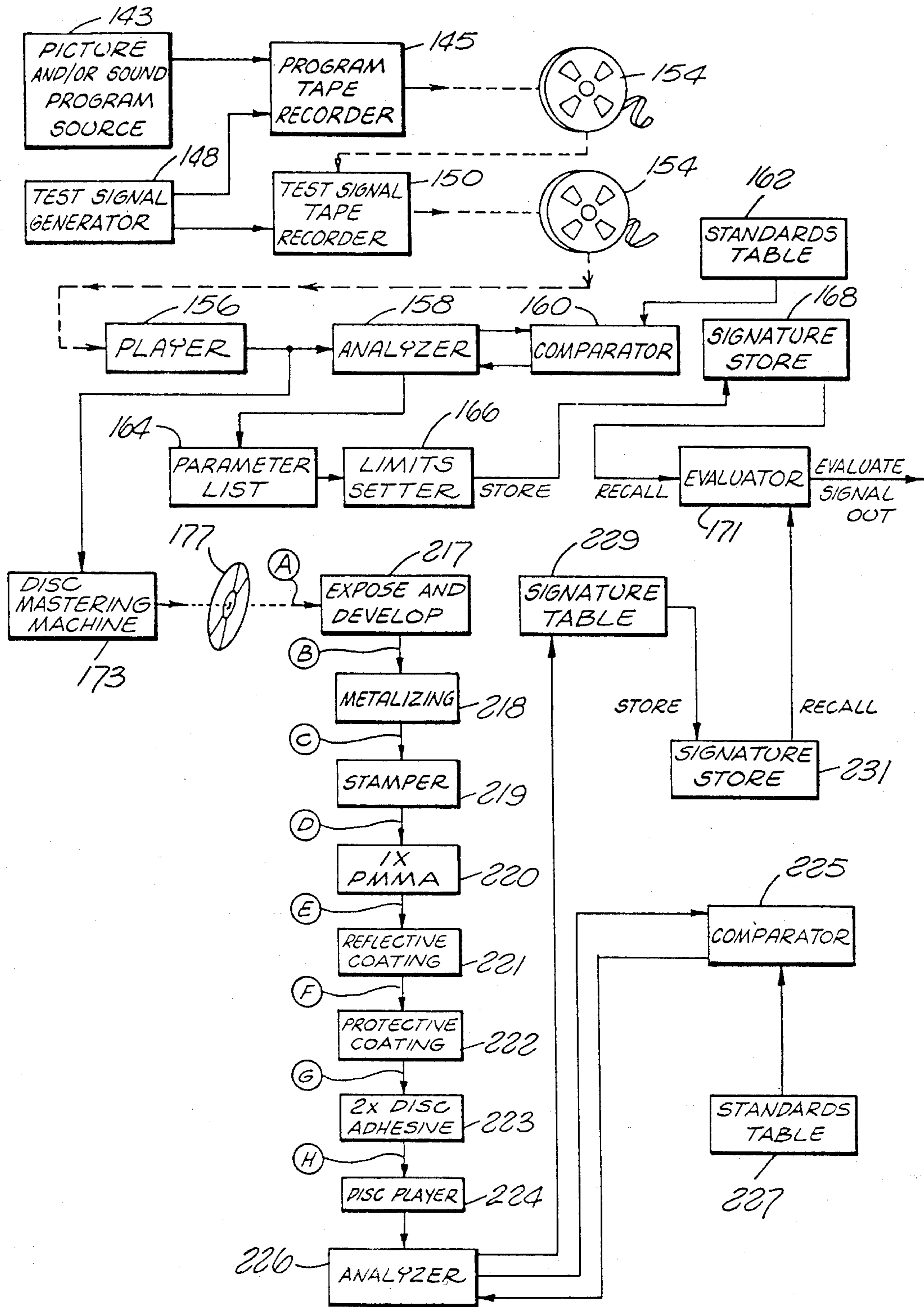
FIG. 25 DISC EVALUATION
