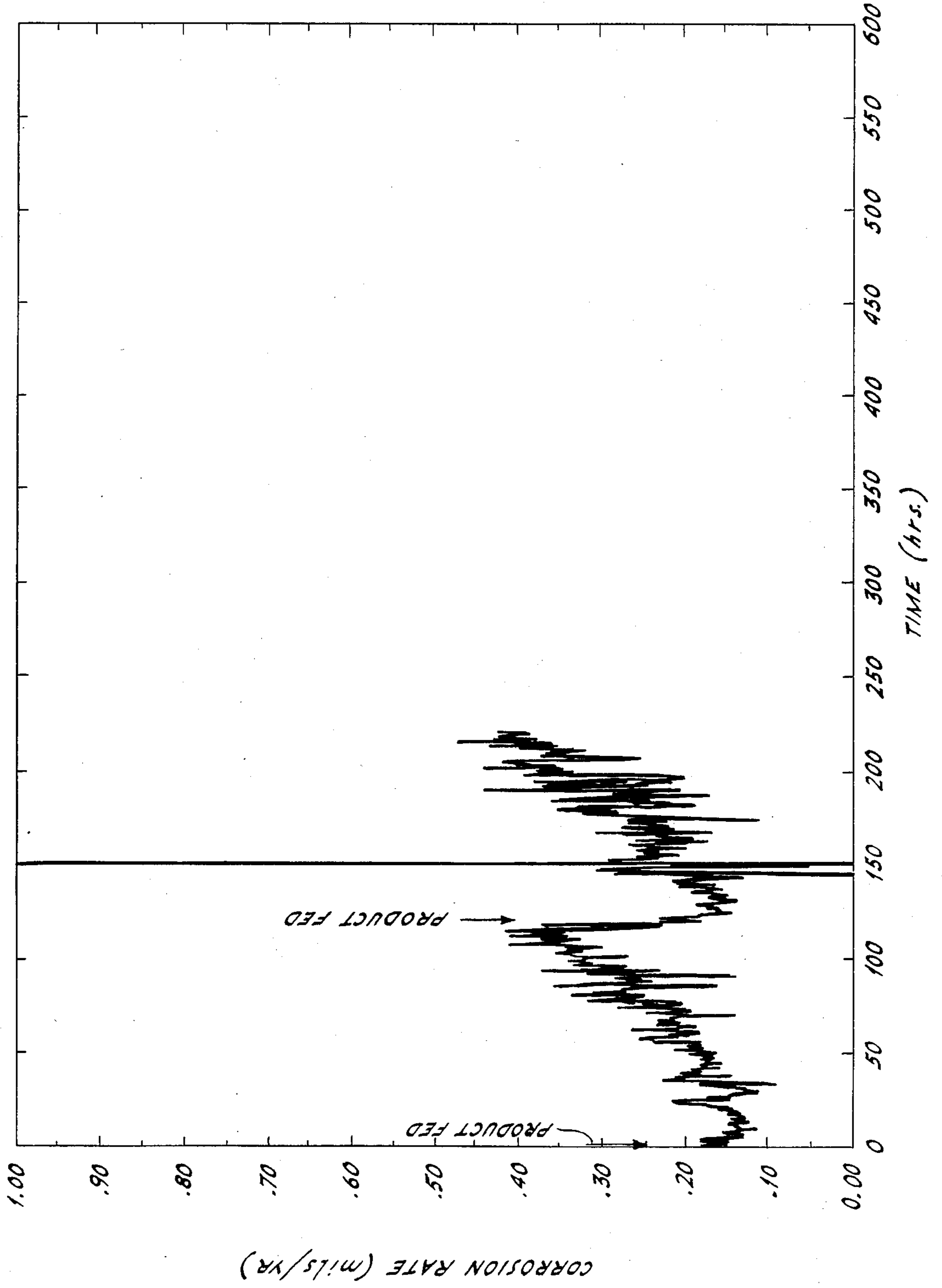
FIG. 1. CORROSION RATE vs TIME TOLYLTRIAZOLE TREATMENT
