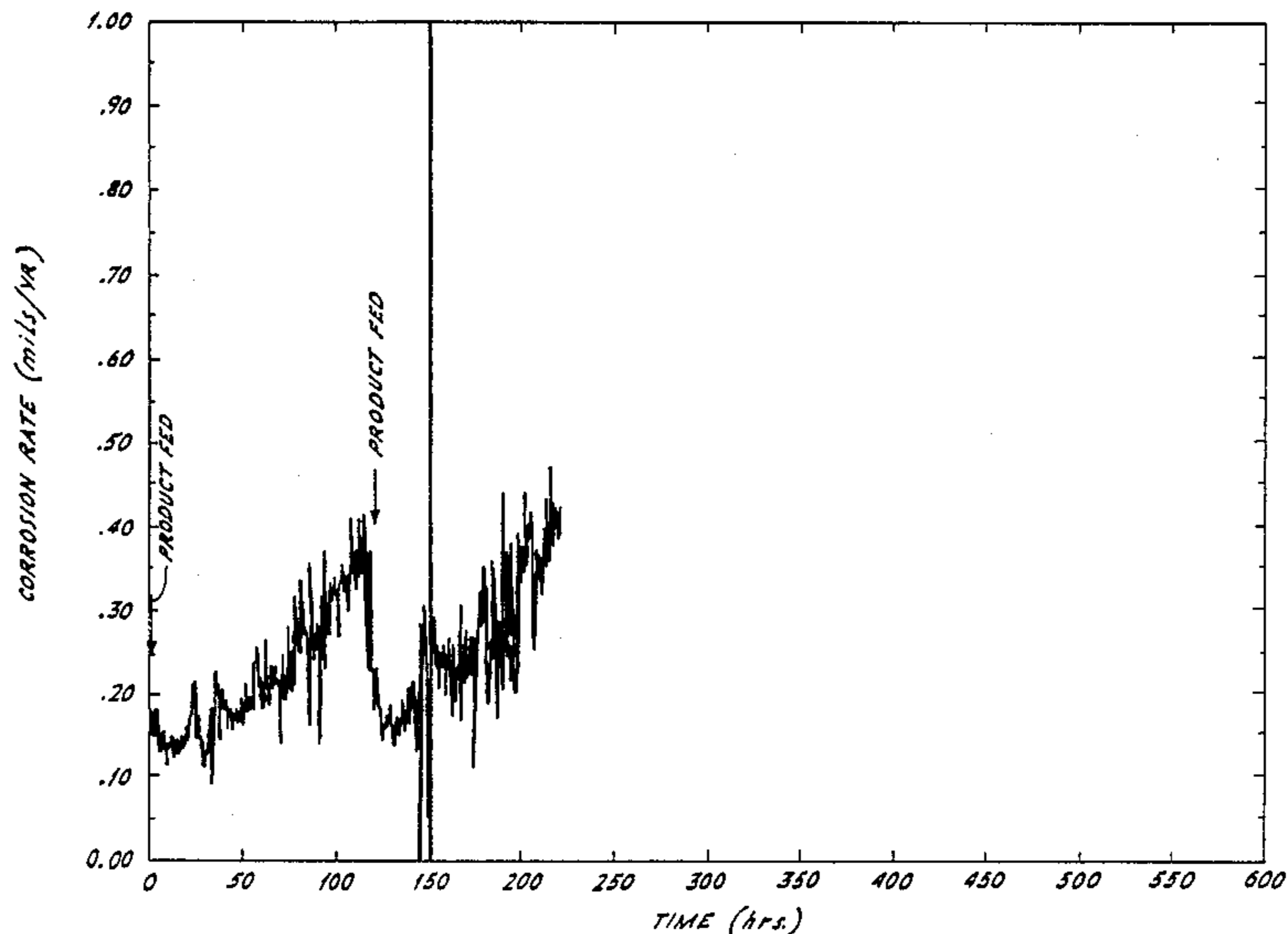
CORROSION RATE vs TIME TOLYLTRIAZOLE TREATMENT
