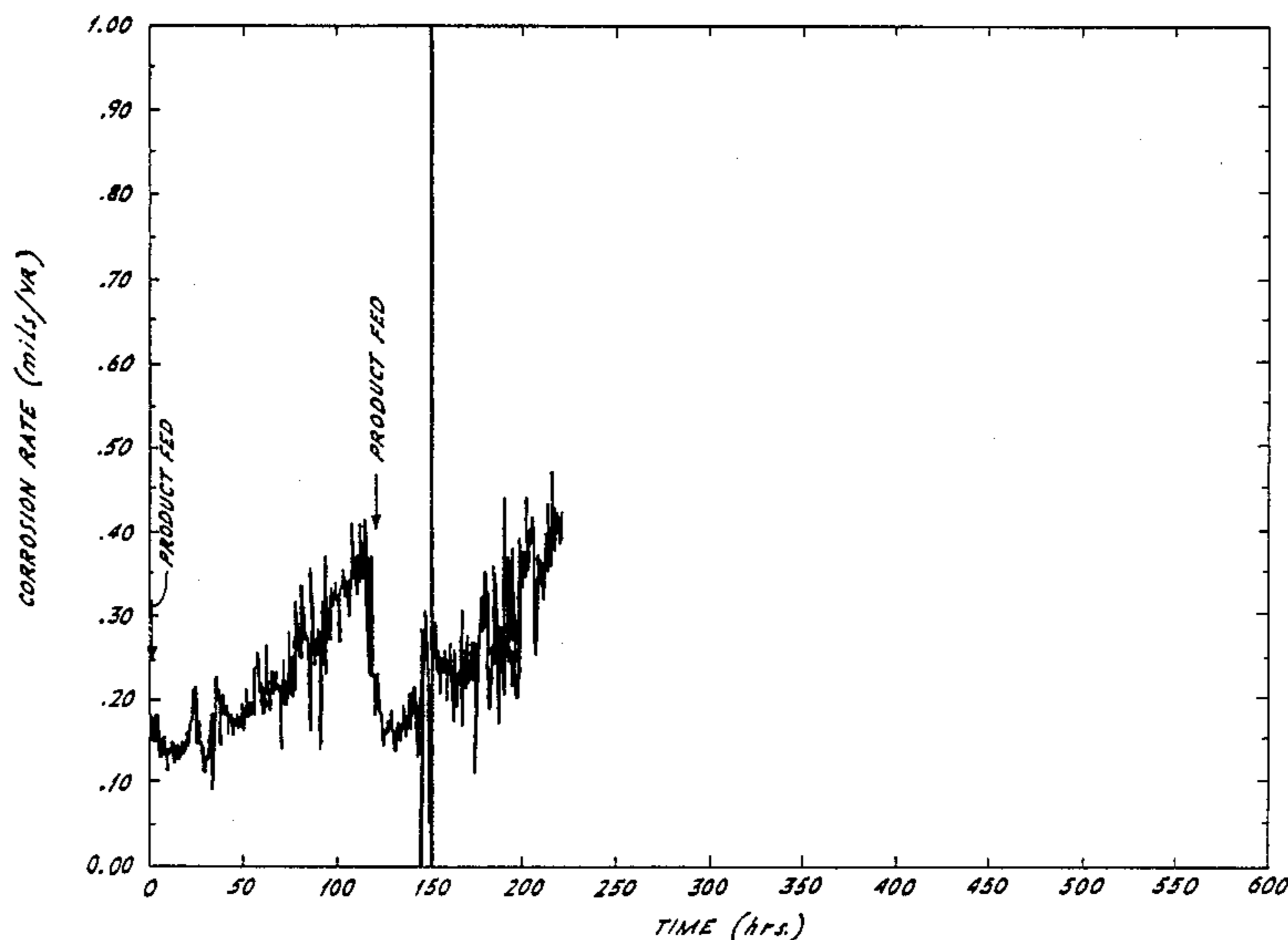
CORROSION RATE vs TIME TOLYLTRIAZOLE TREATMENT
