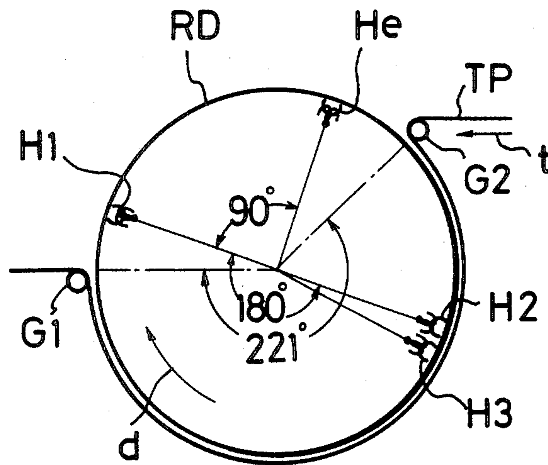
FIG. 1 (PRIOR ART)
