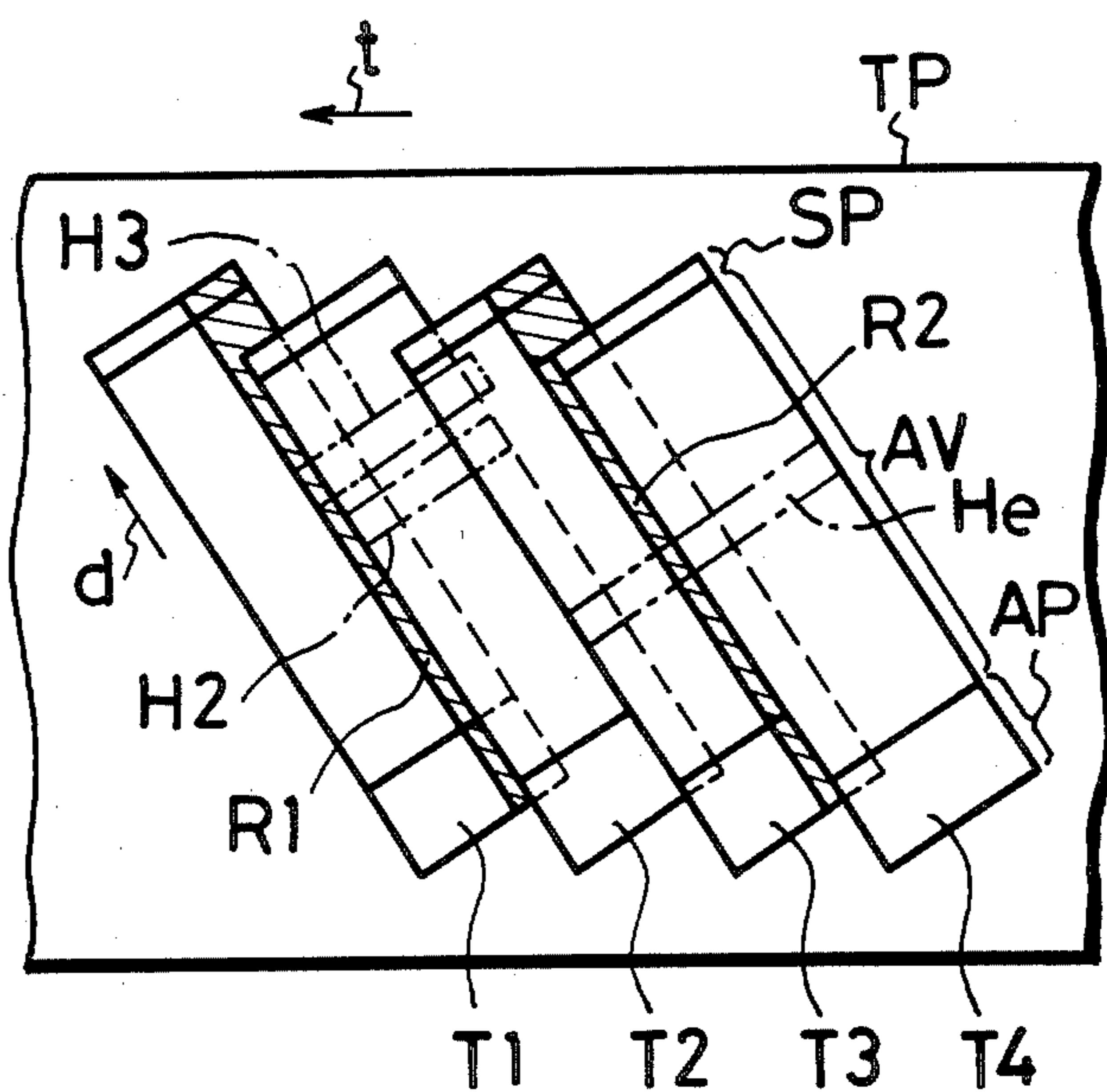
FIG. 6 (PRIOR ART)
