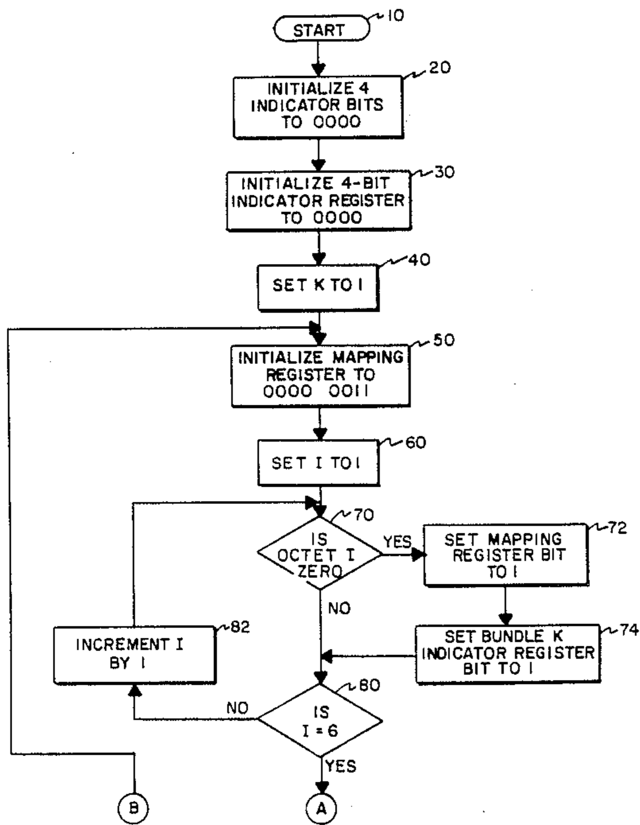
T1 LINE FORMAT FOR CCITT 32 KBPS ADPCM AND 64 KBPS CLEAR CHANNEL TRANSMISSION FRAME/BUNDLE ENCODE LOGIC
