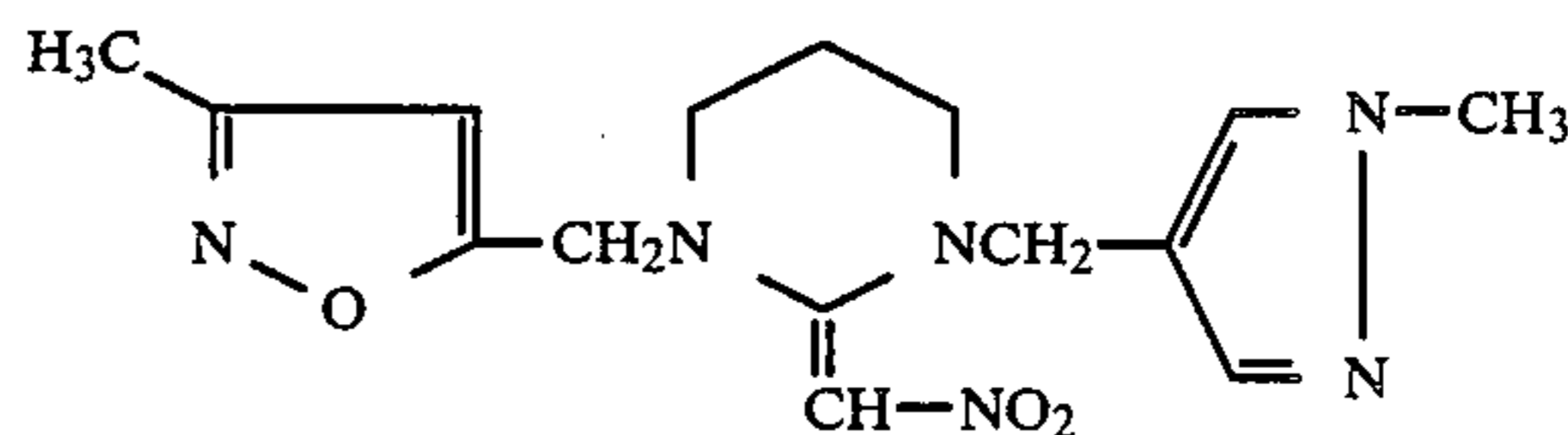
(Compound No. 16)
