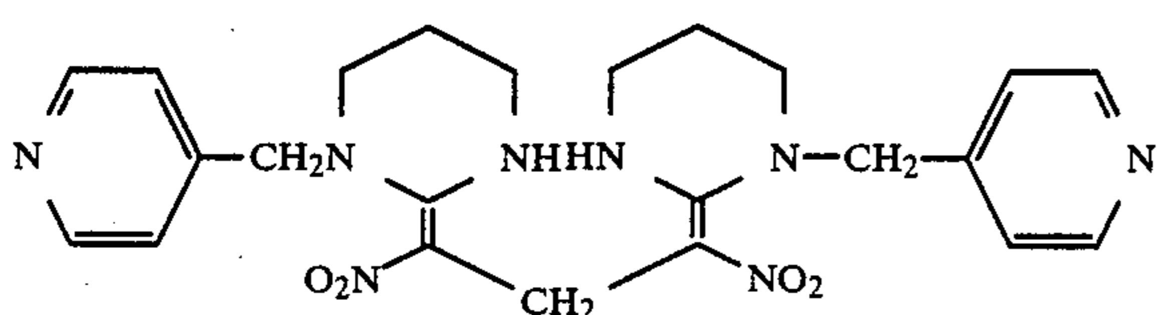
(Compound No. 25)
