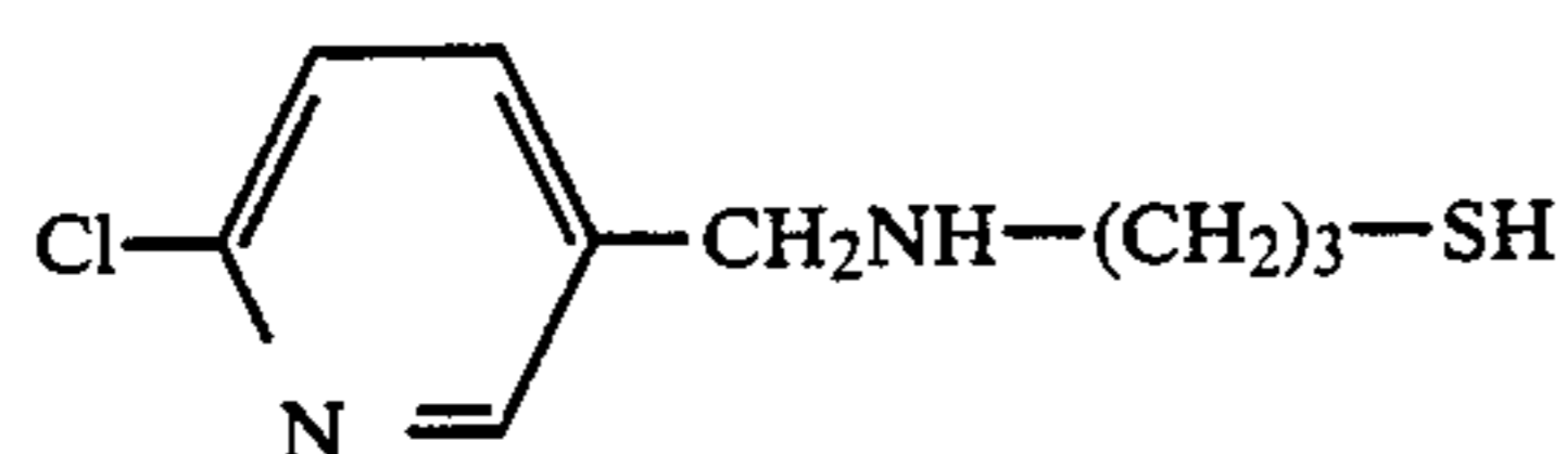
N-(2-chloro-5-pyridylmethyl)3-aminopropanethiol ( n_D^{22} : 1.5890)
