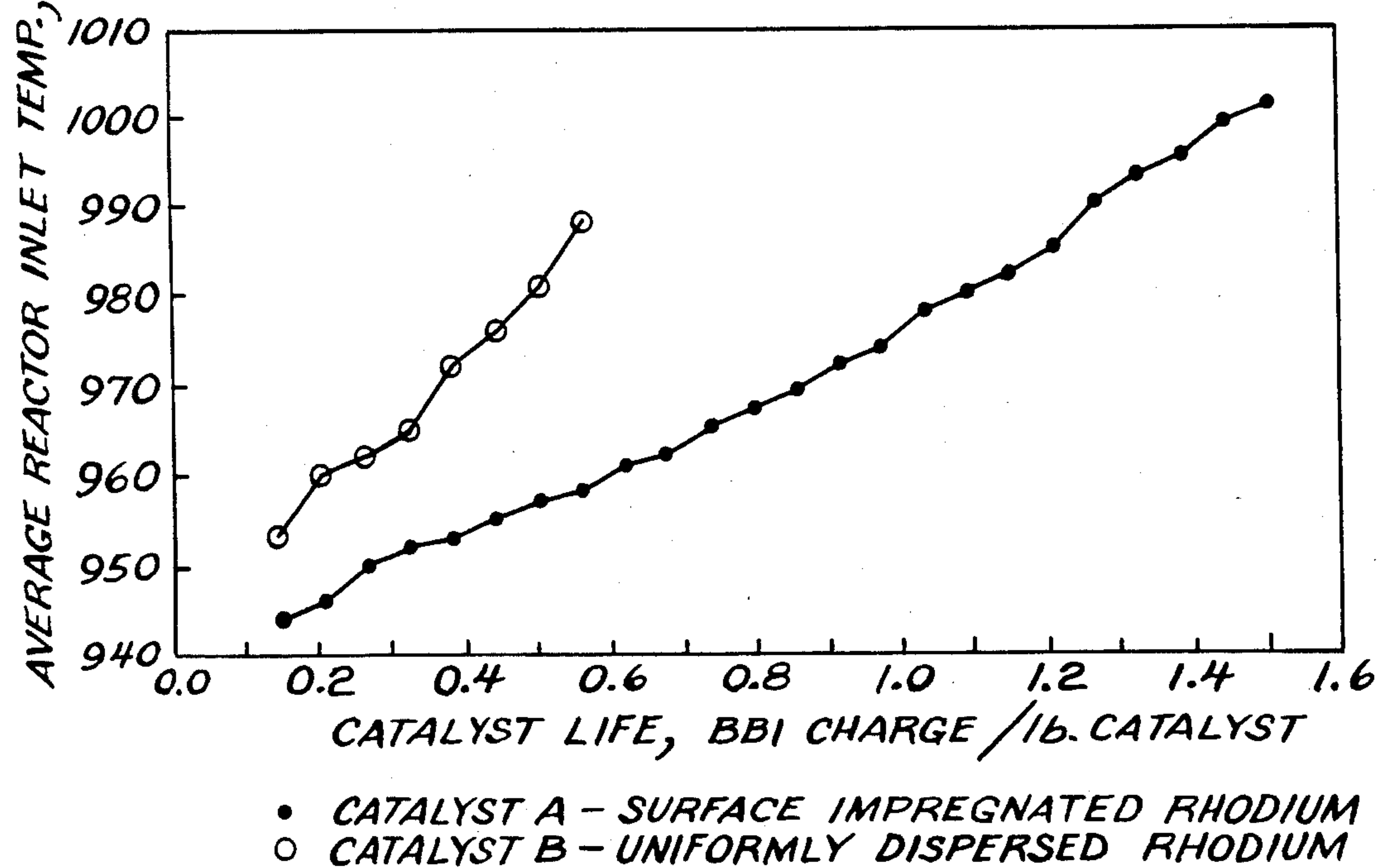
FIG. 4 AVE. REACTOR INLET TEMP. VS CATALYST LIFE
