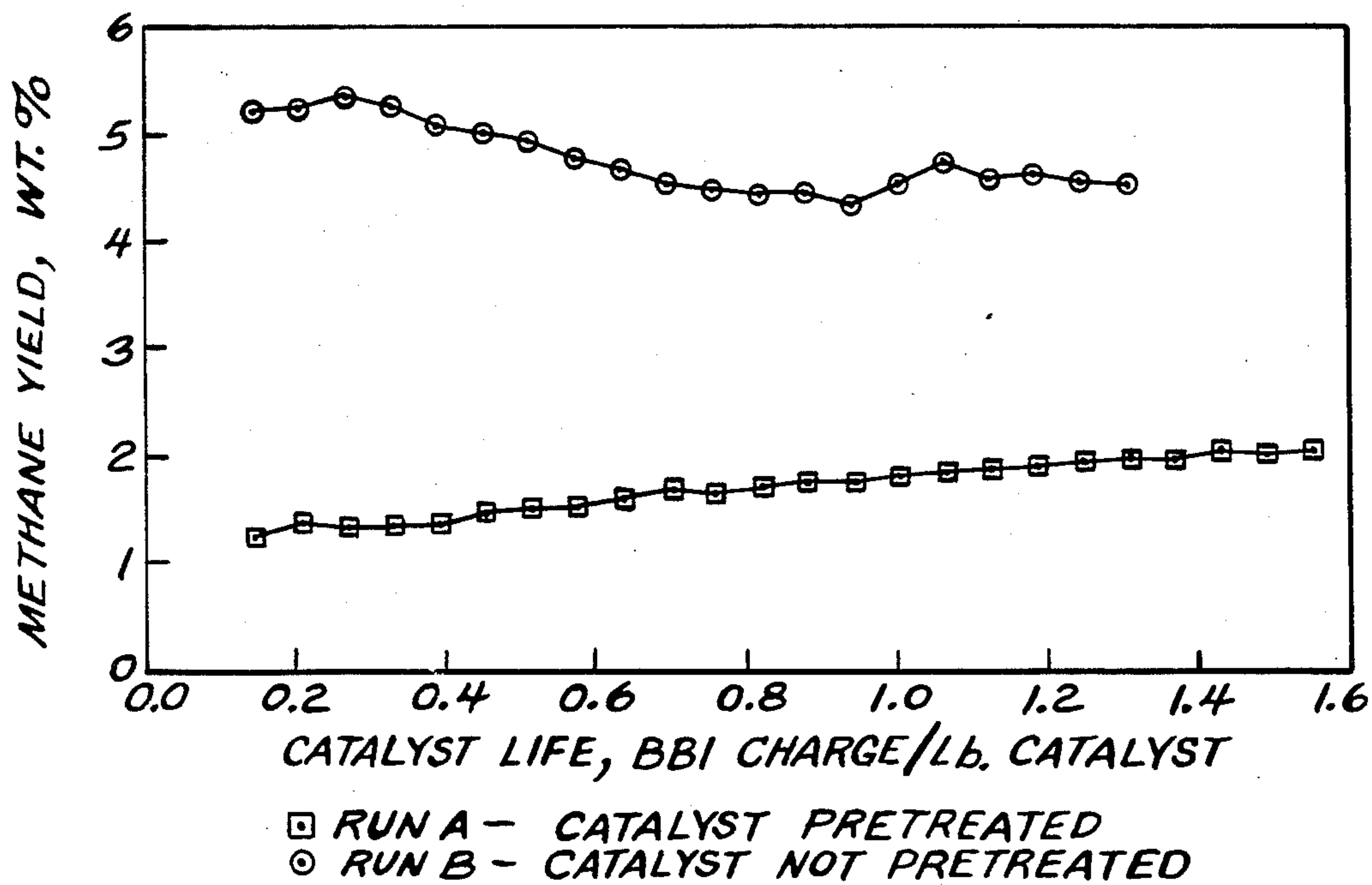
FIG. 6 METHANE YIELD VS. CATALYST LIFE
