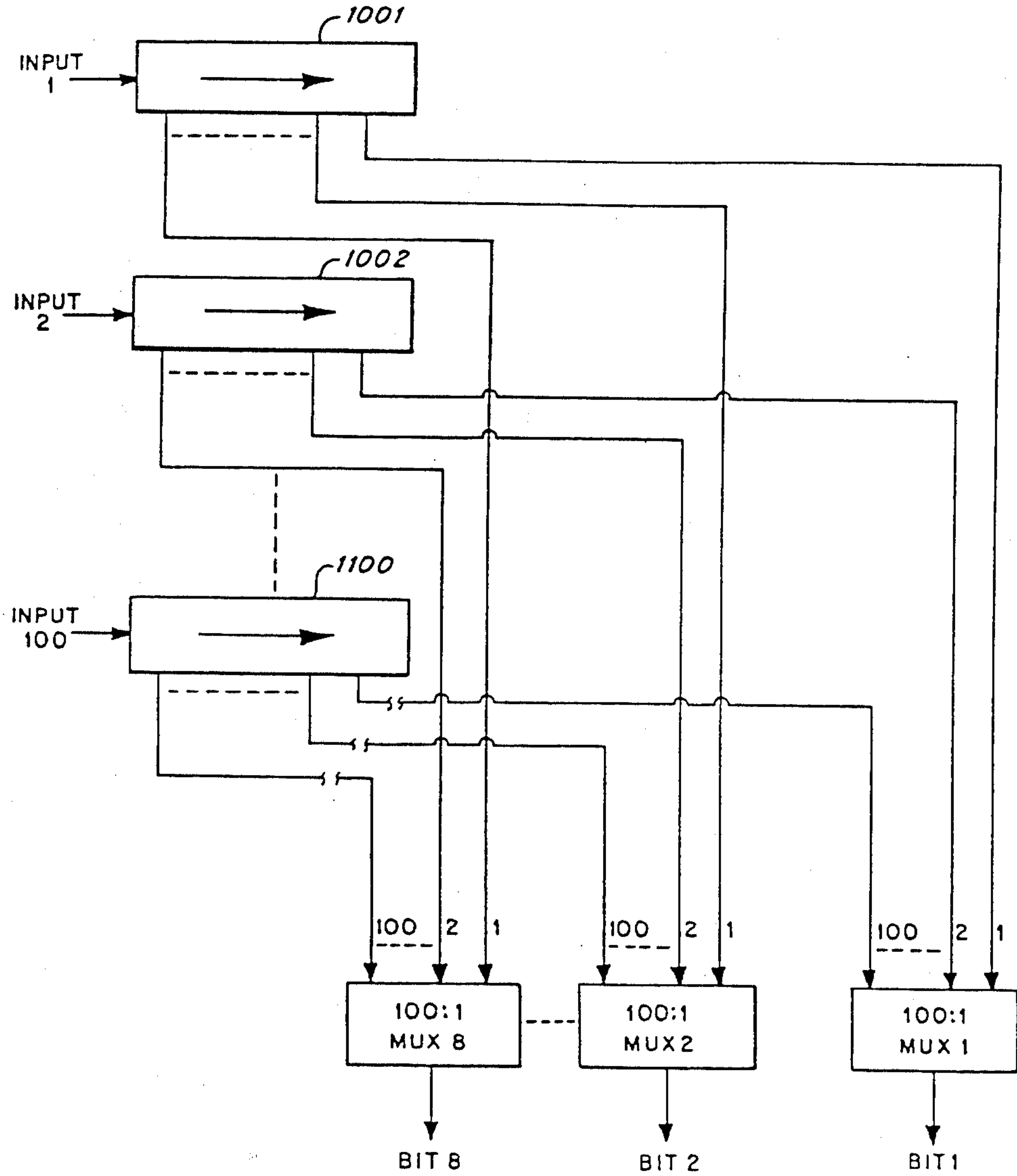
Fig. 9 PRIOR ART
