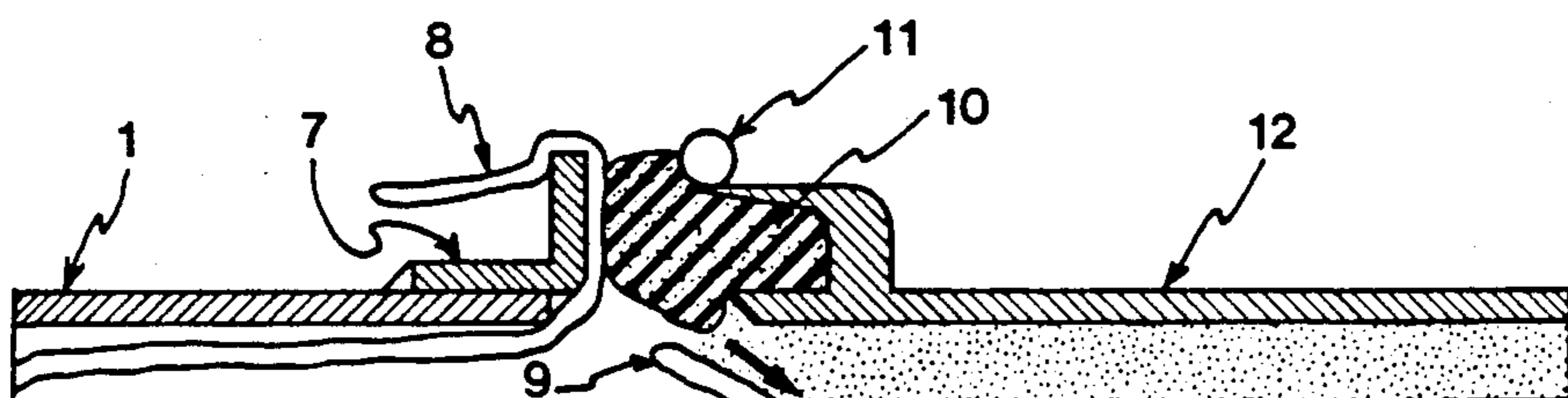
FIGURE 7c - Slip Seal
