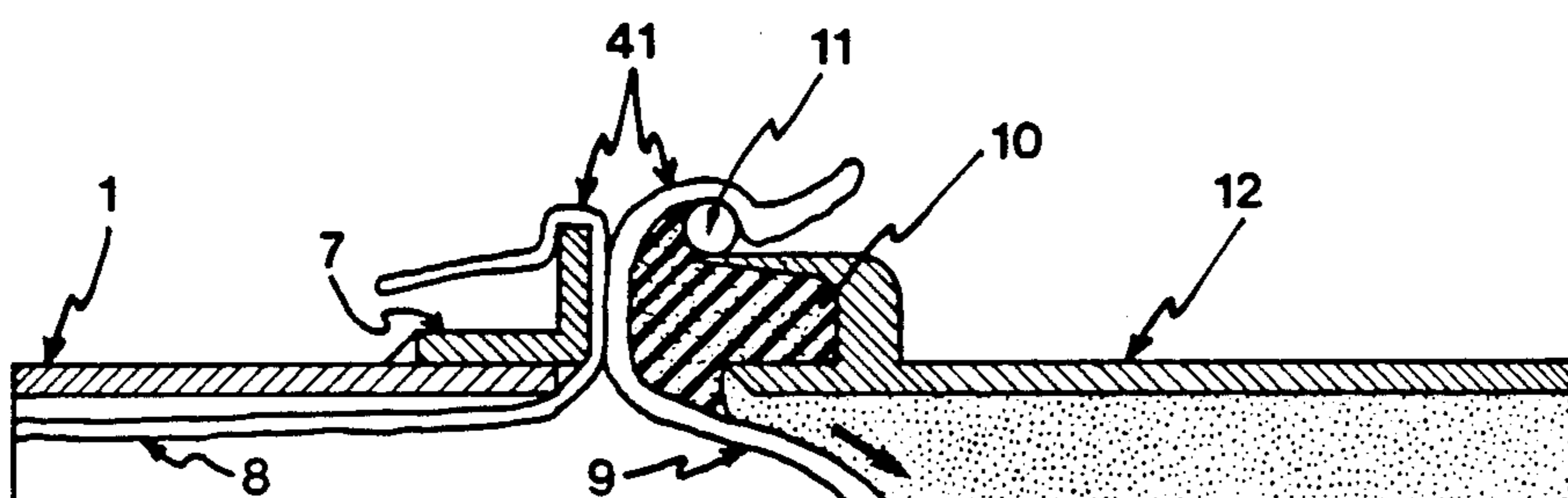
FIGURE 7b - Contact Seal
