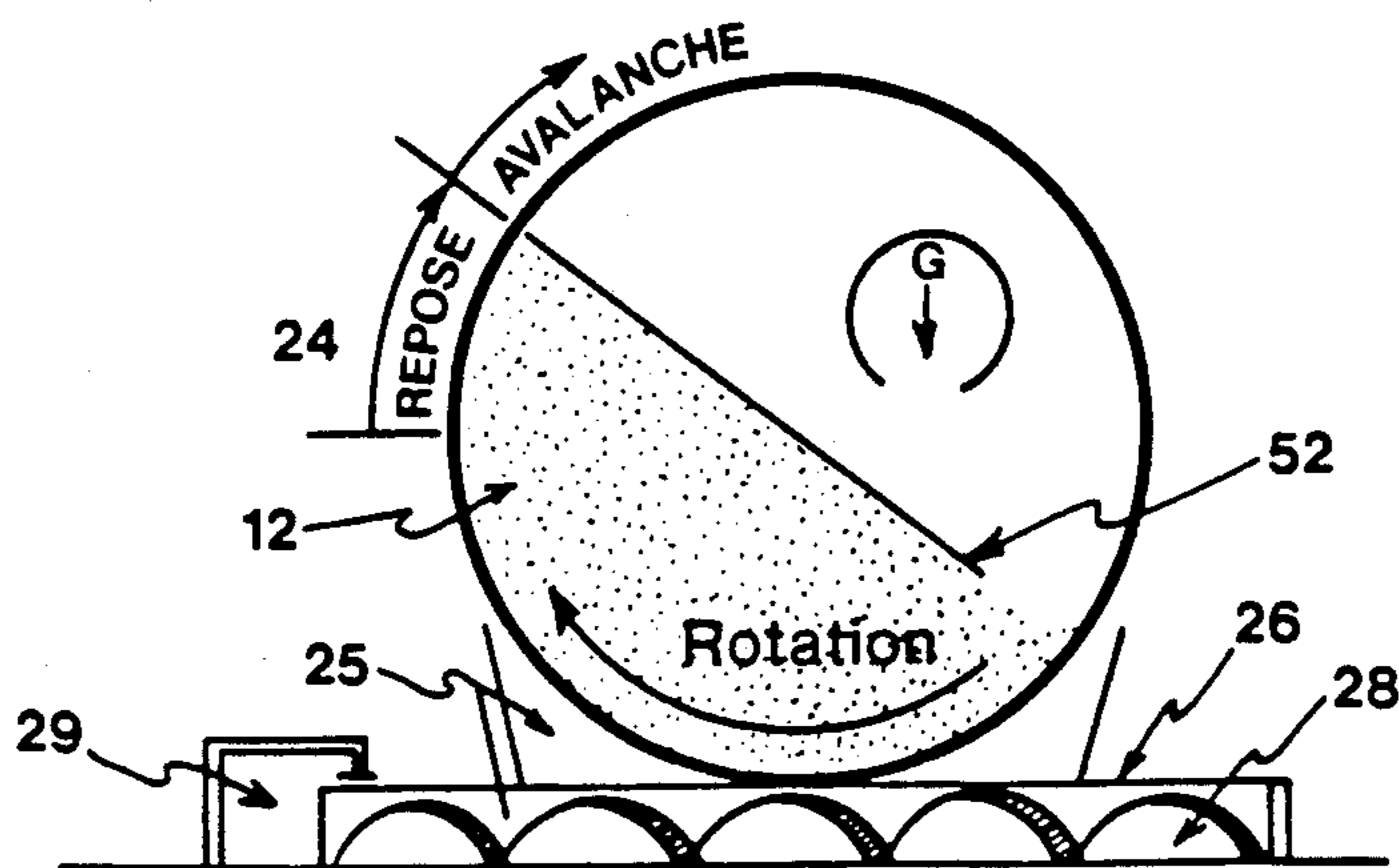
FIGURE 6 - Drum Rotation
