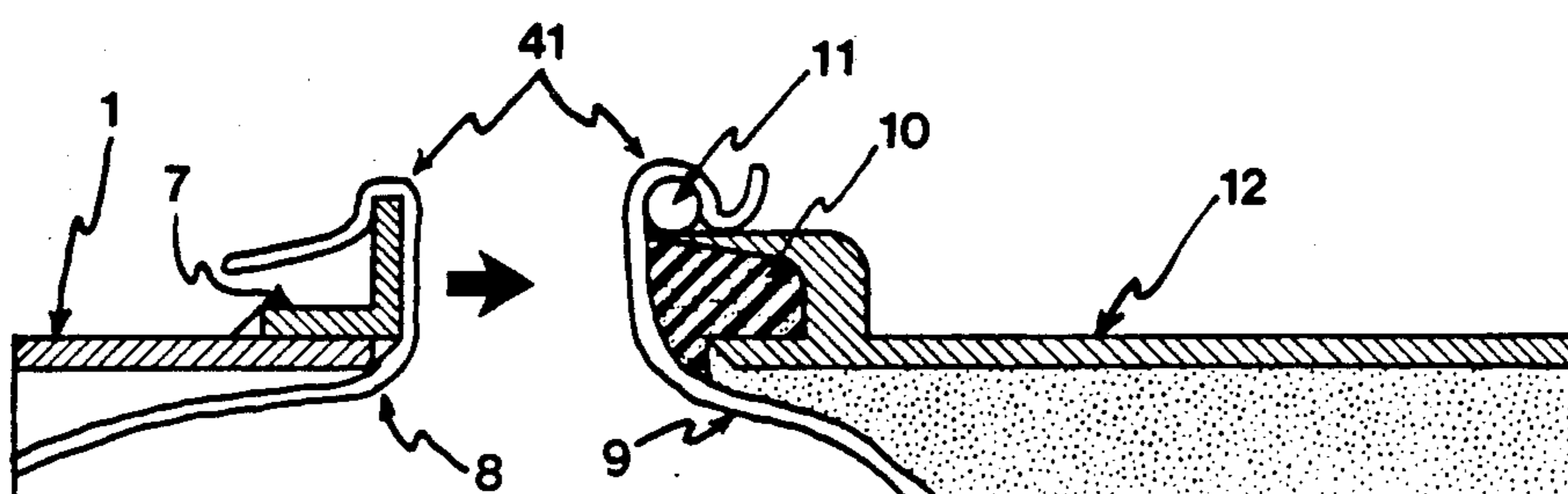
FIGURE 7a - Drum Attachment
