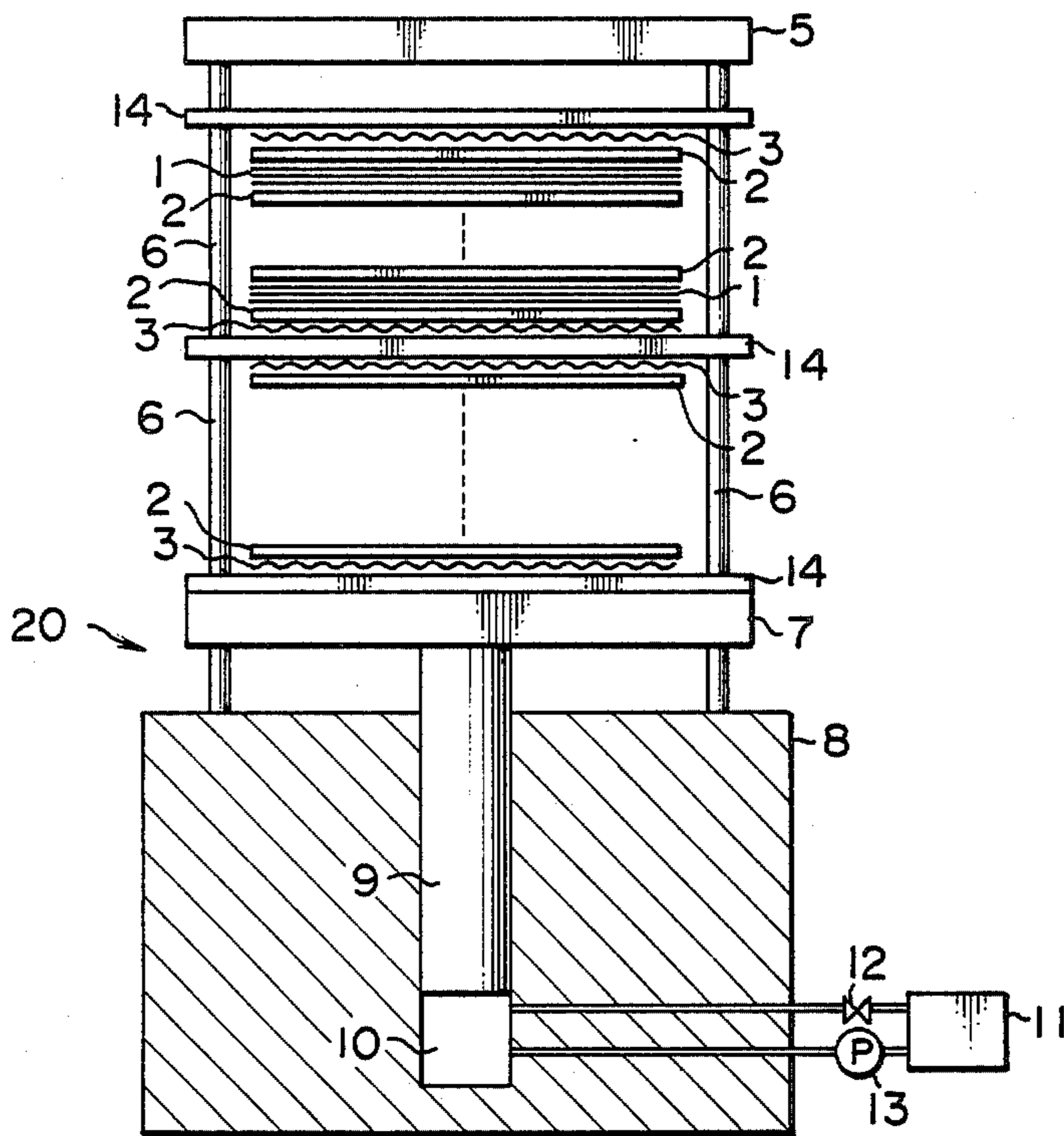
FIG. 2 PRIOR ART
