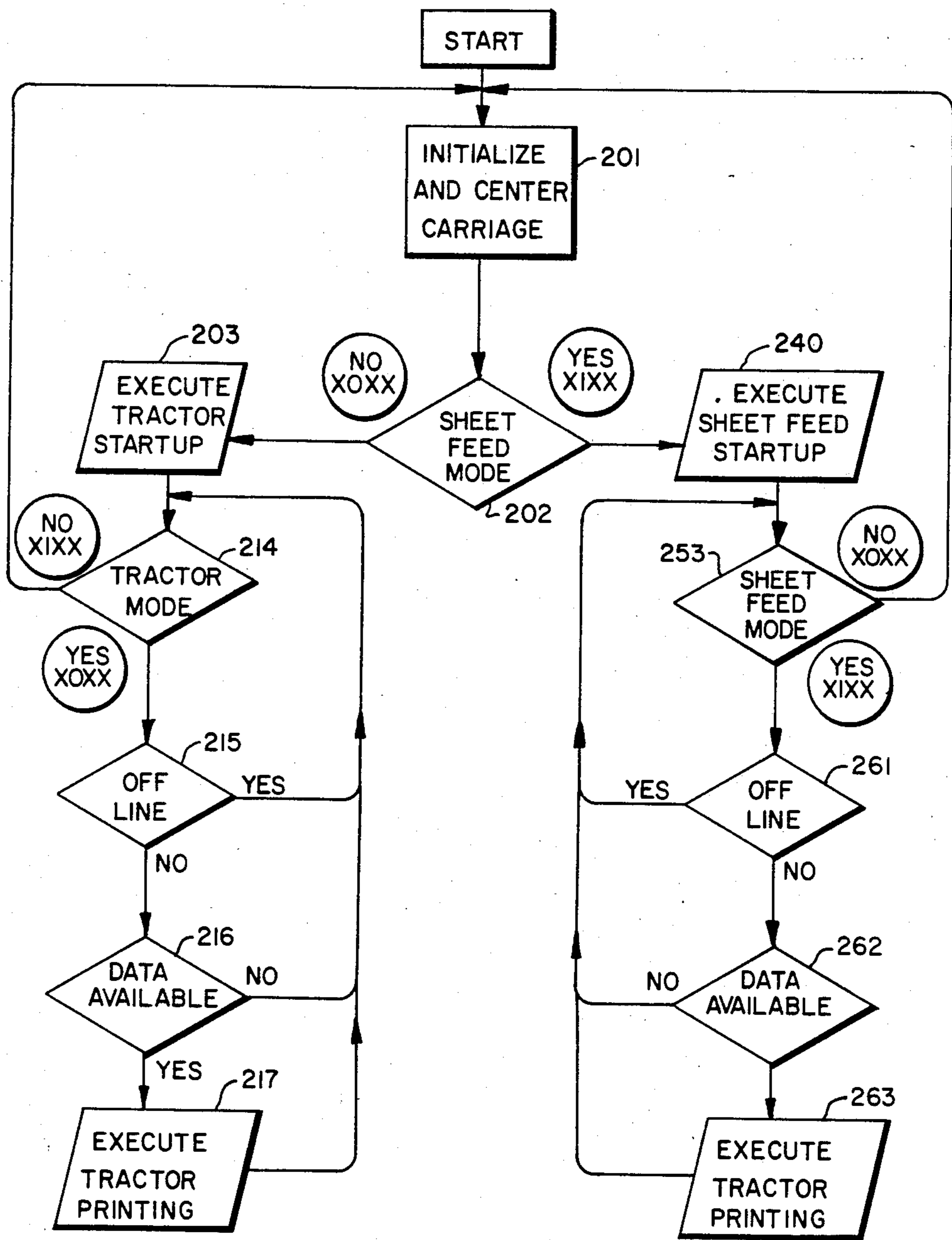
FIG. 12 MASTER FLOW CHART
