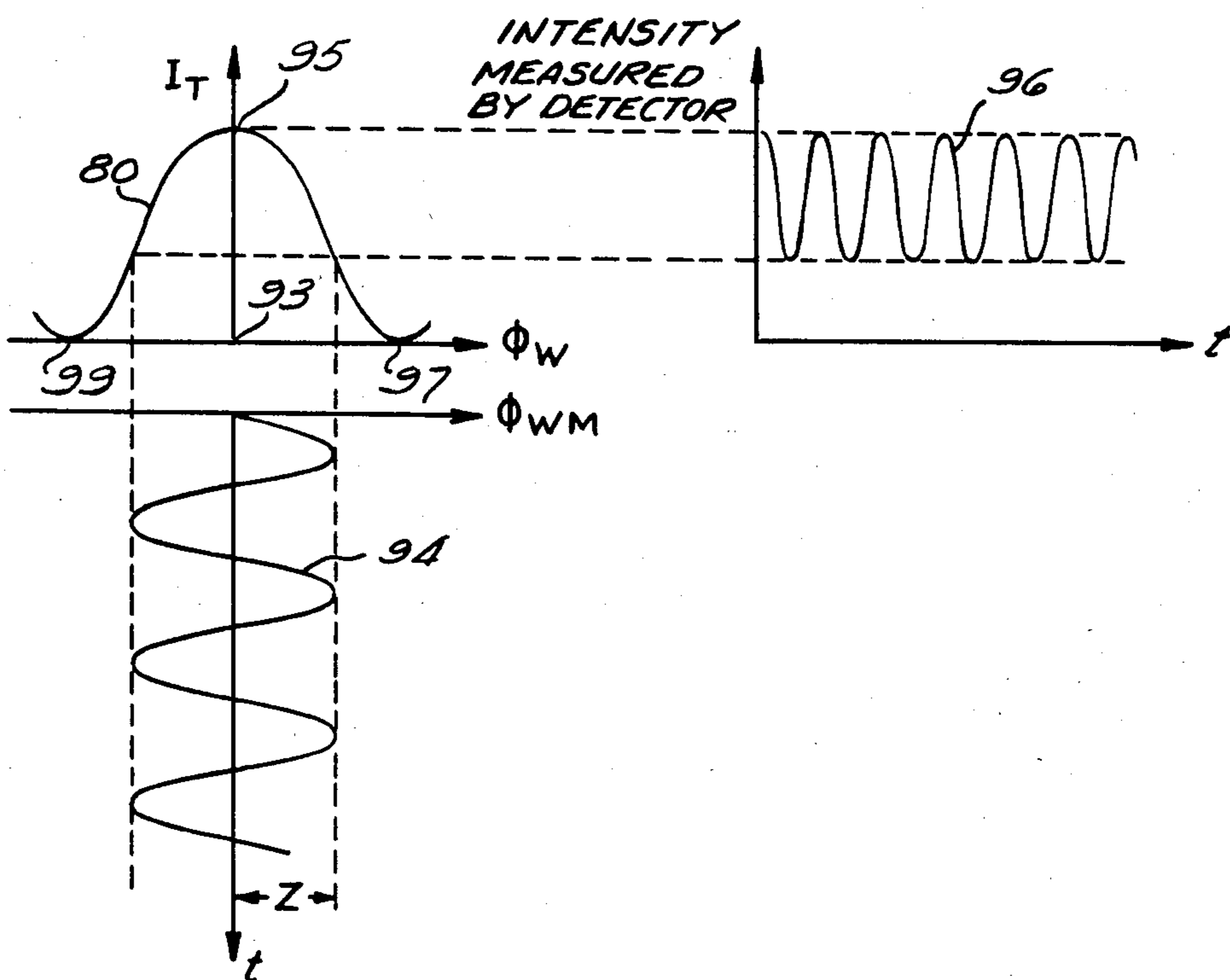
Fig. 8 (PRIOR ART)
