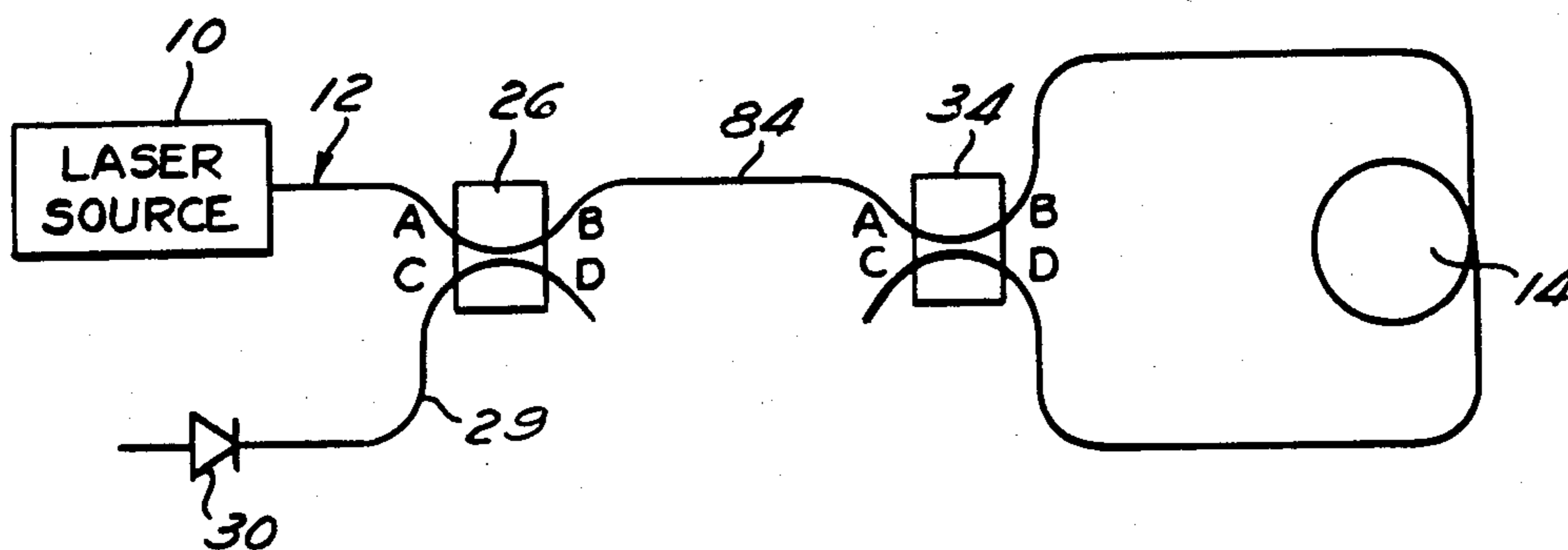
Fig. 5 (PRIOR ART)
