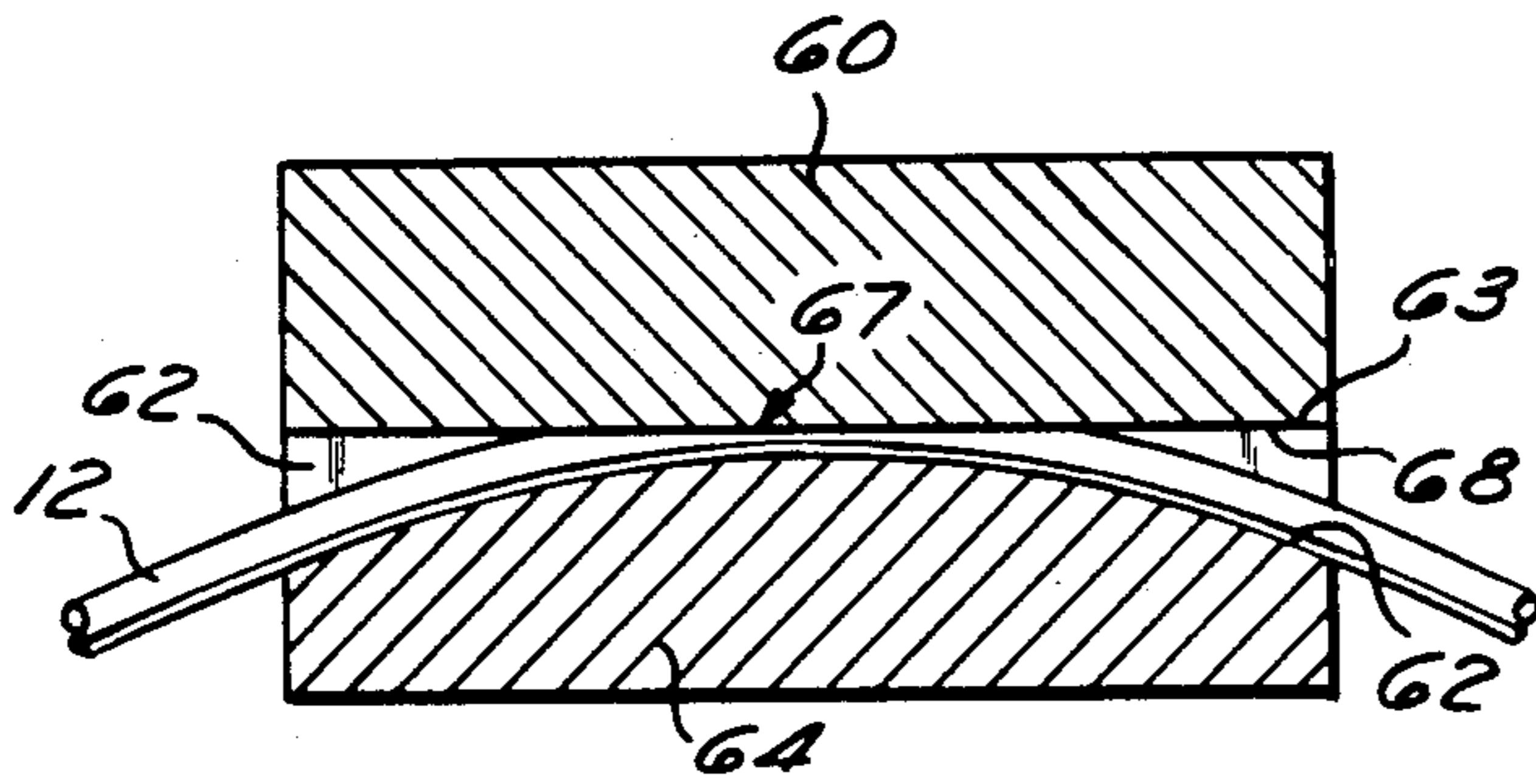
Fig. 3 (PRIOR ART)
