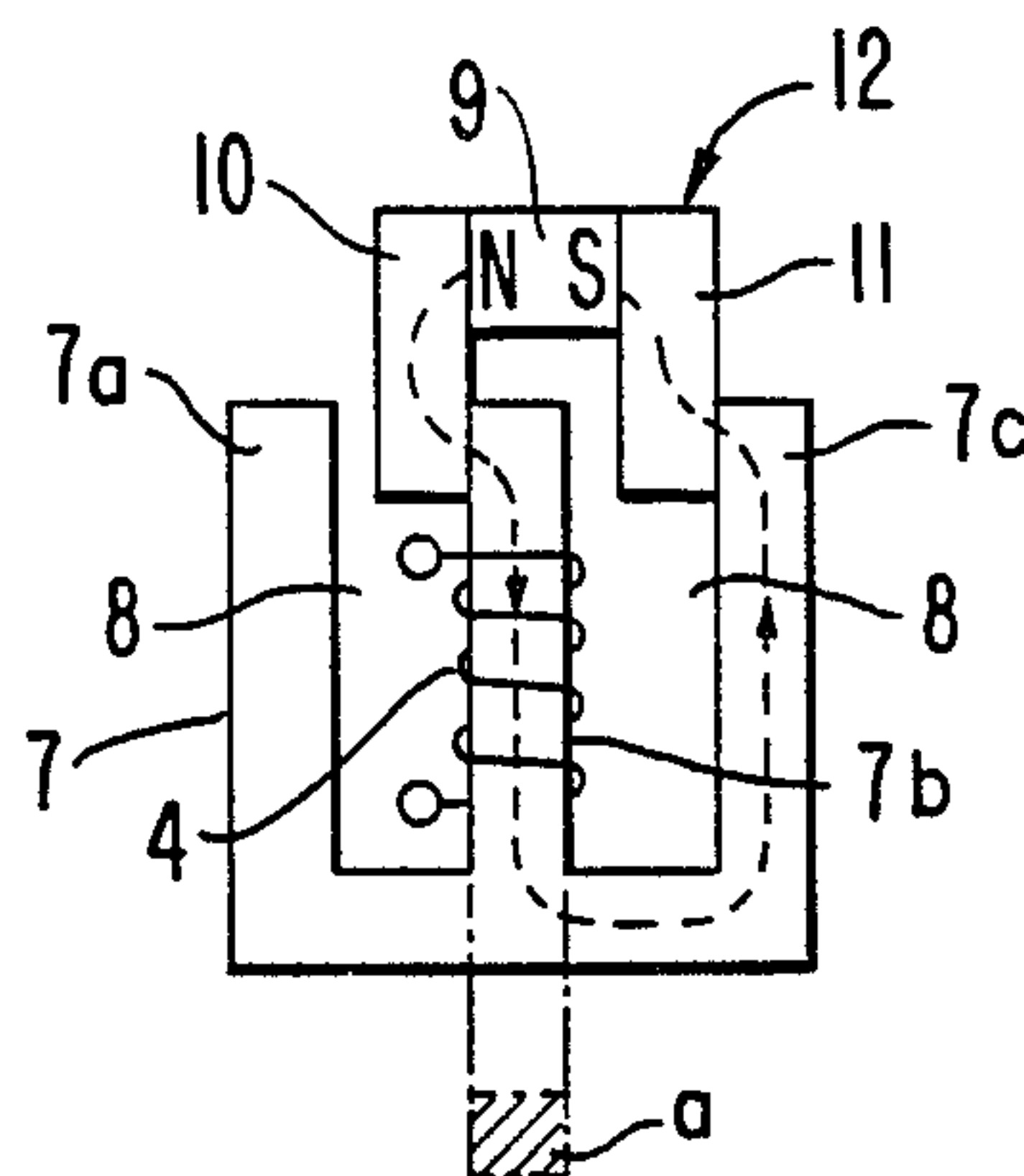
FIG. 2. (PRIOR ART)
