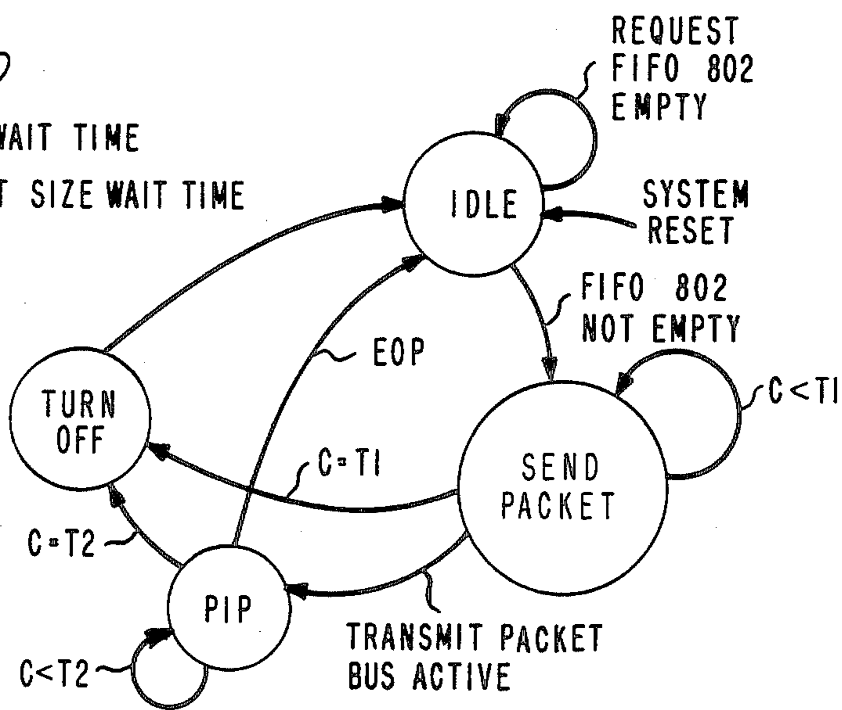
OUTPUT CONTROLLER 803
