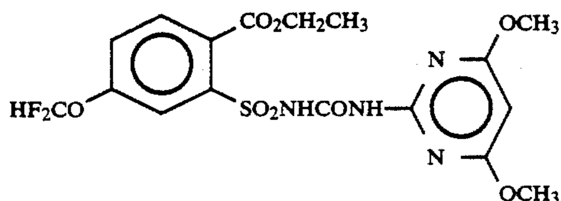
Compound 16
