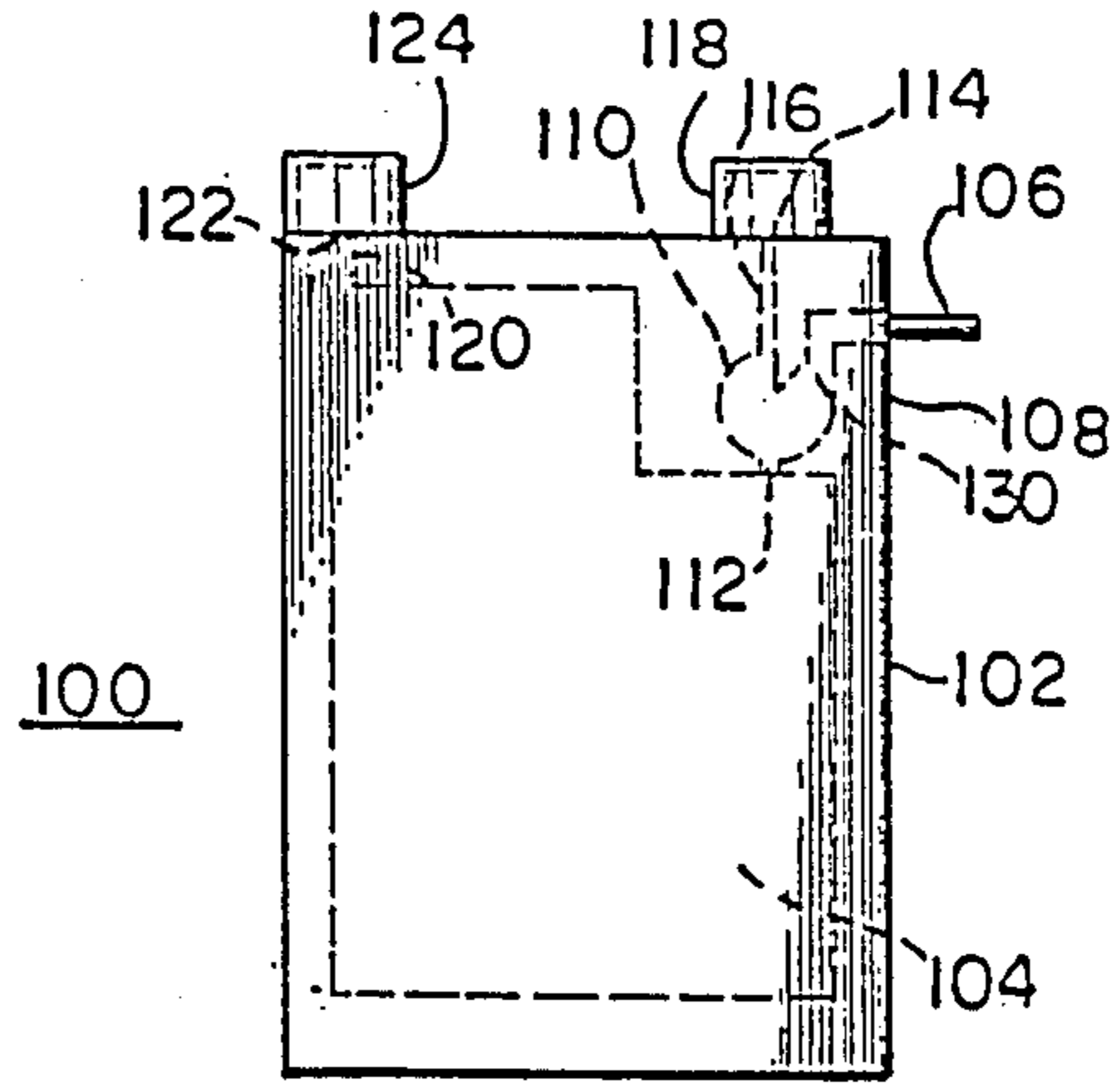
FIG. 2 (PRIOR ART)
