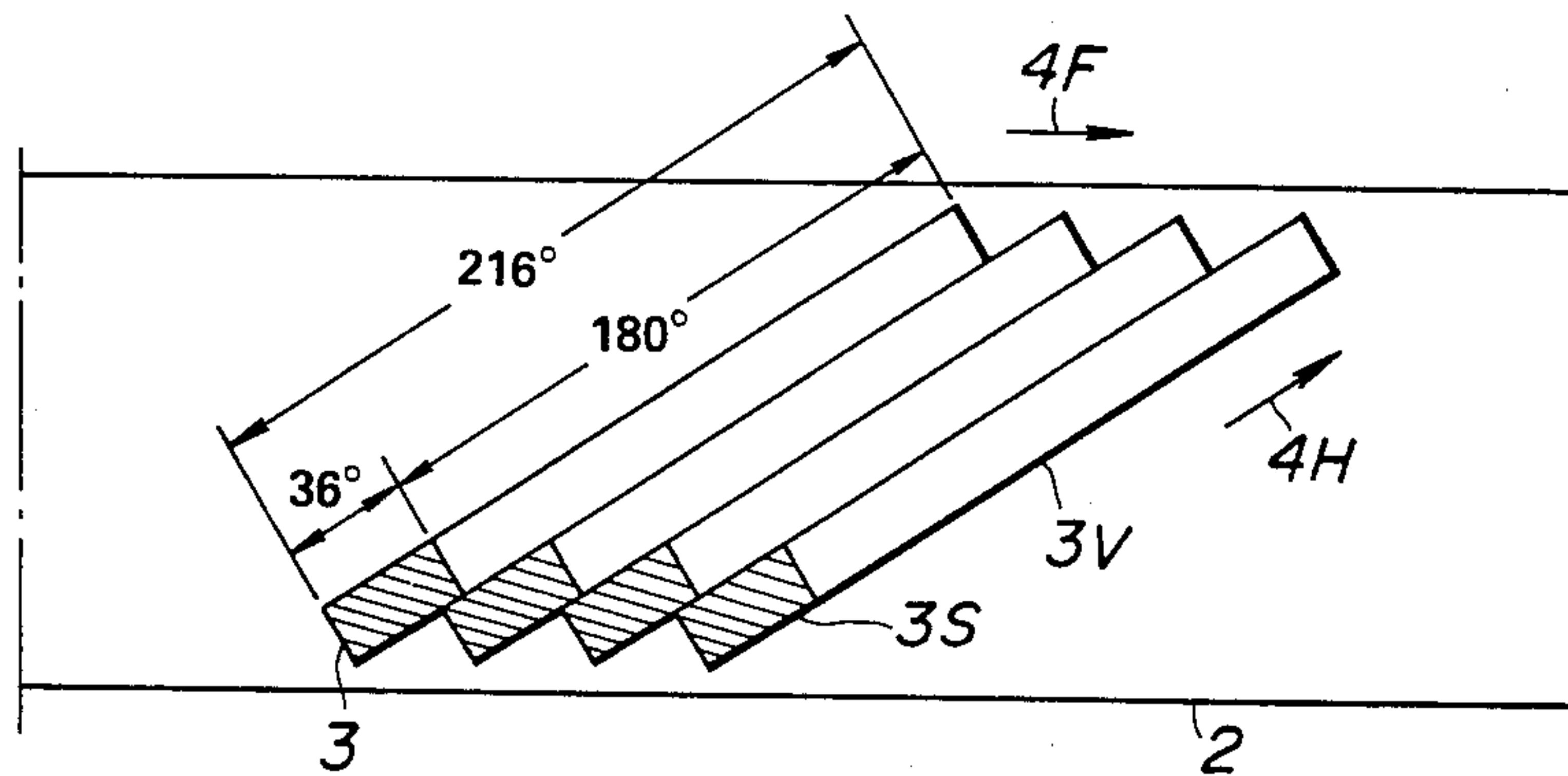
FIG. 1 (PRIOR ART)
