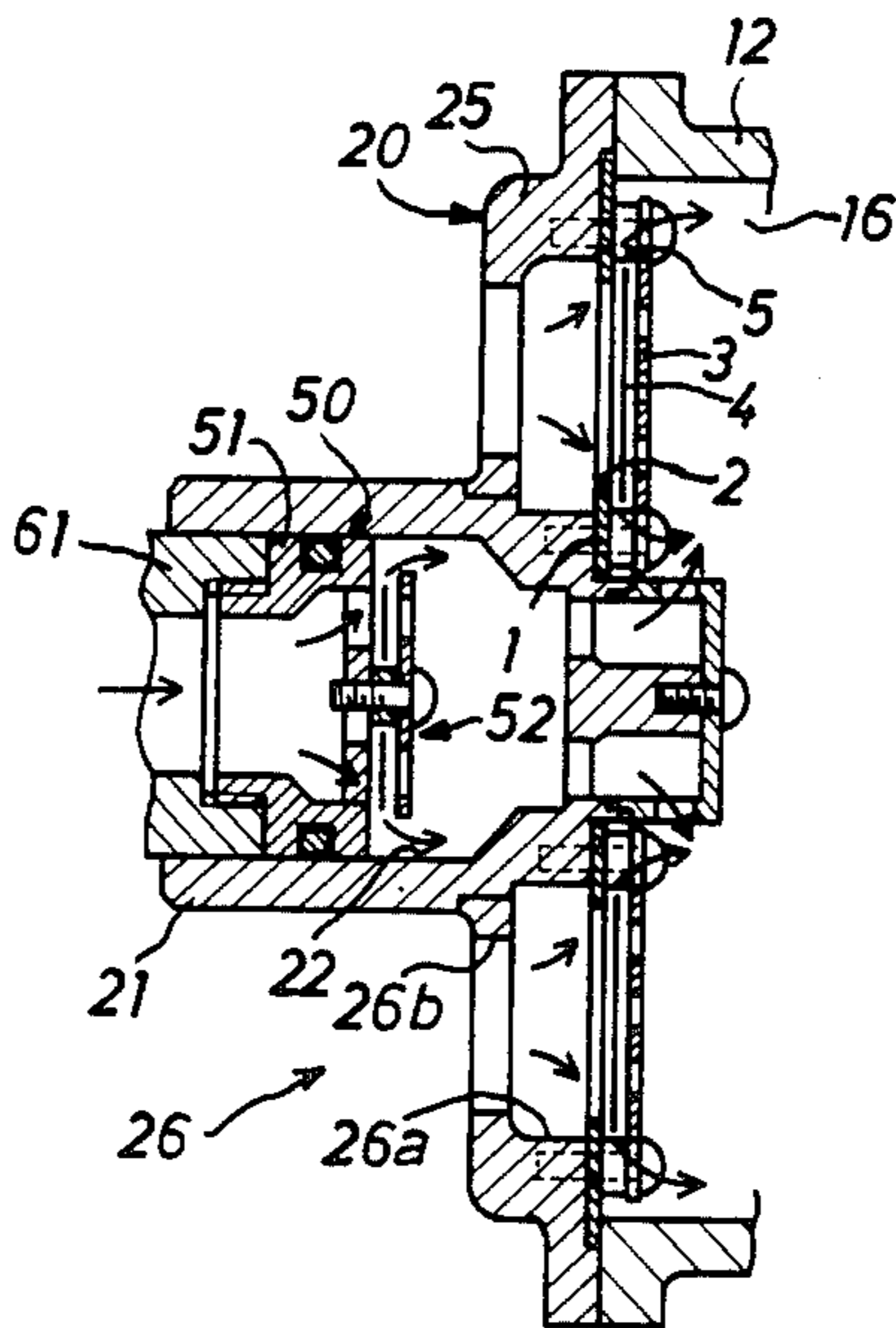
Fig. 3 PRIOR ART
