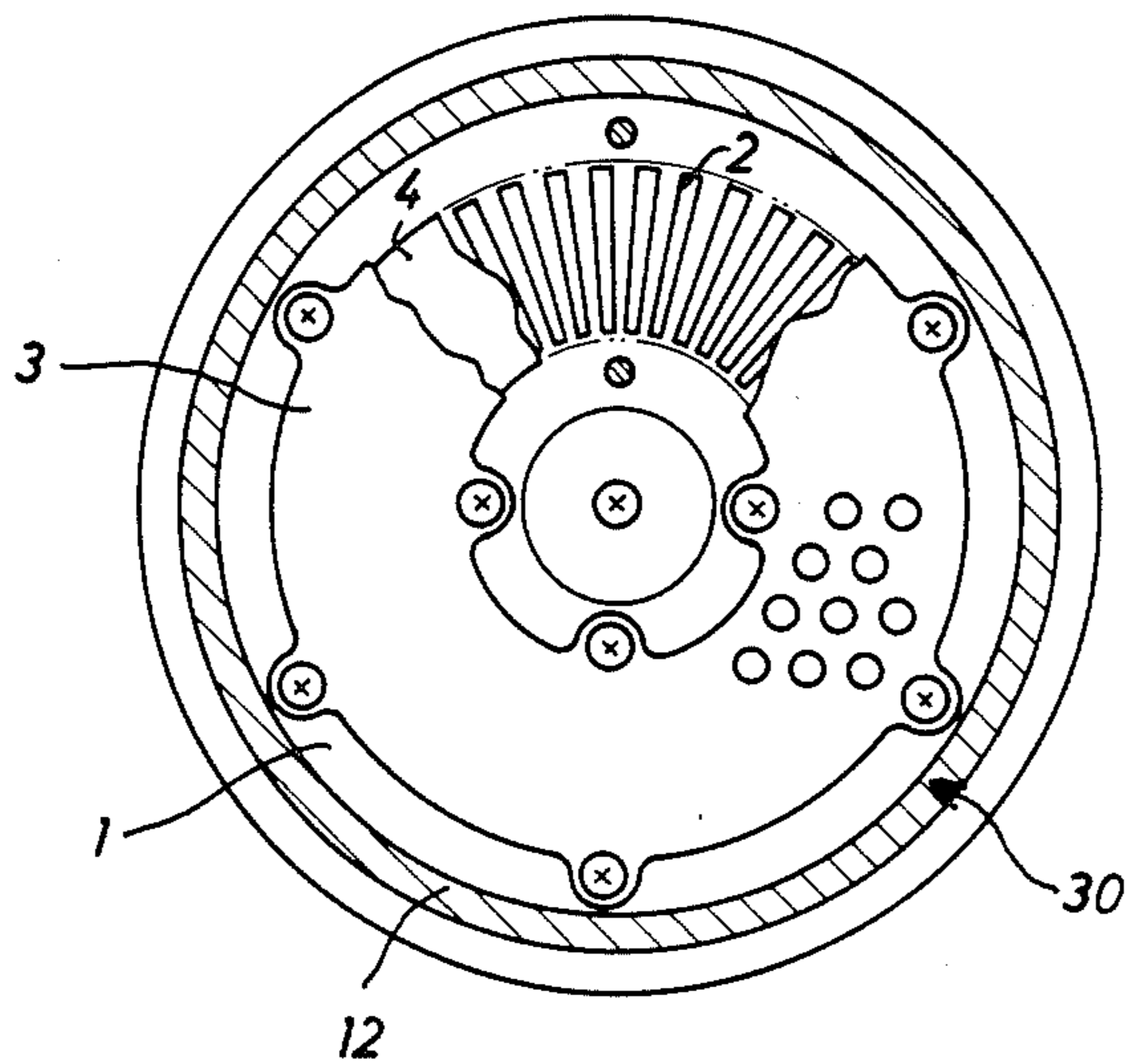
Fig. 4 PRIOR ART
