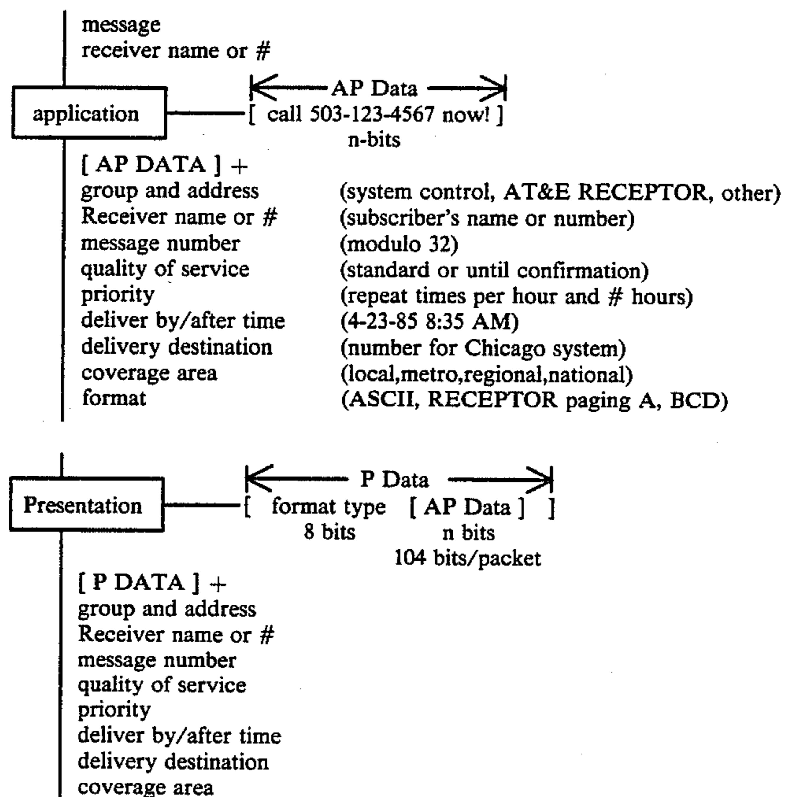
OSI REFERENCE MODEL OF TRANSMISSION SYSTEM
