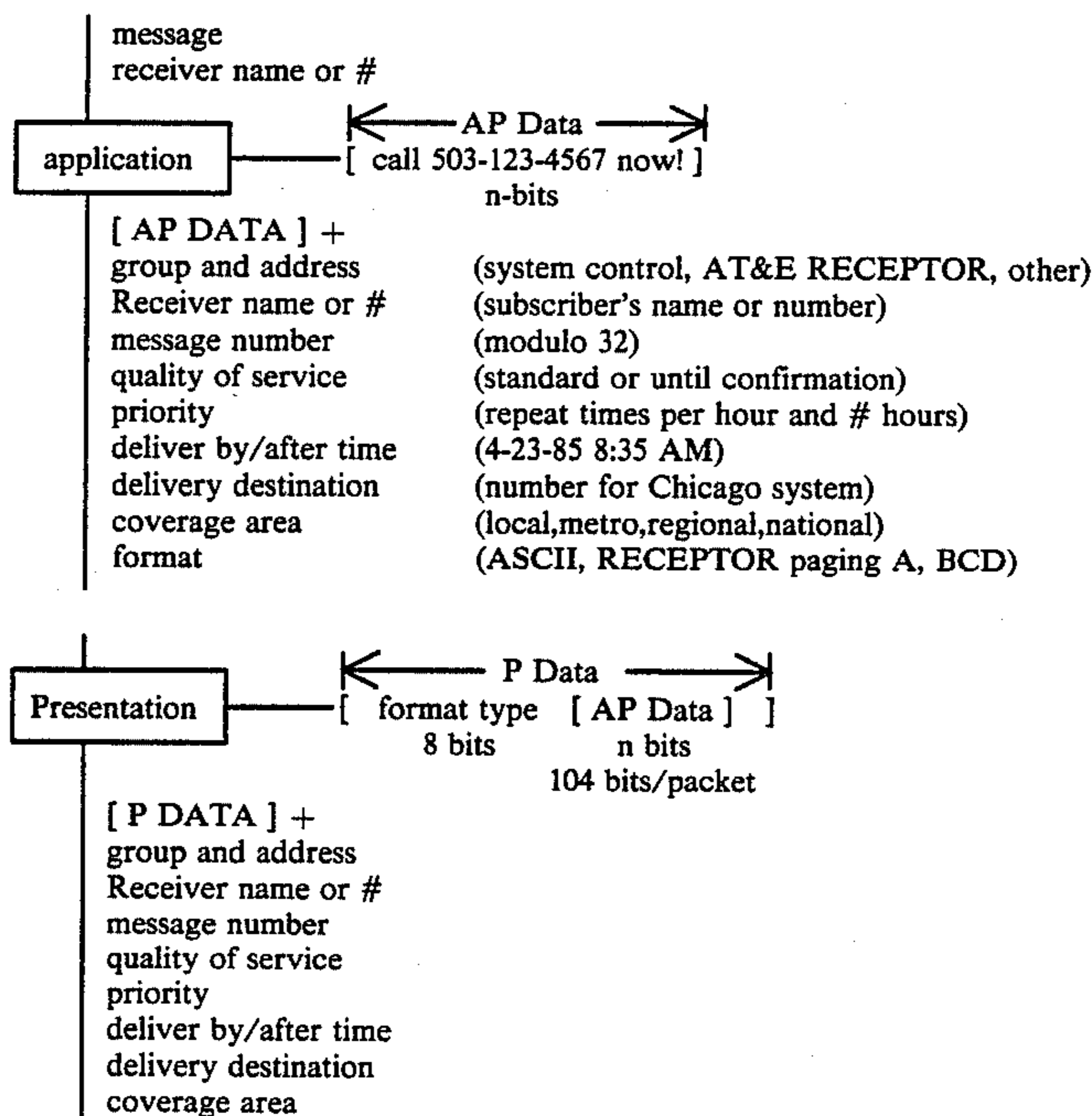
OSI REFERENCE MODEL OF TRANSMISSION SYSTEM
