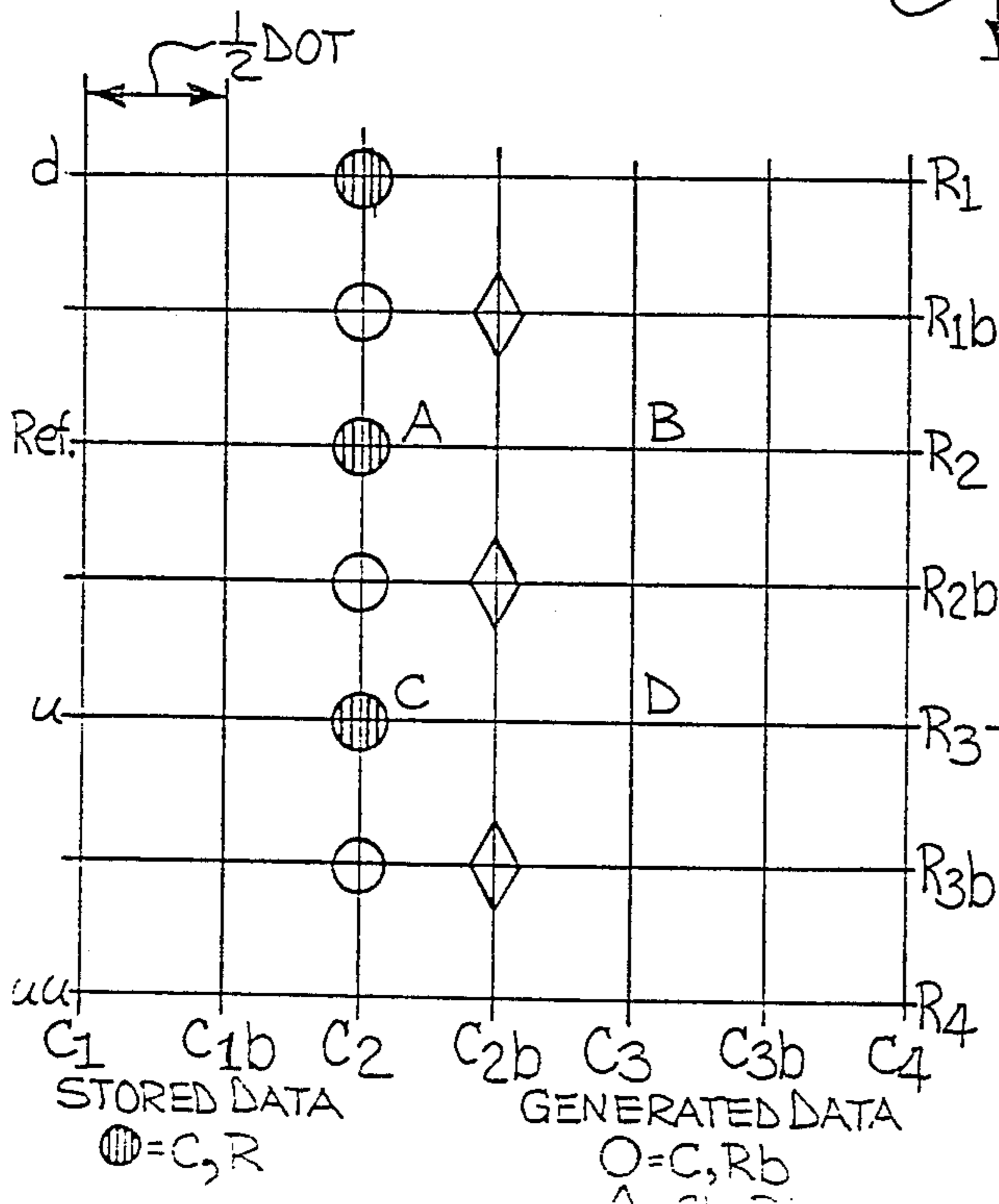
Fig-12 A PREDETERMINED MATRIX D-P
