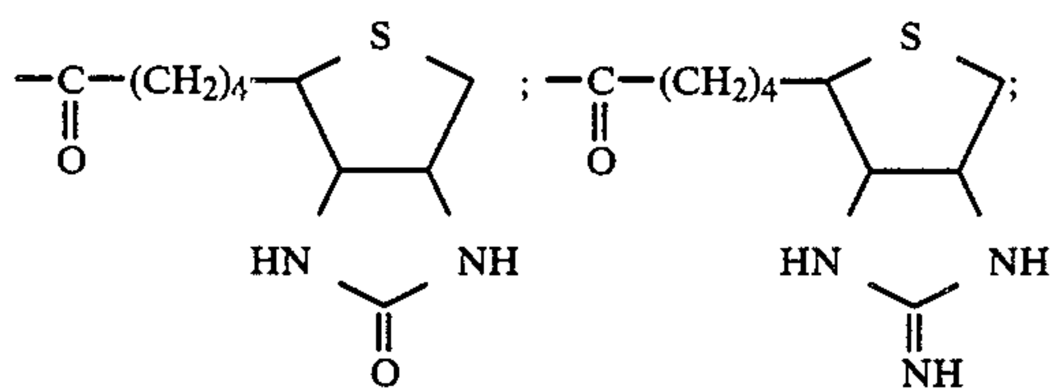
biotin
