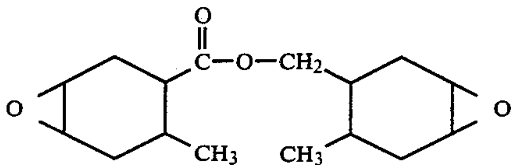
3,4-epoxy-6-methylcyclohexylmethyl 3,4-epoxy-6-methylcyclohexenecarboxylate
