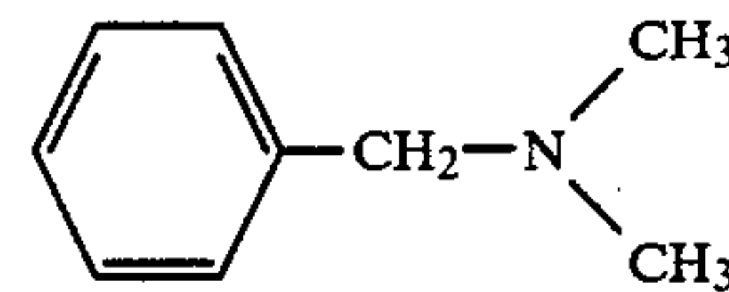
α-methylbenzyl dimethylamine
