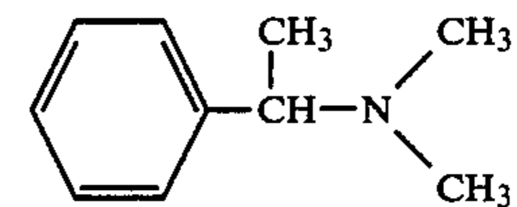
dimethylaminomethylphenol
