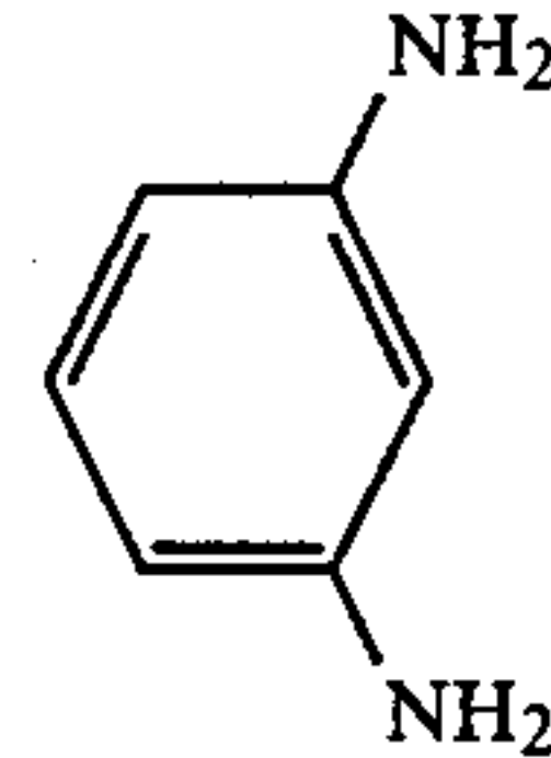
p,p'-diaminophenyl methane
