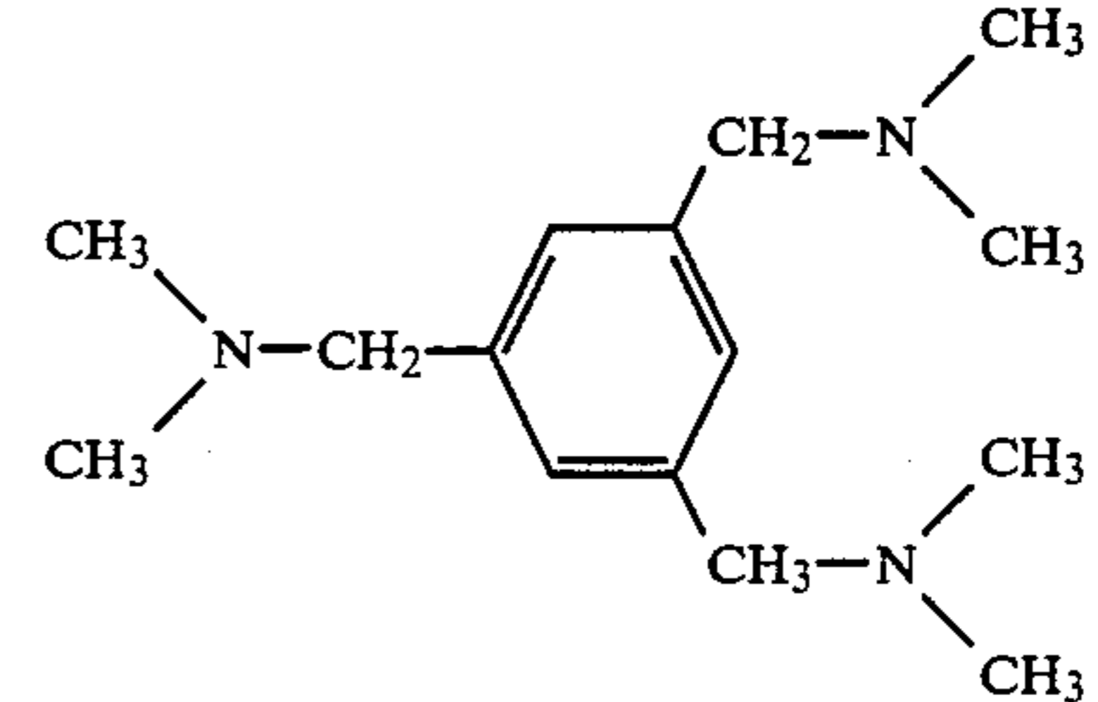
tridimethylaminomethylbenzene
