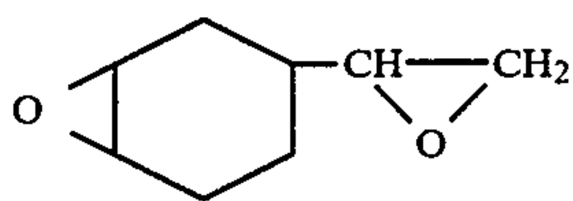
3,4-epoxy-6-methylcyclohexylmethyl 3,4-epoxy-6-methylcyclohexenecarboxylate
