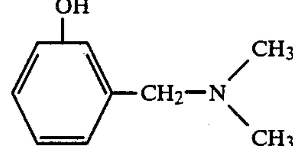
tridimethylaminomethylbenzene
