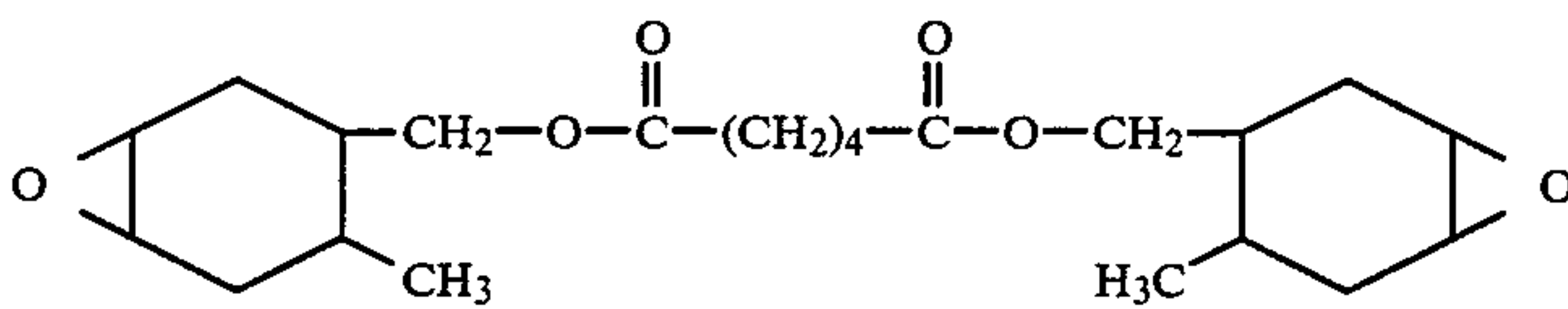
(27) bis(3,4-epoxy-6-methylcyclohexylmethyl)adipate
