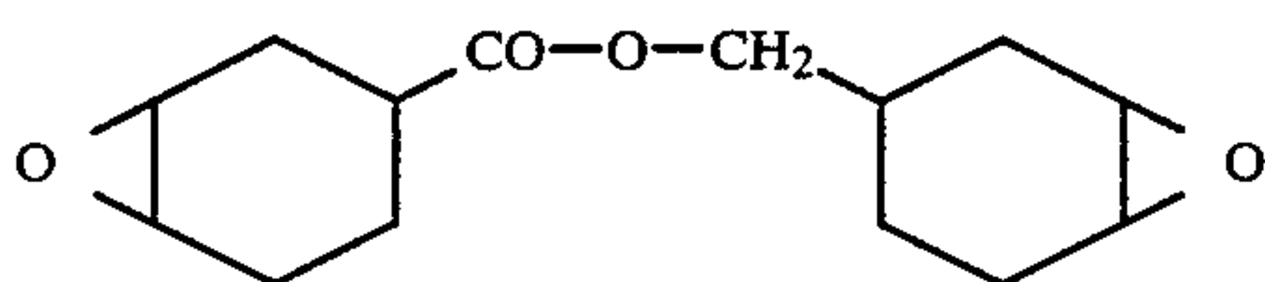
3,4-epoxycyclohexylmethyl 3,4-epoxycyclohexenecarboxylate
