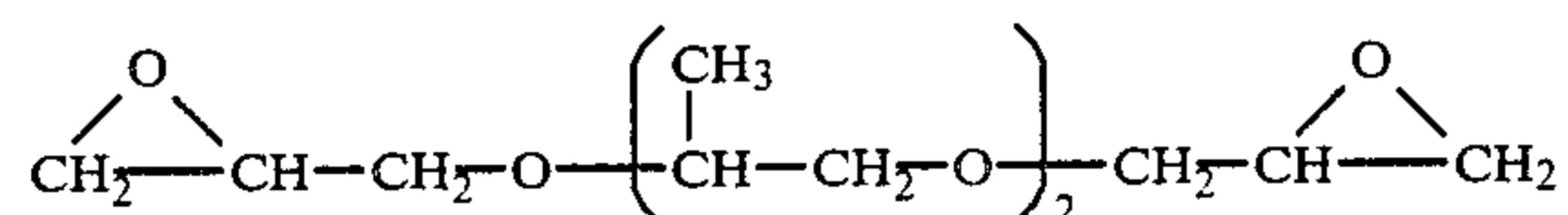
(6) 1,3-bis[3(2,3-epoxypropoxy)propyl]tetramethyl disiloxane
