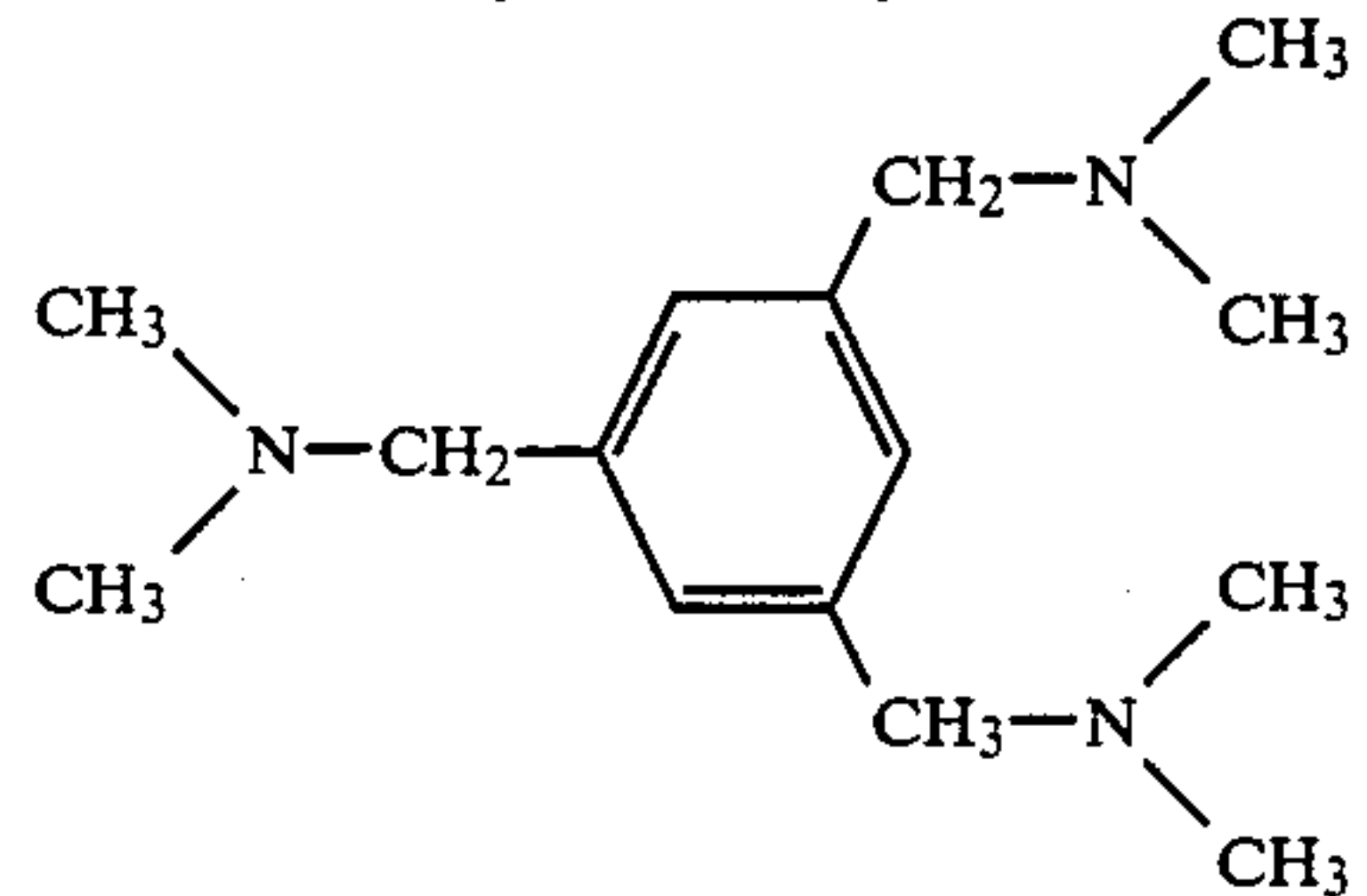
tridimethylaminomethylbenzene
