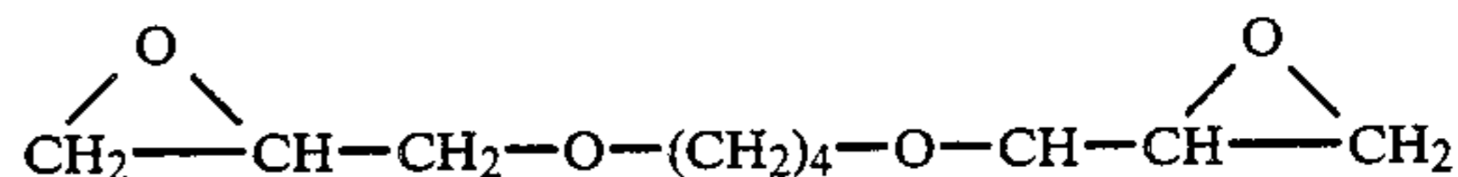
(5) diglycidyl ether of polypropylene glycol
