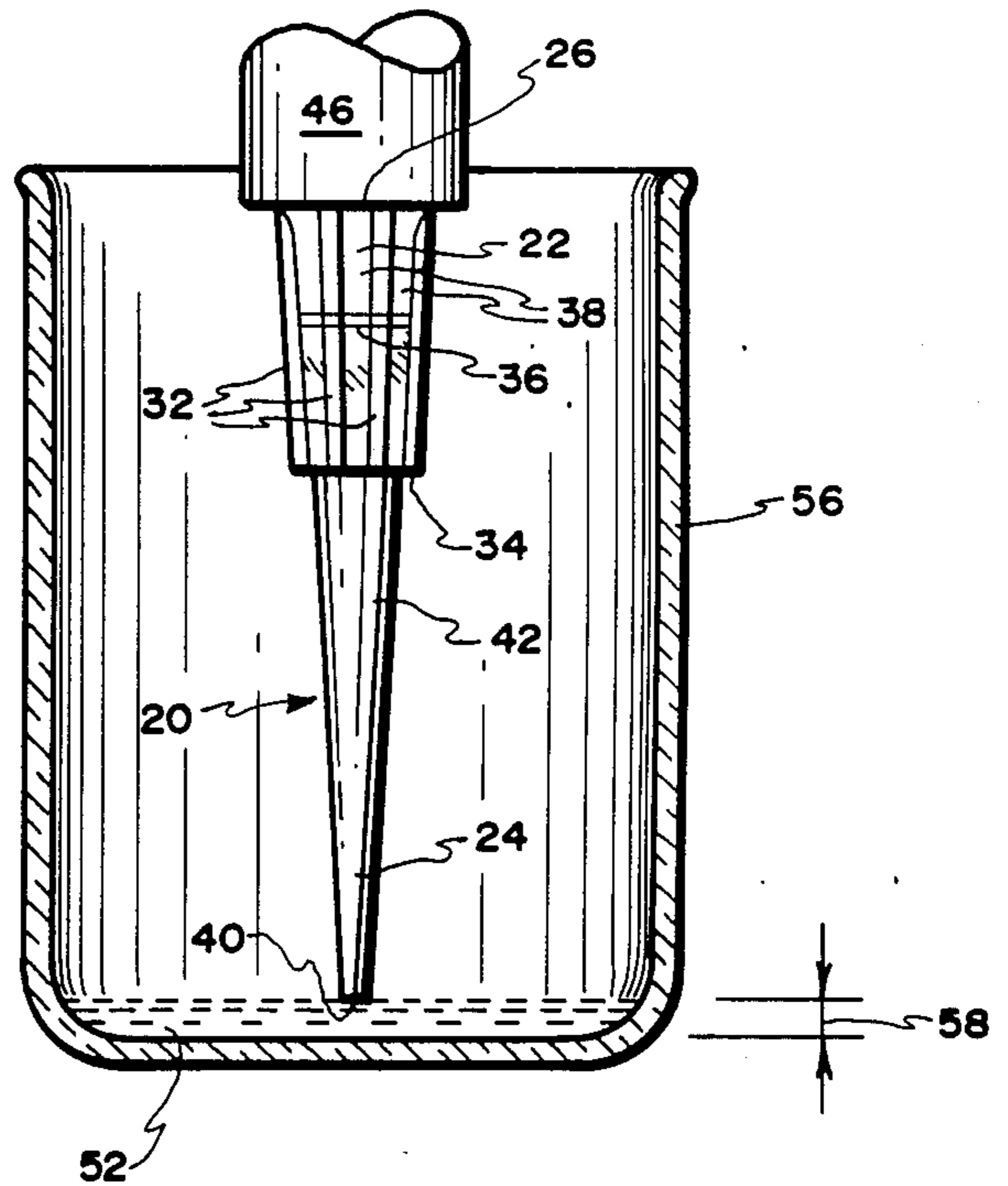
Fig. 4 (PRIOR ART)
