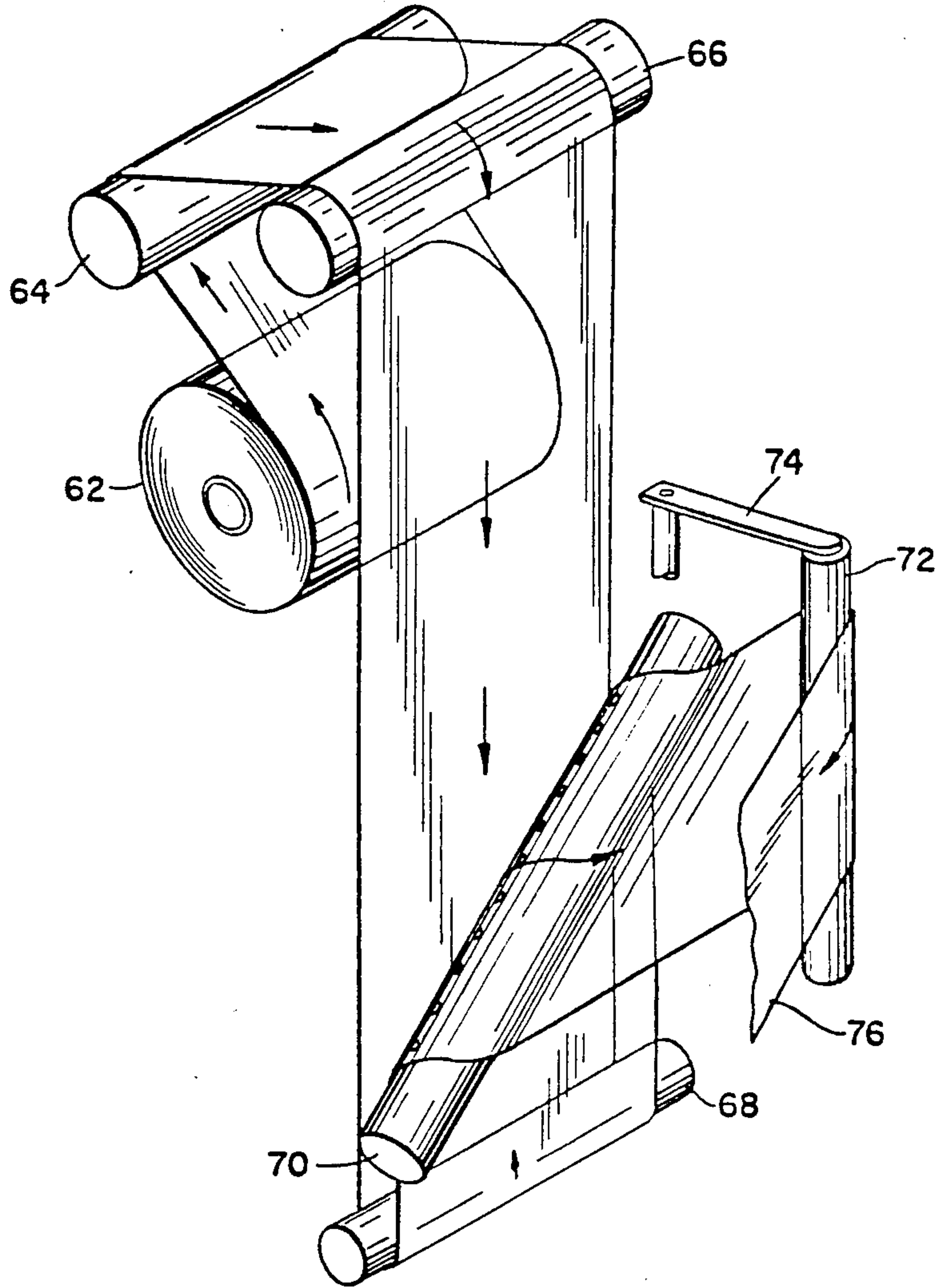
FIG. 8 PRIOR ART
