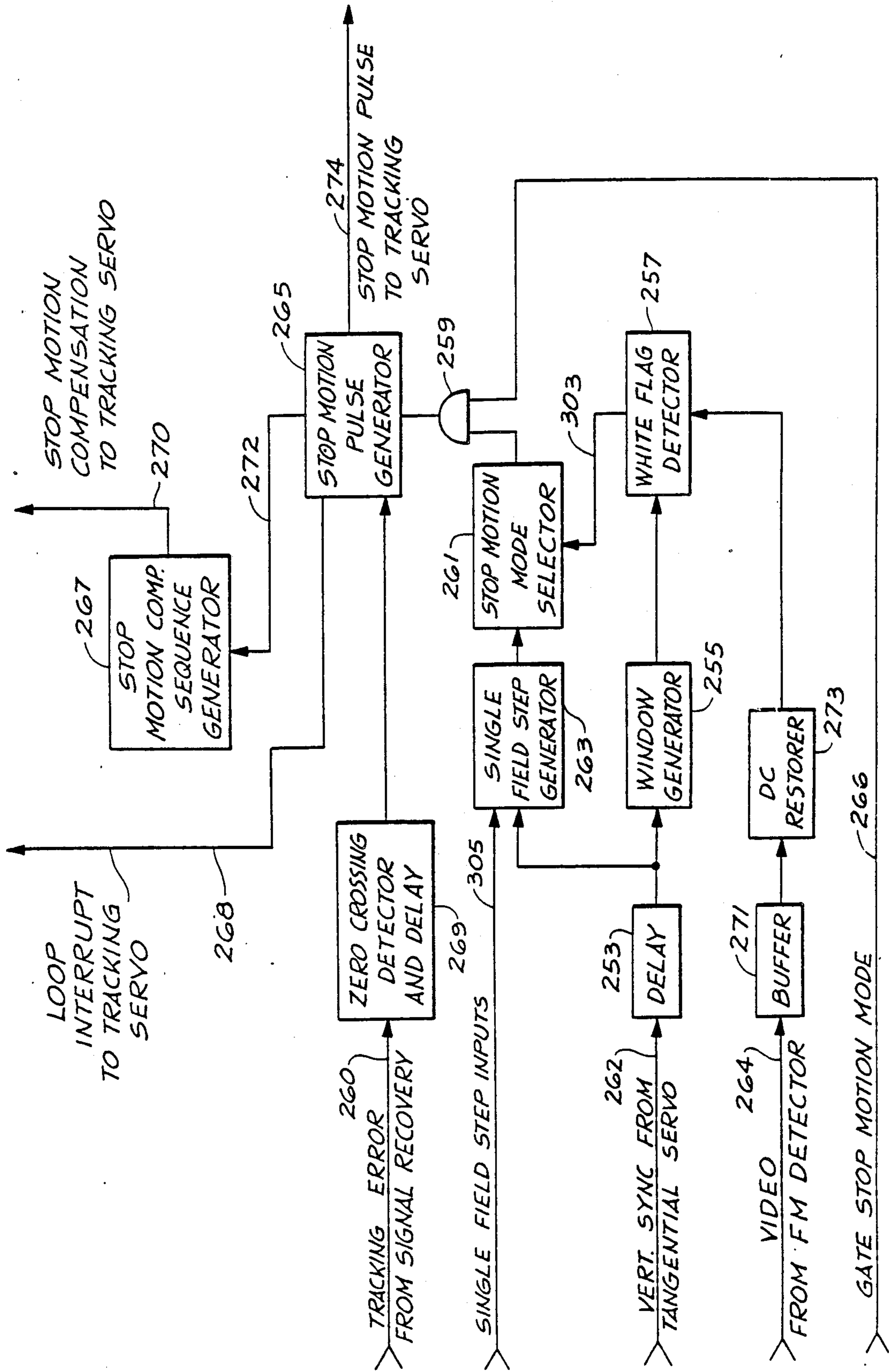
FIG. 7 STOP MOTION
