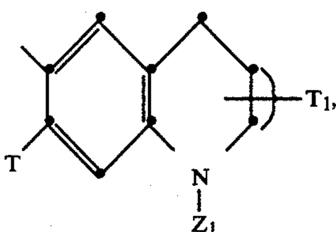
a tetrahydroquinolinyl radical of the formula
