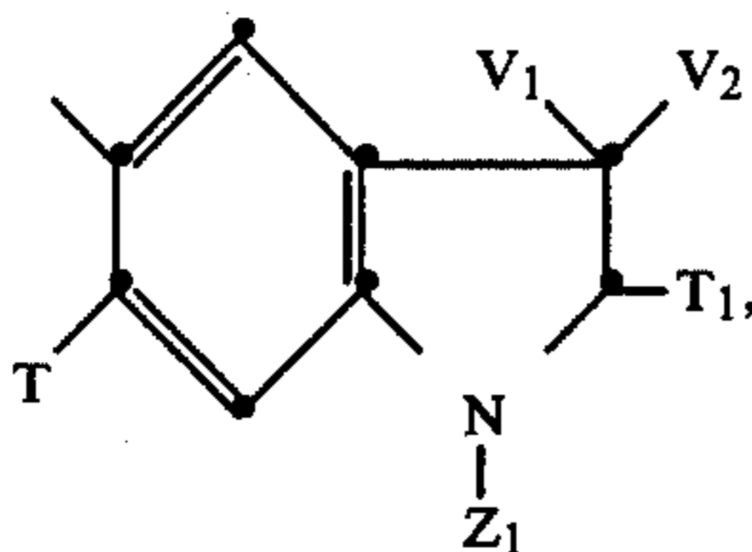
a tetrahydroquinolinyl radical of the formula
