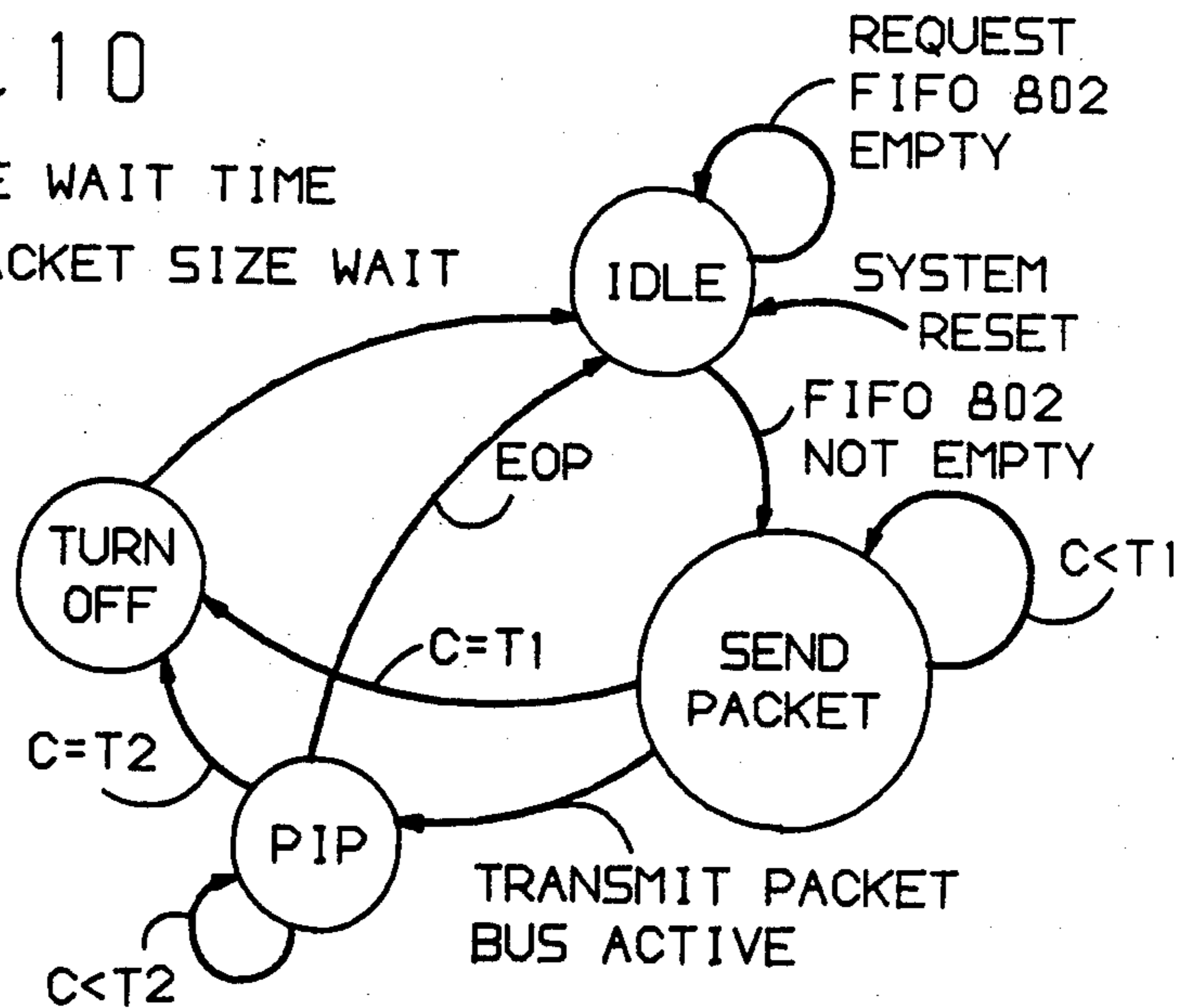
OUTPUT CONTROLLER 803
