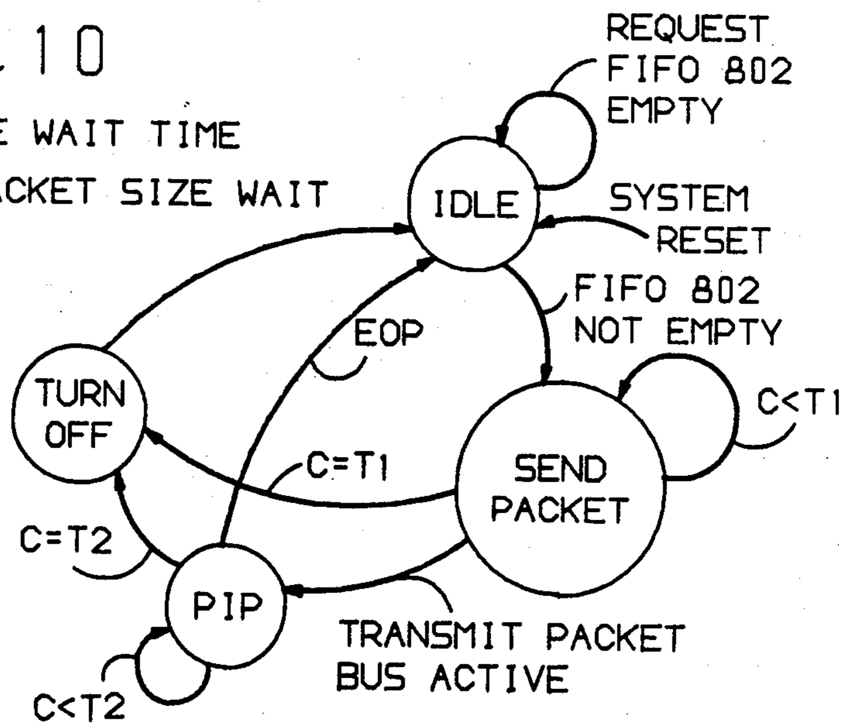
OUTPUT CONTROLLER 803
