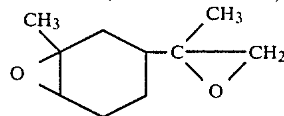
dipentene diepoxide
