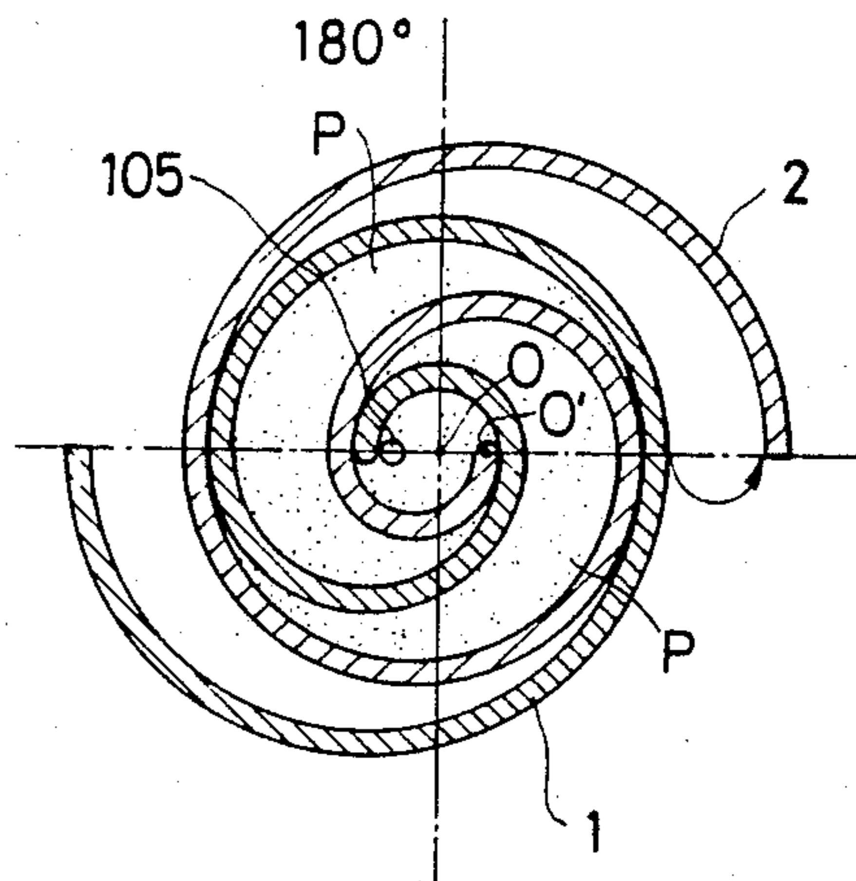
FIG. 1C PRIOR ART
