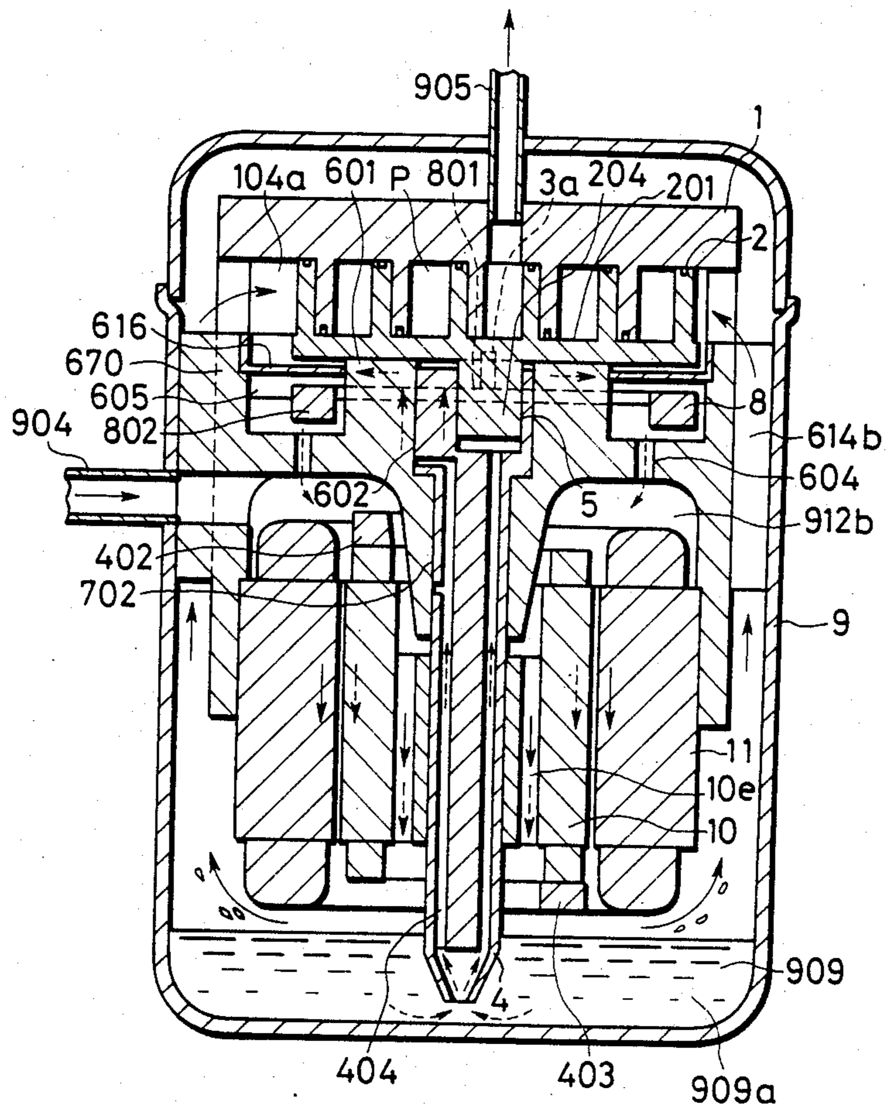
FIG. 2 PRIOR ART
