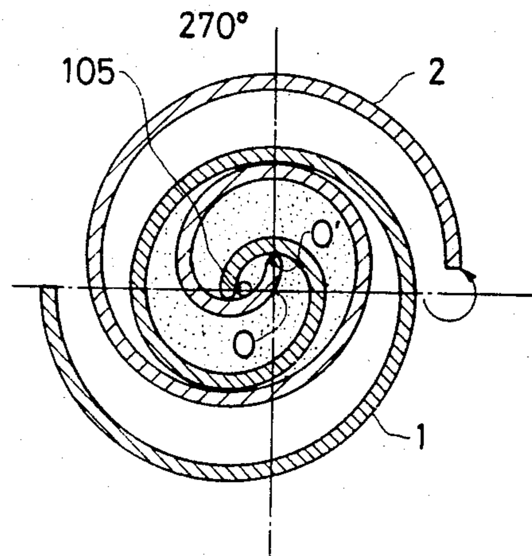
FIG. 1C PRIOR ART
