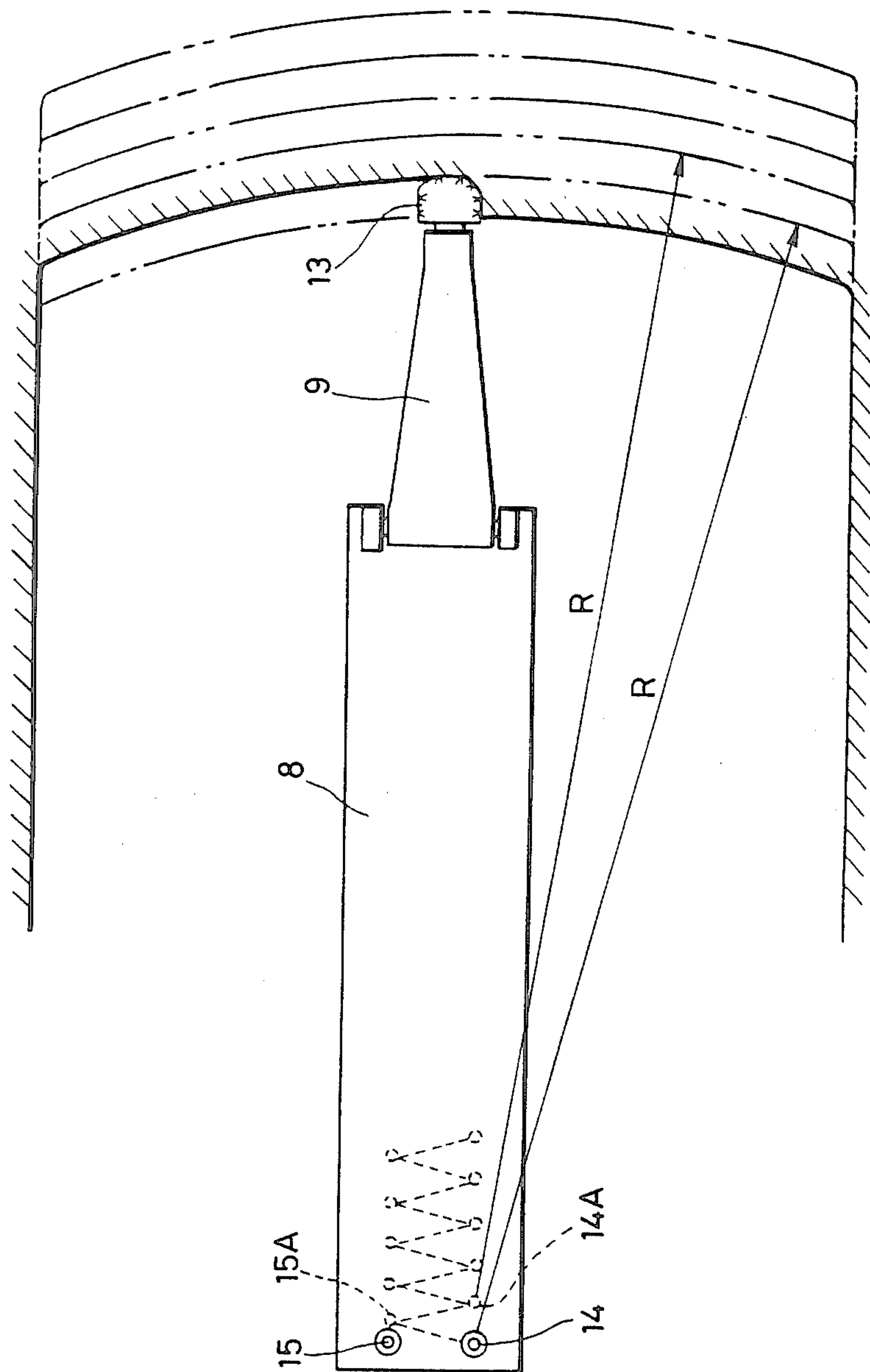
FIG. 4 PRIOR ART
