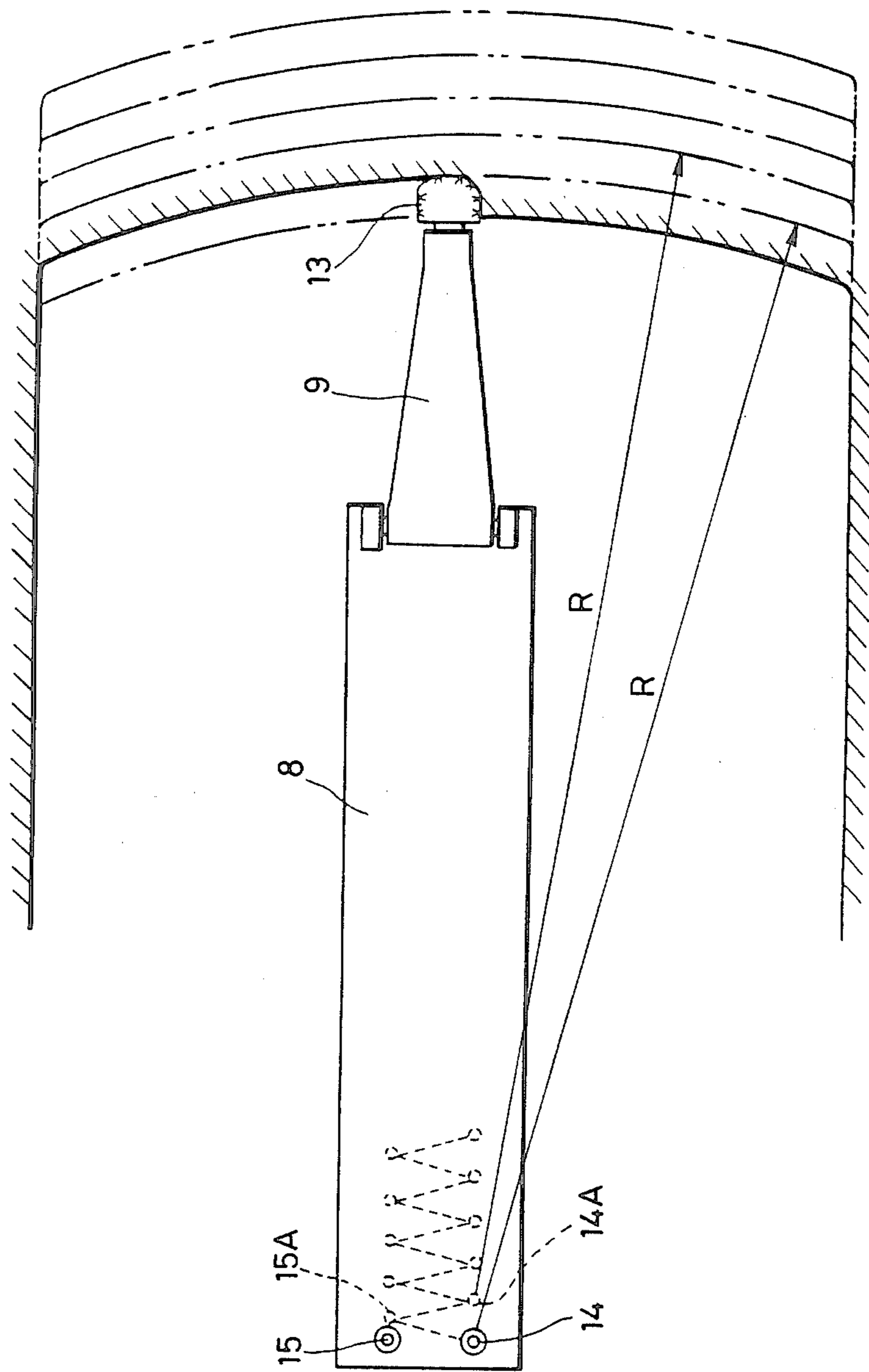
FIG. 4 PRIOR ART
